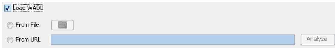
Figure 2: Loading WADL
