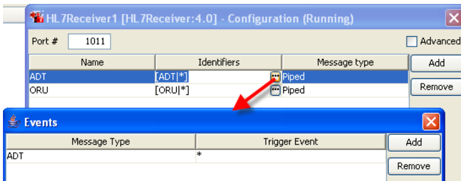
Figure 4.78: Configuring Identifiers
