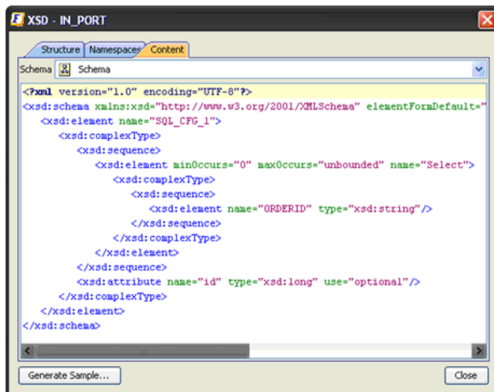
Figure 4.196: Input schema
