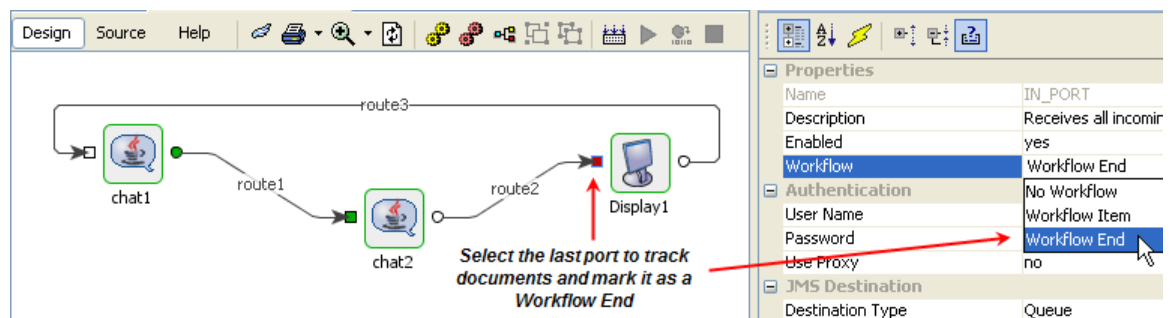
Figure 5.7.2: Workflow End
