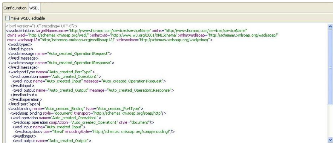
Figure 4.513: WSDL view
