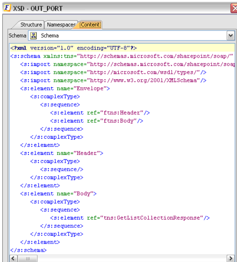
Figure 4.552: Output Schema
