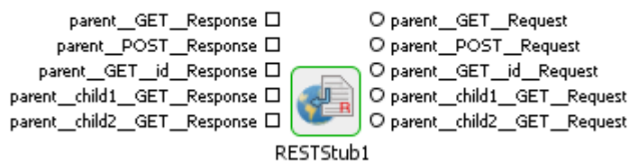
Figure 25: Port Generation
