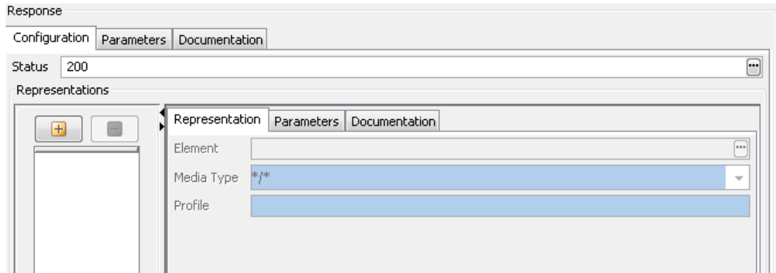
Figure 10: Response configuration
