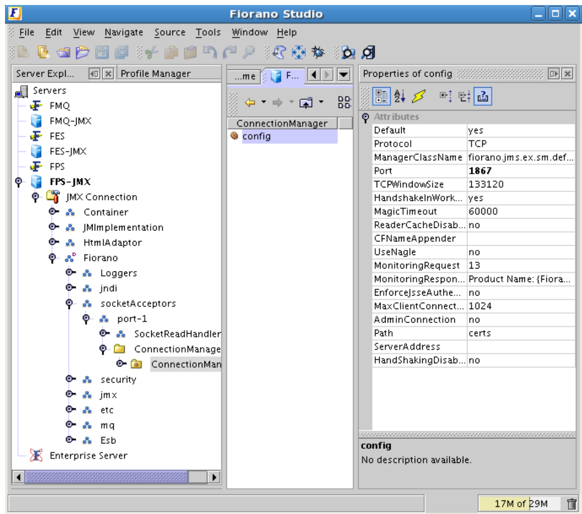
Figure 2.4.6: JMX Explorer
