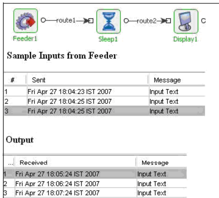
Figure 4.291: Scenario demonstration with sample input and output
