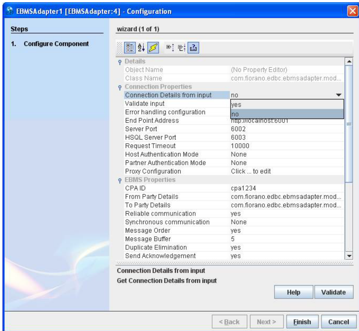
Figure 2: Configuration Property Sheet with expert properties
