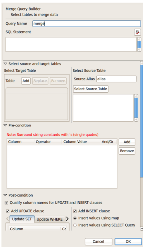
Figure: Merge Query Builder
