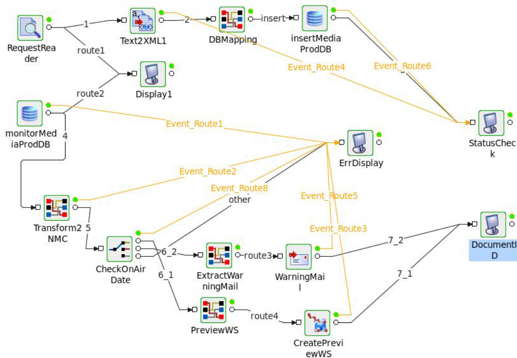
Figure 5.14.7: Retail Television Event Process Diagram
