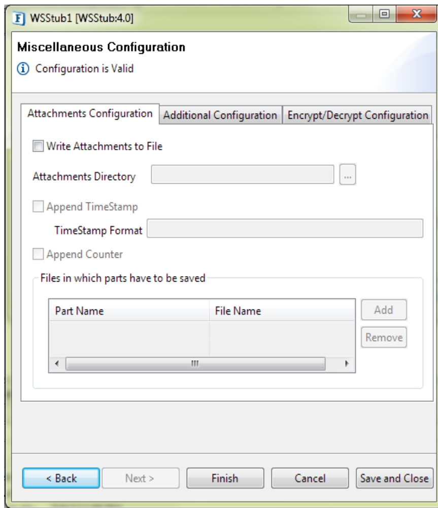
Figure: Attachments Configuration
