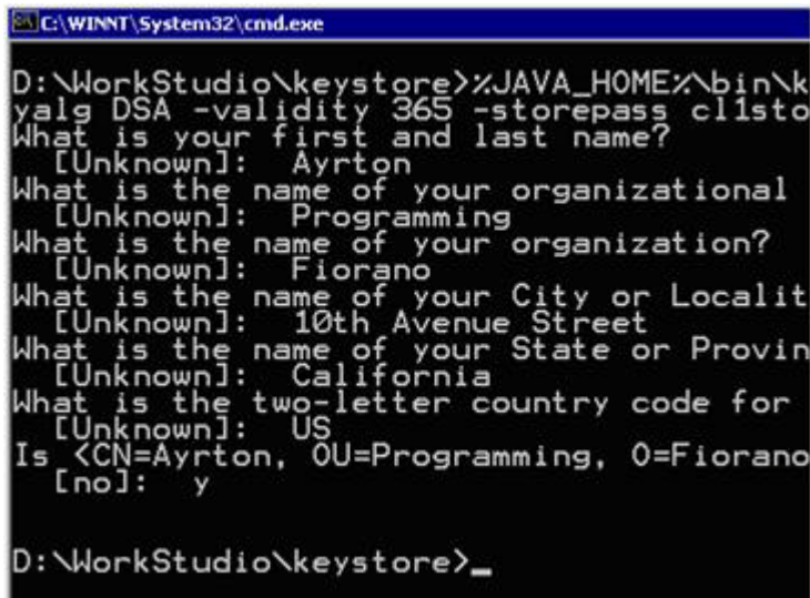
Figure I: Running the keytool command
