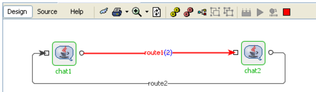
Figure 5.5.8: Route Color
