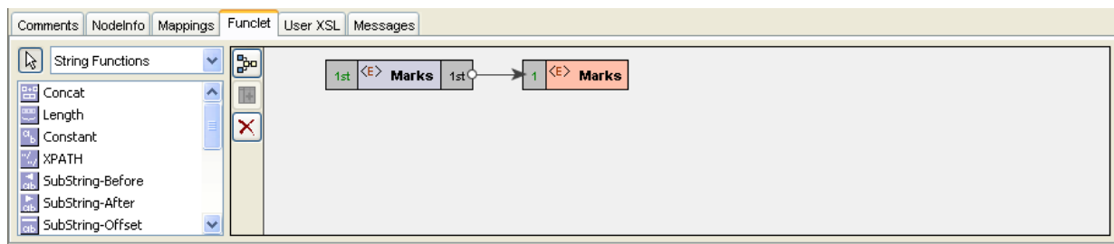
Figure 9.4.24: Funclet easel
