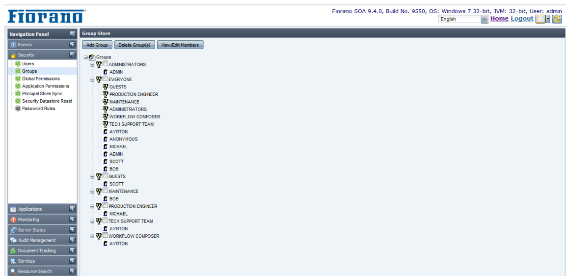
Figure 8.1.1: Users List
