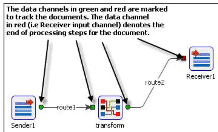
Figure 1.3.9: Tracking Document
