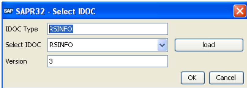
Figure 3: Select IDOC
