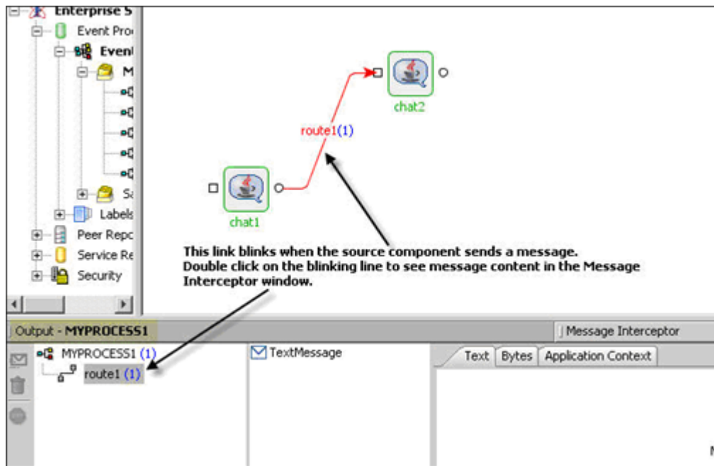
Figure 1.3.8: Intercepted Messages
