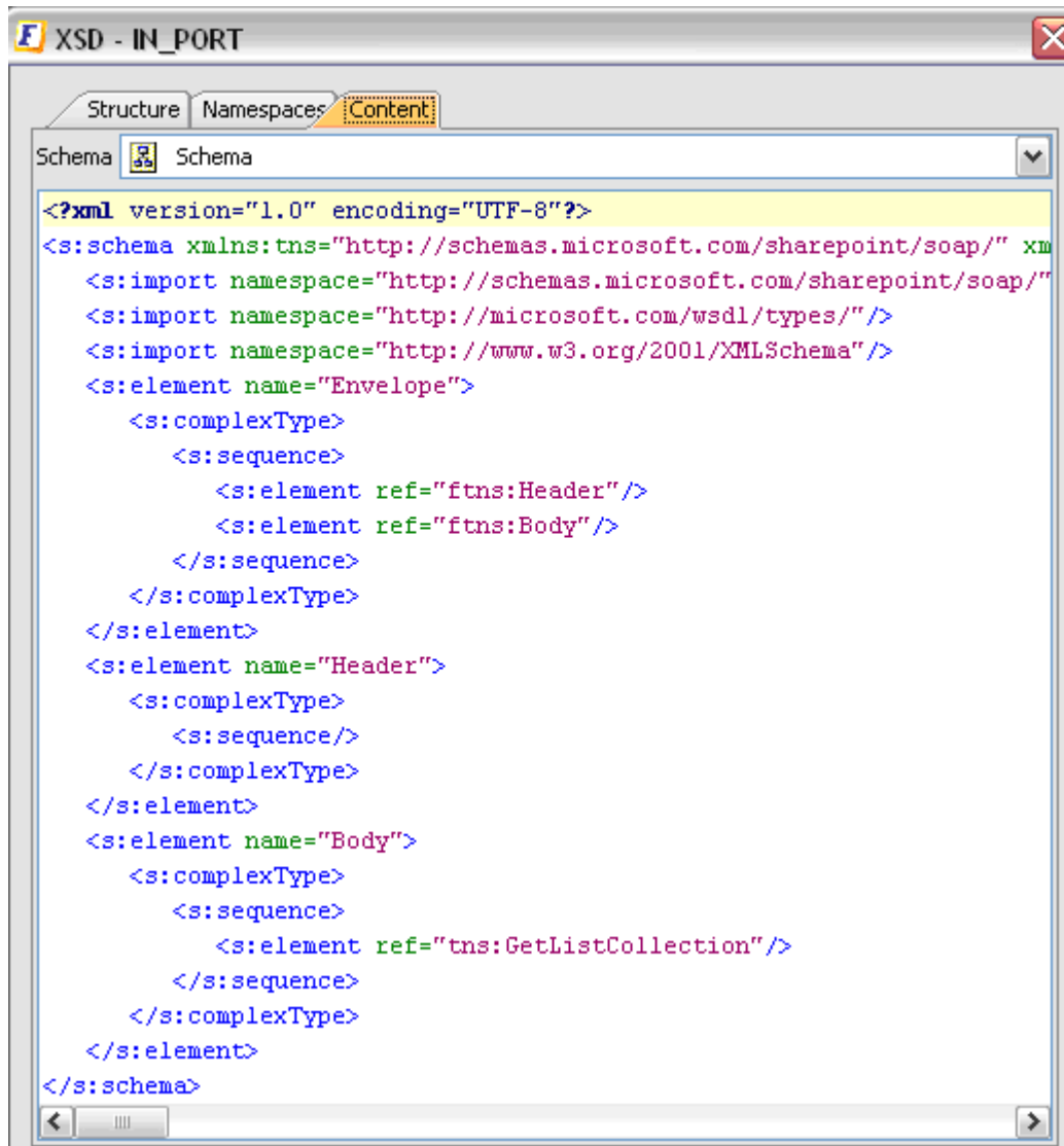
Figure 4.551: Input Schema
