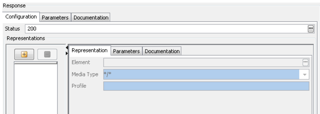
Figure 10: Response configuration
