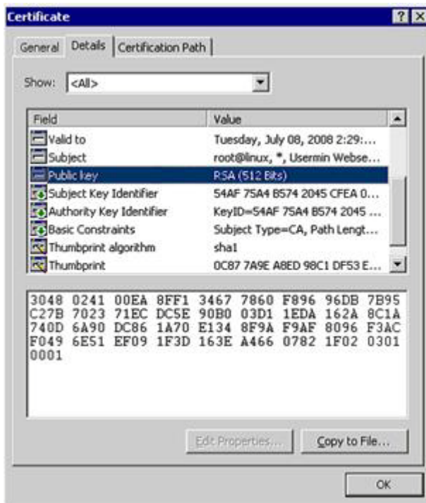
Figure IV:Public Key
