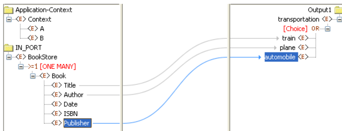
Figure 10: Sample transformation
