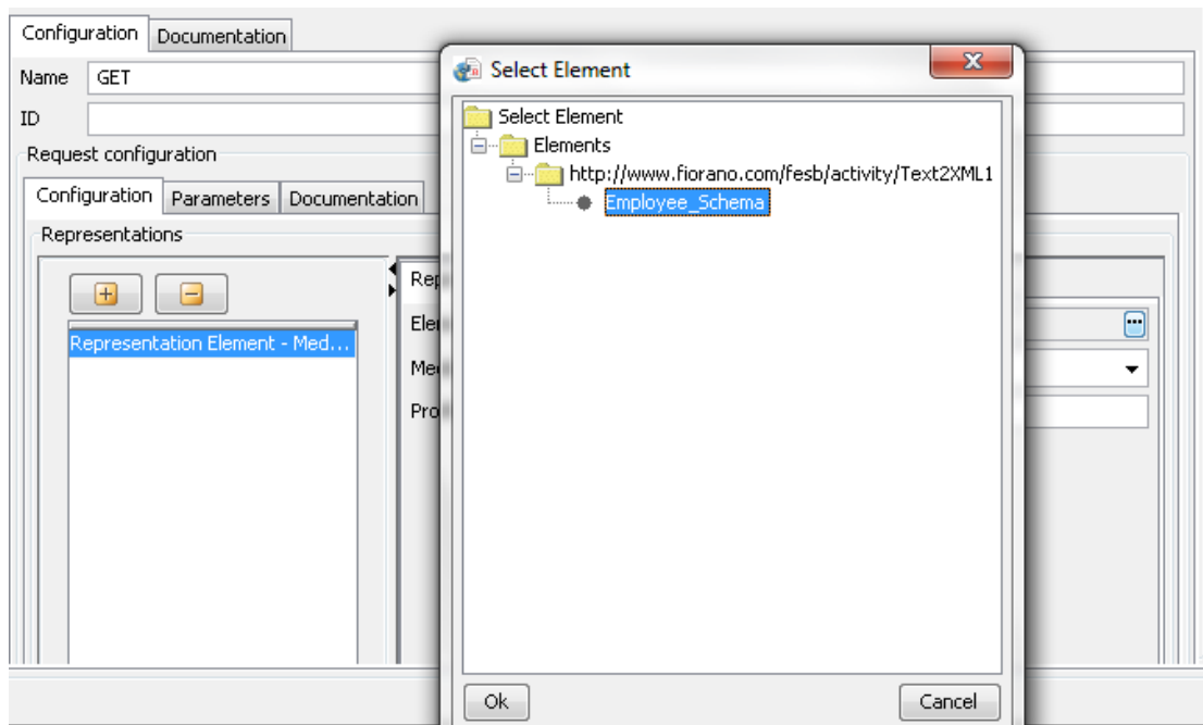
Figure 13: Configuring elements
