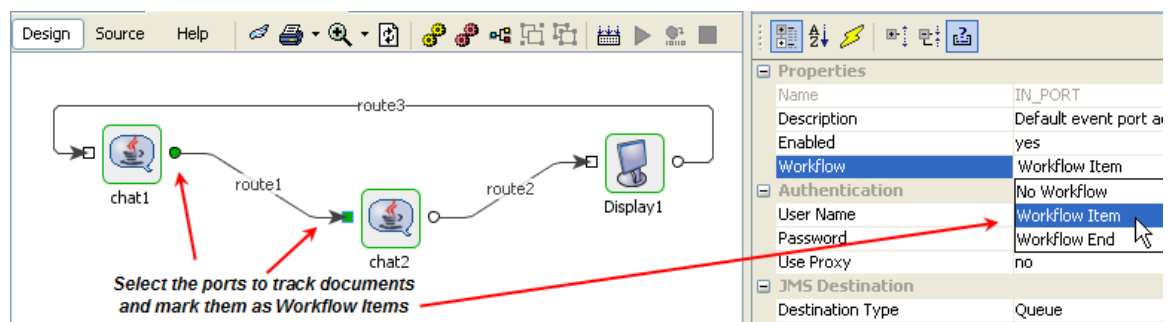
Figure 5.7.1: Workflow Items
