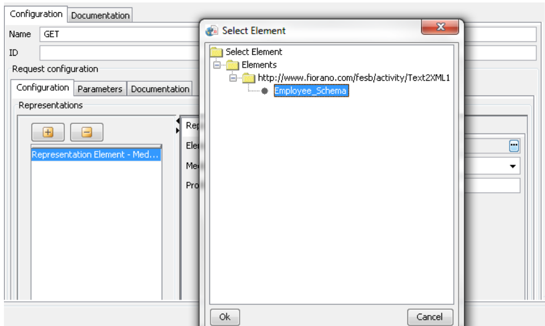
Figure 13: Configuring elements
