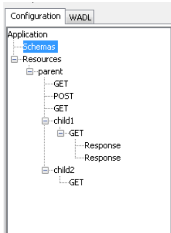
Figure 24: Sample Configuration
