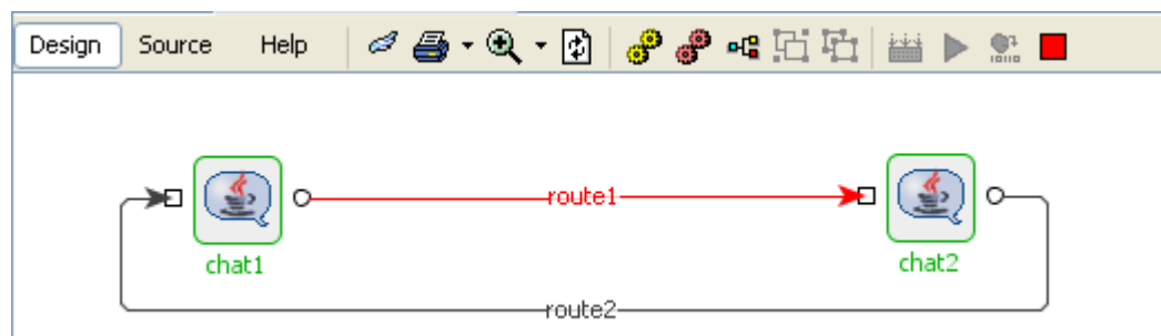
Figure 5.5.7: Route Color
