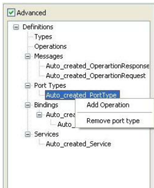
Figure 4.499: Adding Operation
