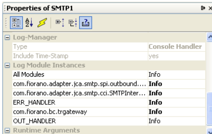
Figure 3.3.30: Log settings
