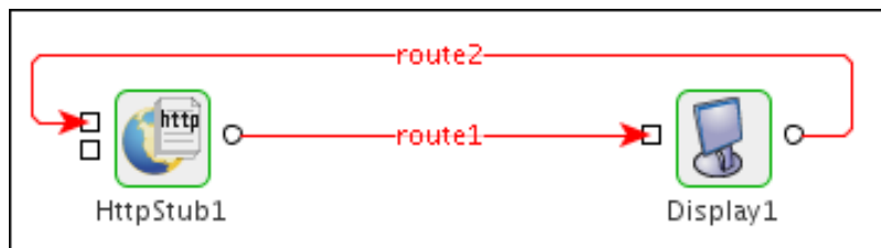
Figure 14: Demonstrating Scenario 1
