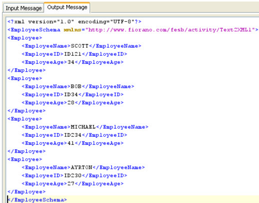
Figure 7: Sample Output
