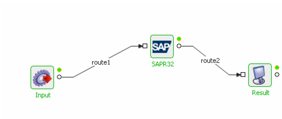
Figure 8: Sample Flow
