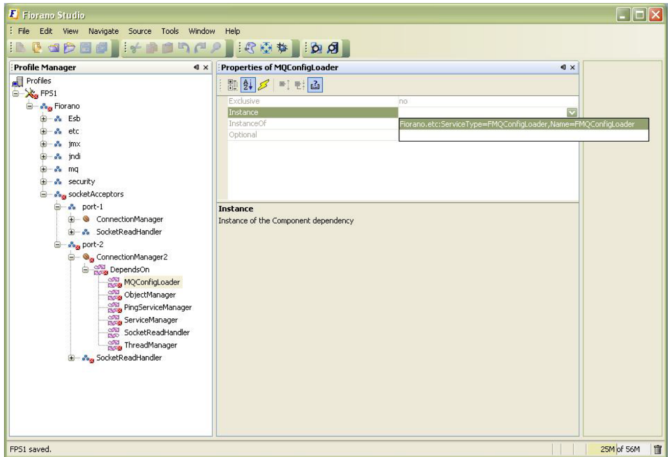
Figure 2.6.17: Adding Components
