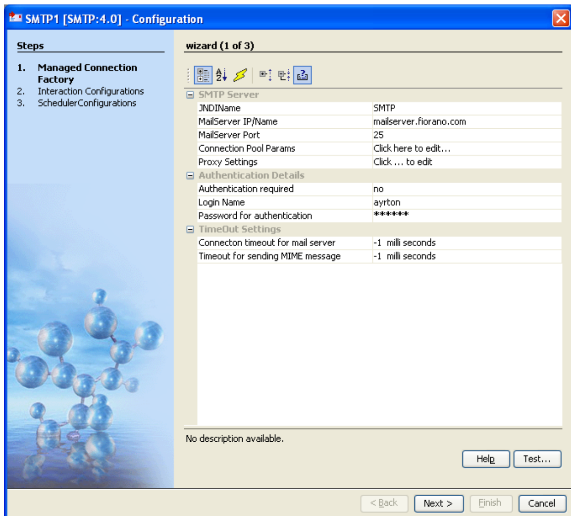
Figure 3.3.3: A typical CPS (SMTP component)
