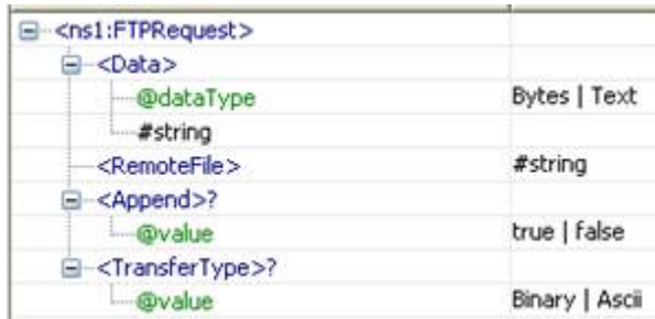
Figure 23: Input schema structure for the request type - Data
