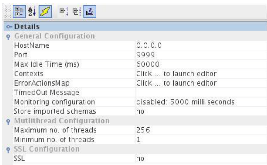
Figure 1: Configuration of HTTPReceive
