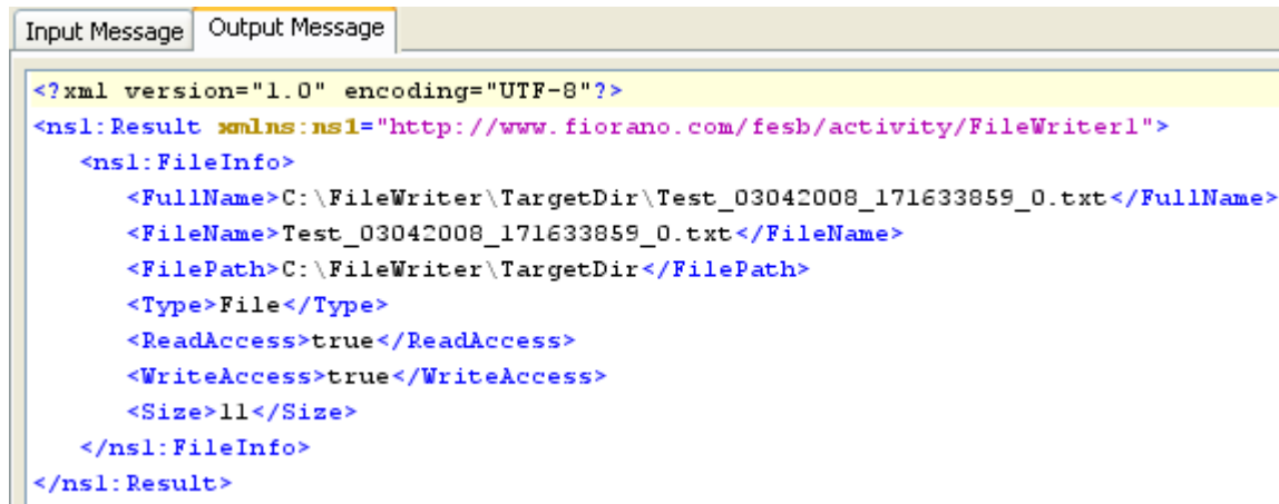
Figure 11: Output generated for input shown in Figure 10.
