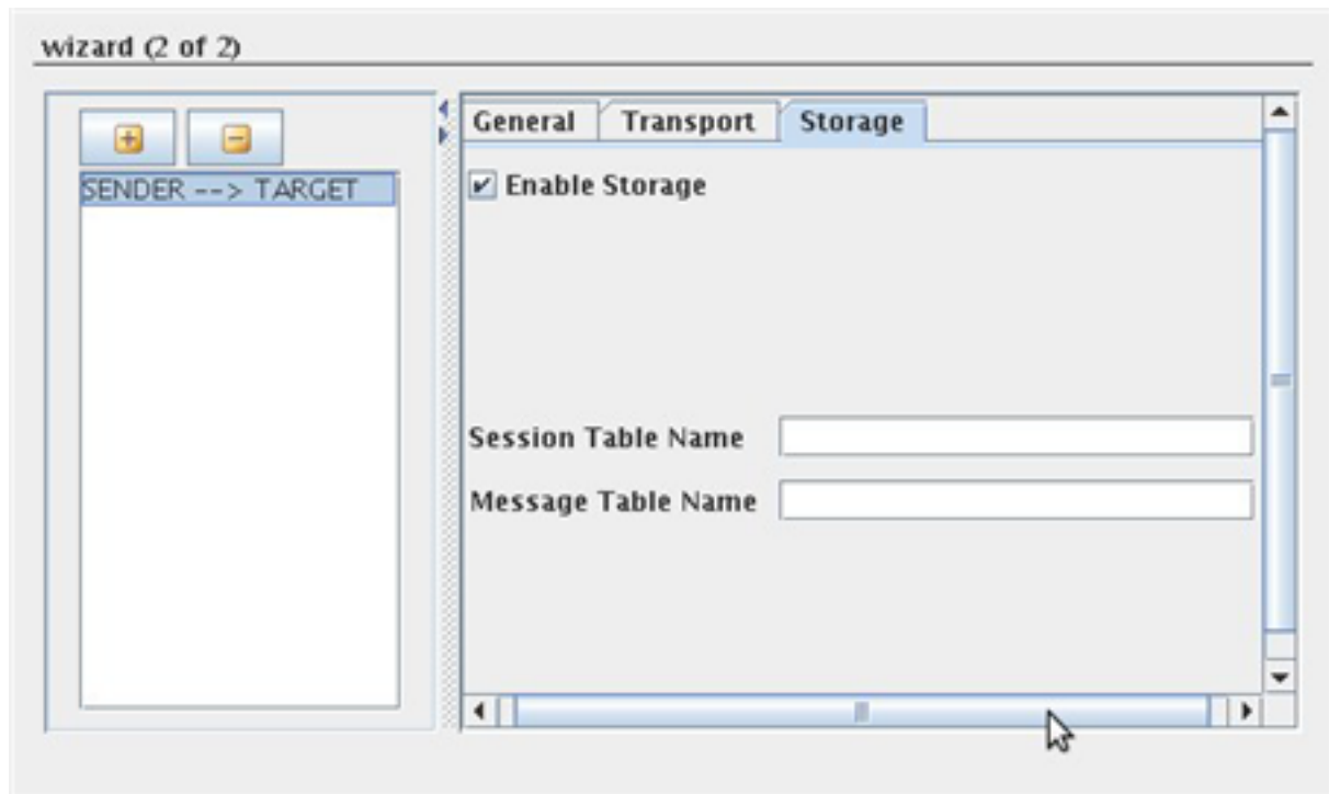
Figure 7: Database Store Configuration
