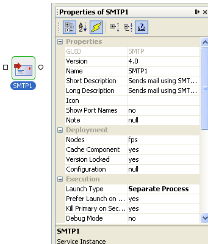
Figure 1: Component instance properties for a SMTP component
