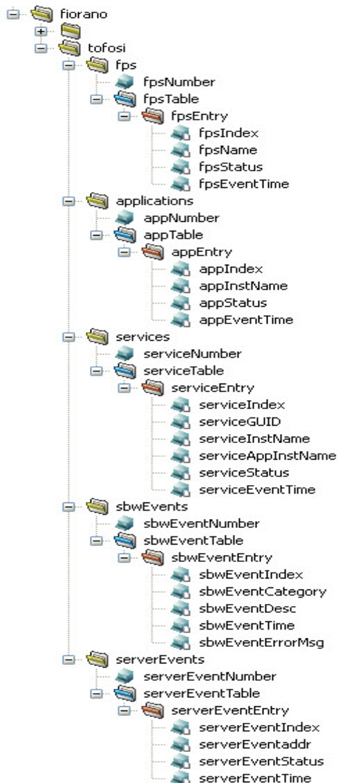
Figure 2.6.22: Fiorano SOA Platform MIB tree
