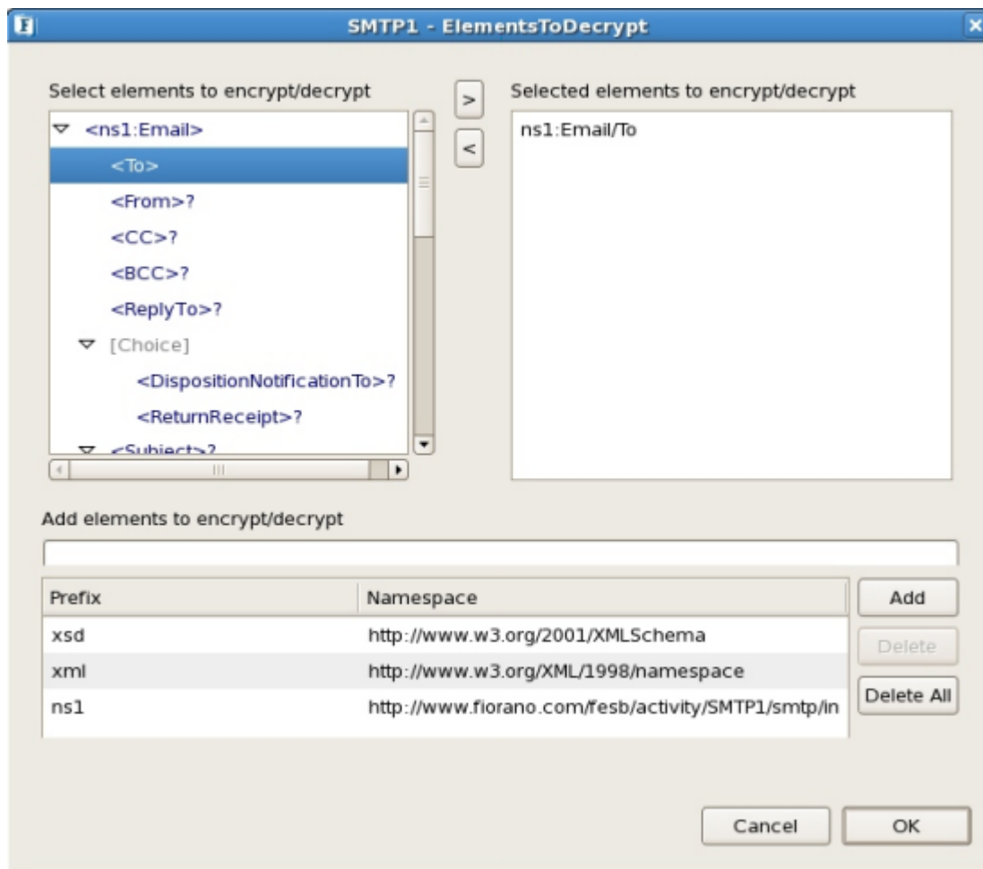
Figure 45: Encrypt/Decrypt Configuration page in SMTP
