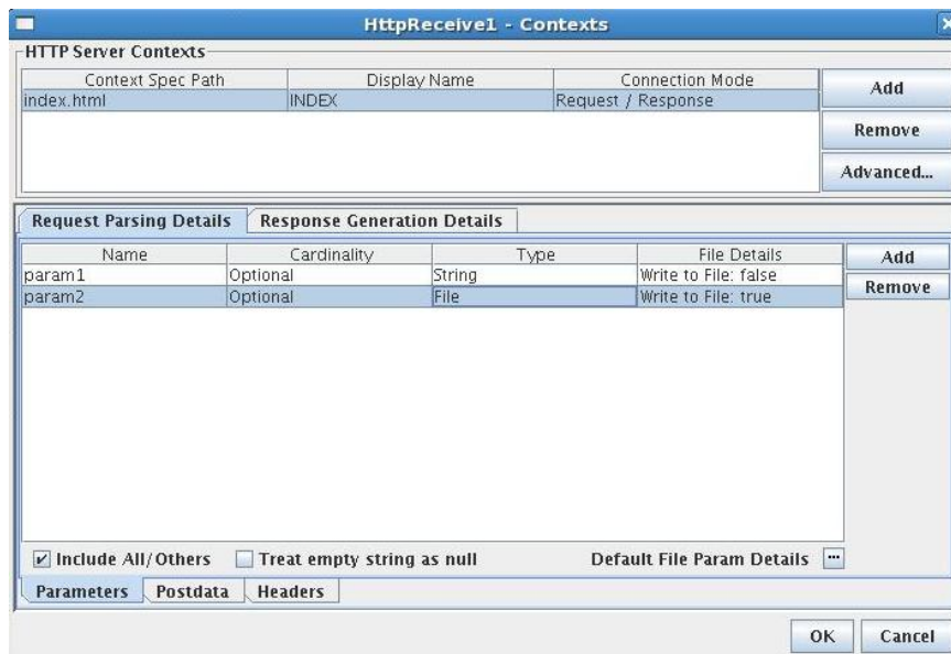
Figure 3: Configuration of Request Parsing Details
