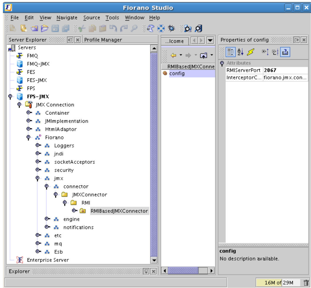
Figure 2.4.10: JMX Explorer
