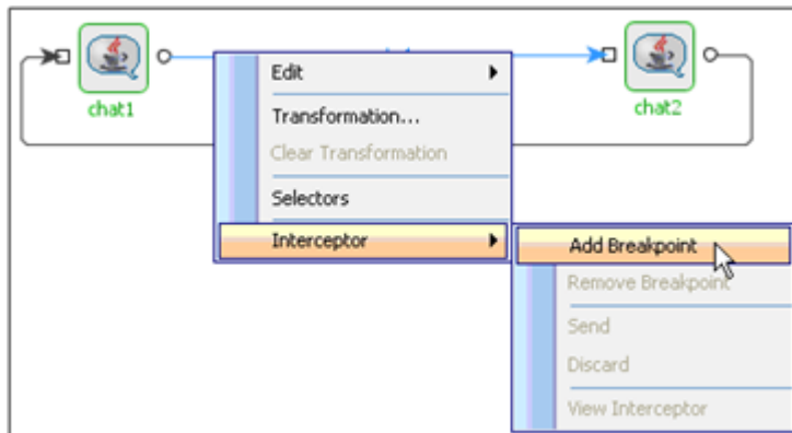
Figure 5.5.6: Add Breakpoint
