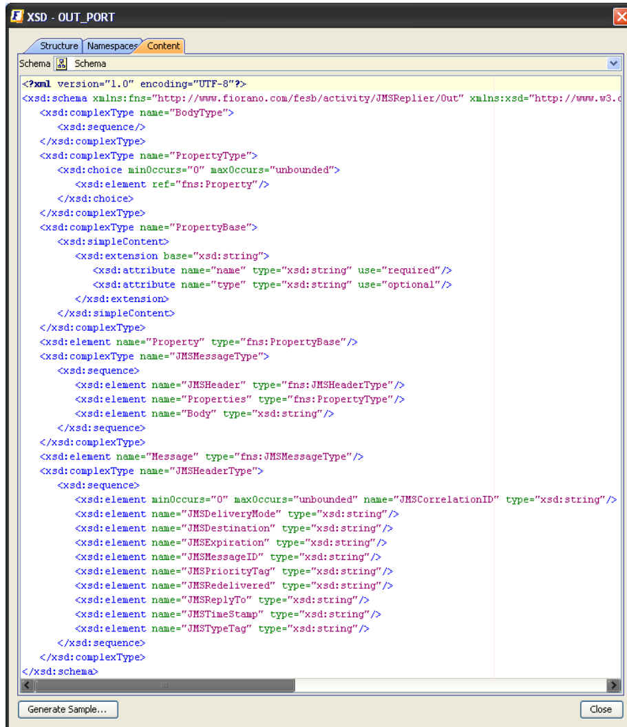
Figure 4.329: Output Schema
