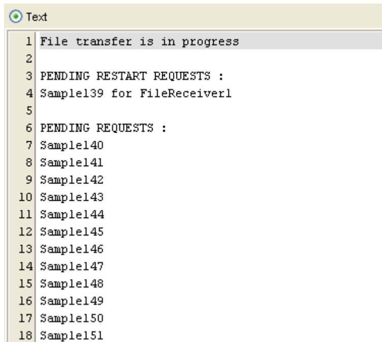
Figure 4.269: Sample output
