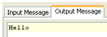
Figure 4.16: Sample output
