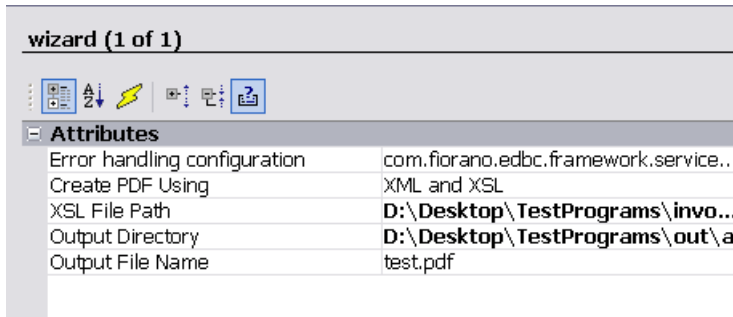
Figure 1: Component configuration
