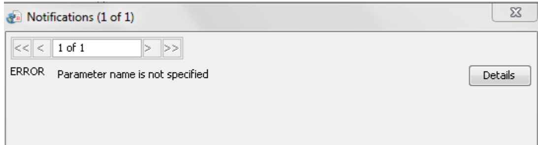
Figure 17: Error Notifications
