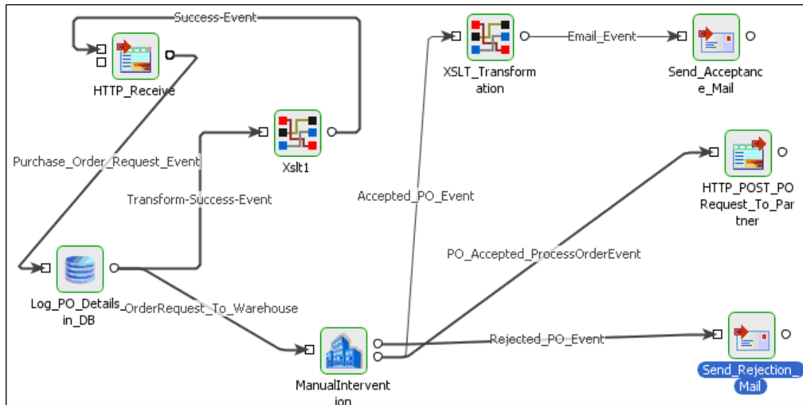
Figure 33: Order Entry
