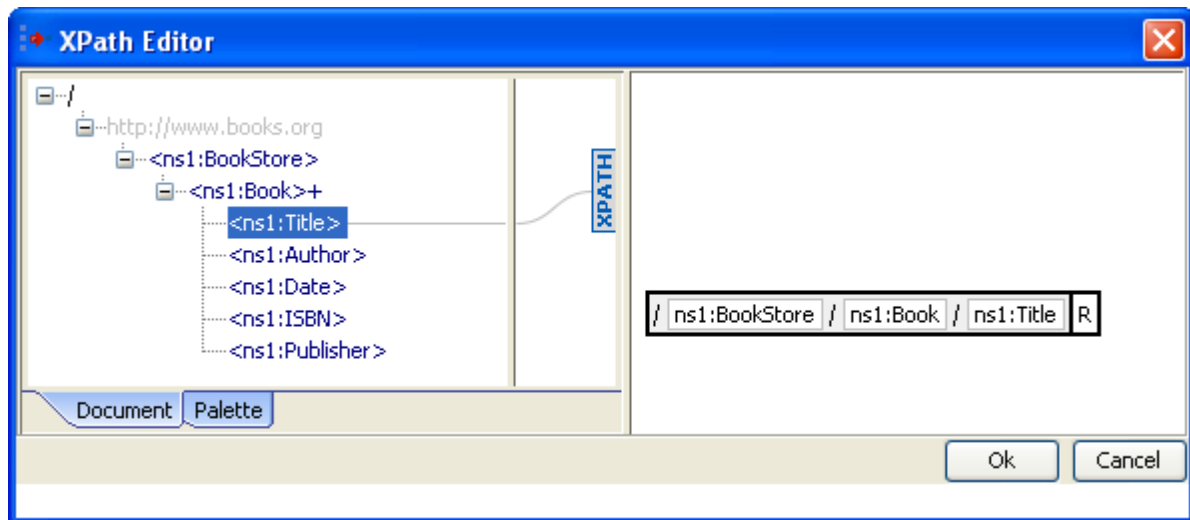
Figure 34: XPath Editor
