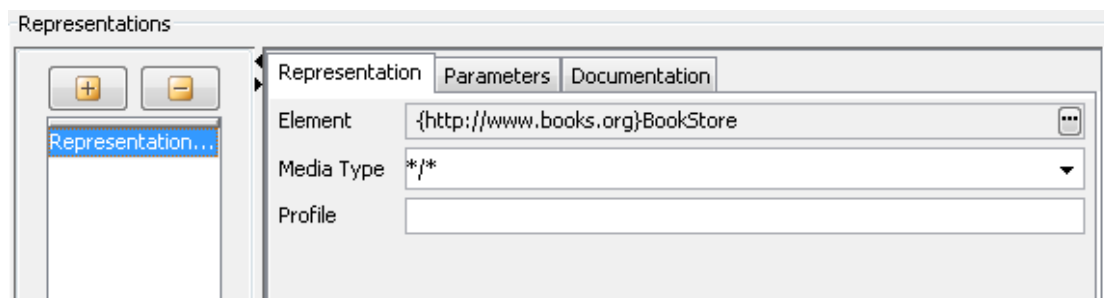
Figure 12: Representation Configuration
