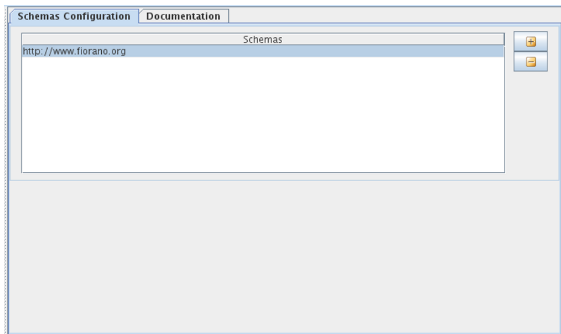
Figure 5: Schemas Configuration
