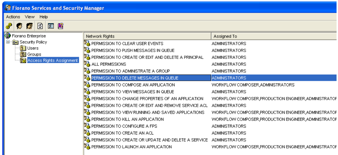
Figure 2.3.23: Realms Description
