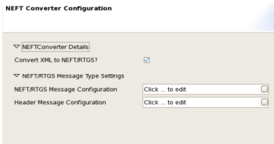
Figure 1: NEFTConverter CPS
