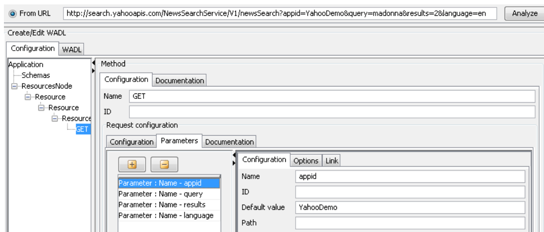
Figure 4: Analyzing URL
