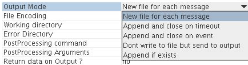
Figure 5: Output Mode
