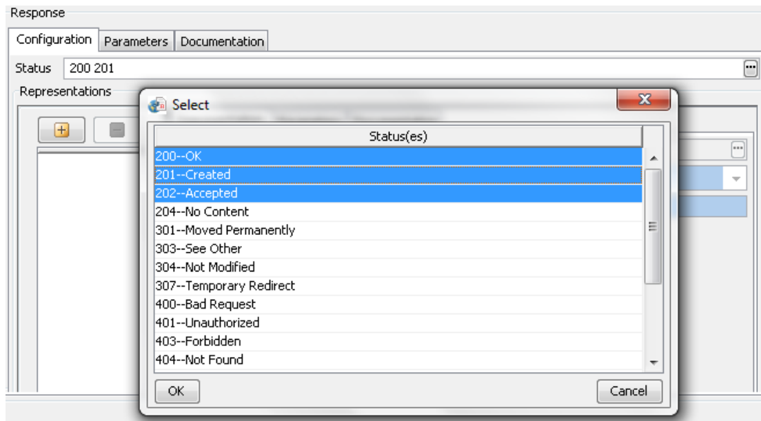
Figure 11: Configuring status
