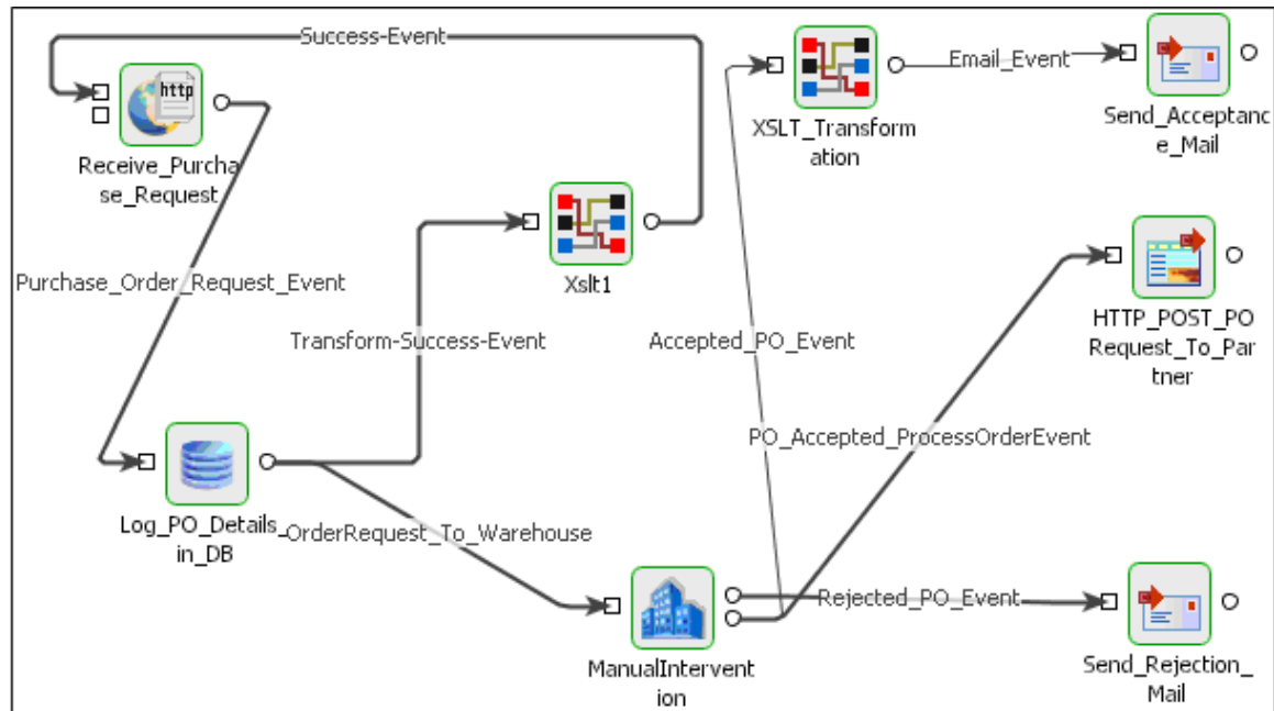
Figure 16: Order Entry
