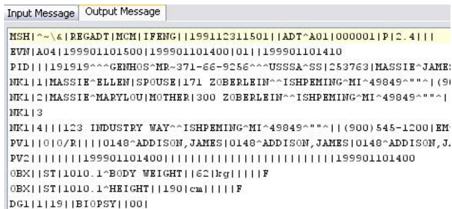
Figure 4.406: Response Generated
