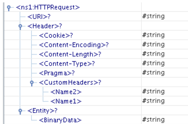
Figure 18: Schema when parameters/postdata set to 'BinaryData'
