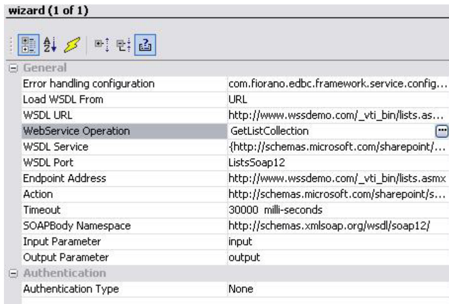
Figure 4.547: CPS after selecting WSDL operation
