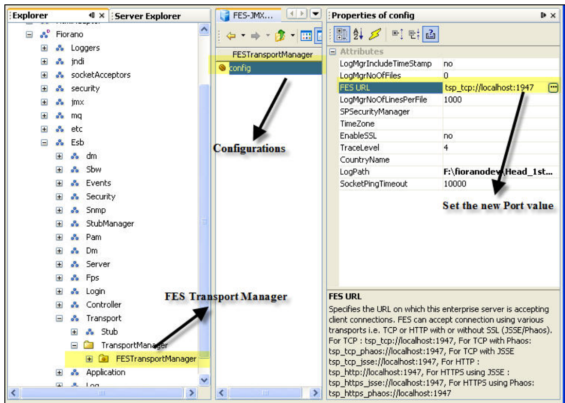
Figure 2.3.7: JMX Explorer
