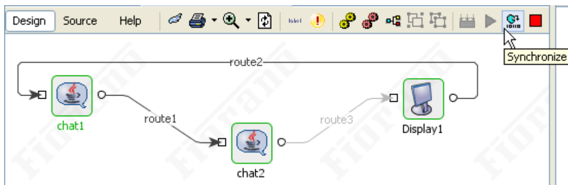
Figure 5.6.4: Synchronize Routes
