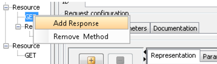
Figure 9: Adding Response
