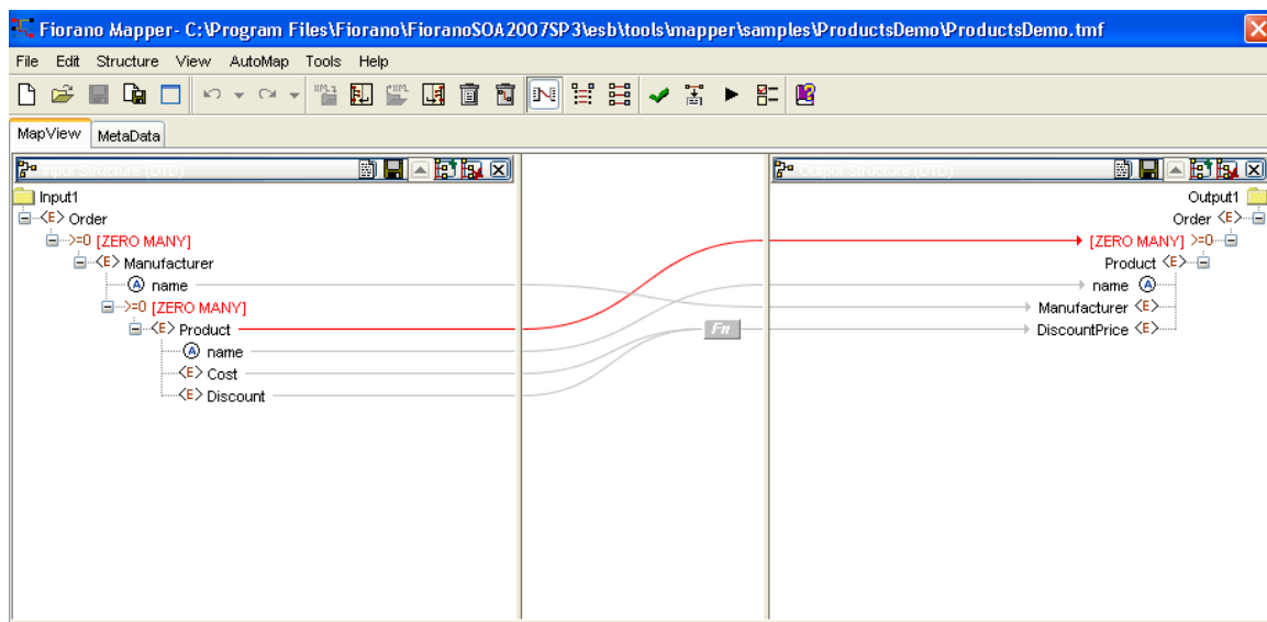
Figure 9.5.6: Name-to-name Mapping
