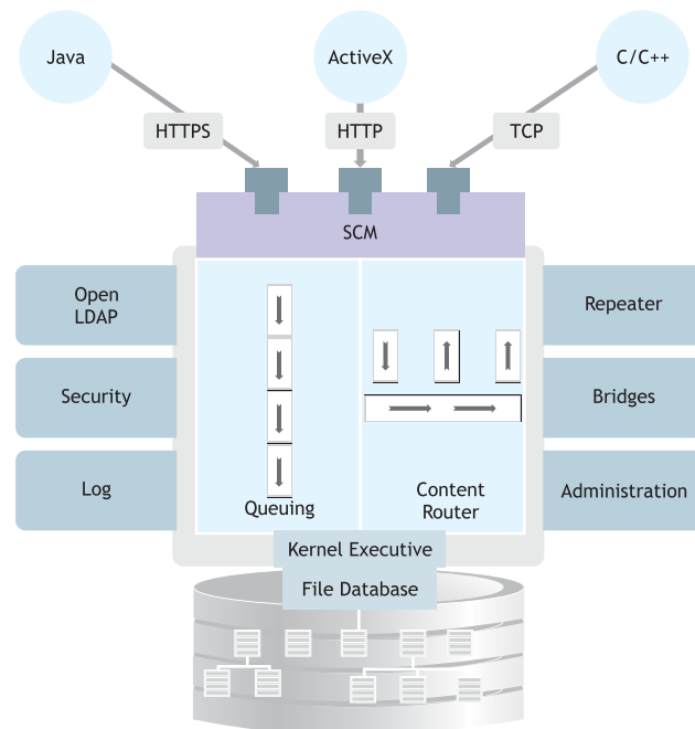
FioranoMQ Architecture
