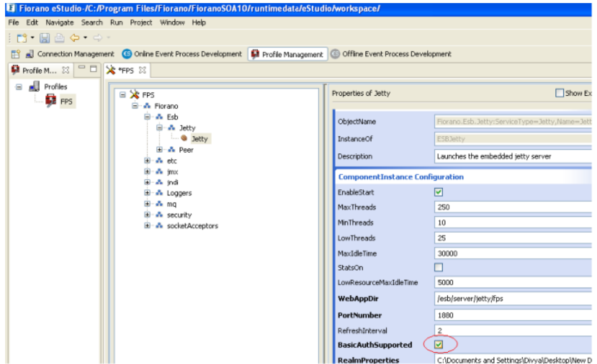
Figure 2.6.11: Enabling Basic Authentication
