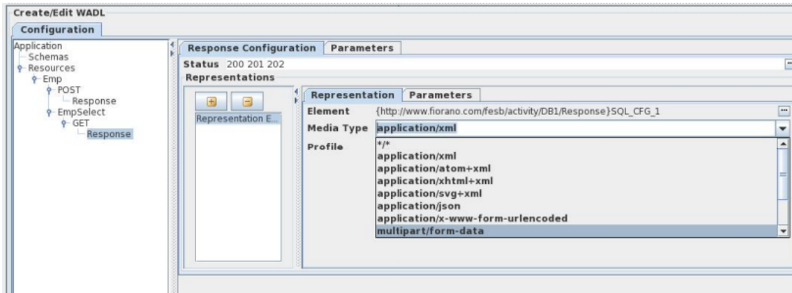
Figure 14: Media Type configuration
