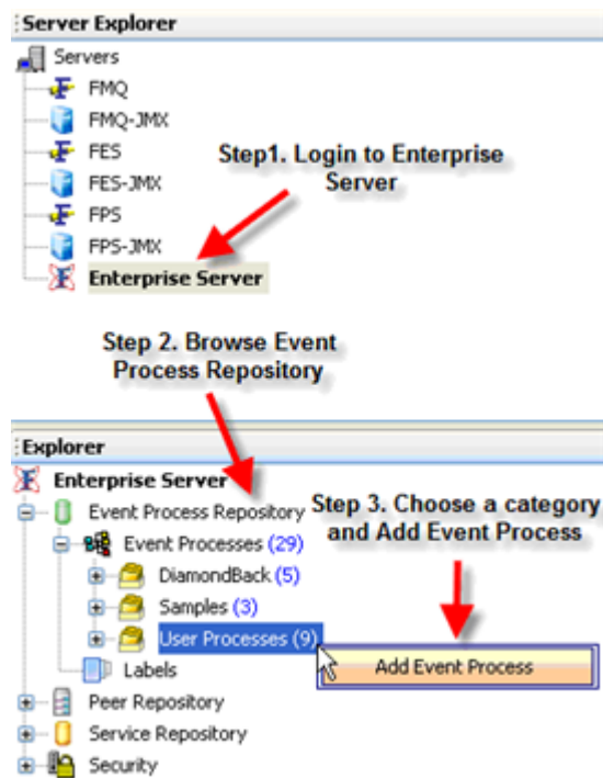
Figure 5.2.3: Create an Event Process
