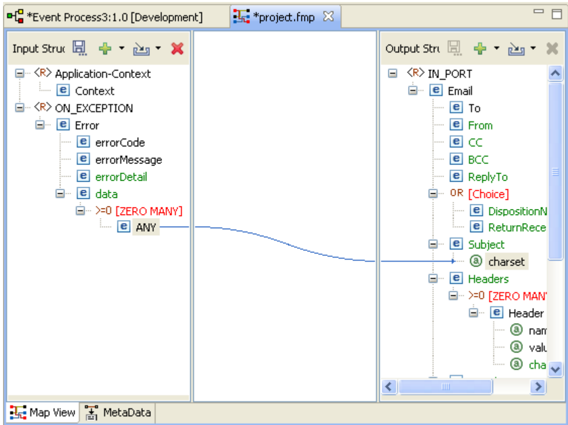
Figure 1.3.5: The Fiorano eMapper Screen
