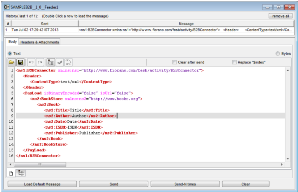
Figure 7: Sample Input Message sent to B2b Core Event Process
