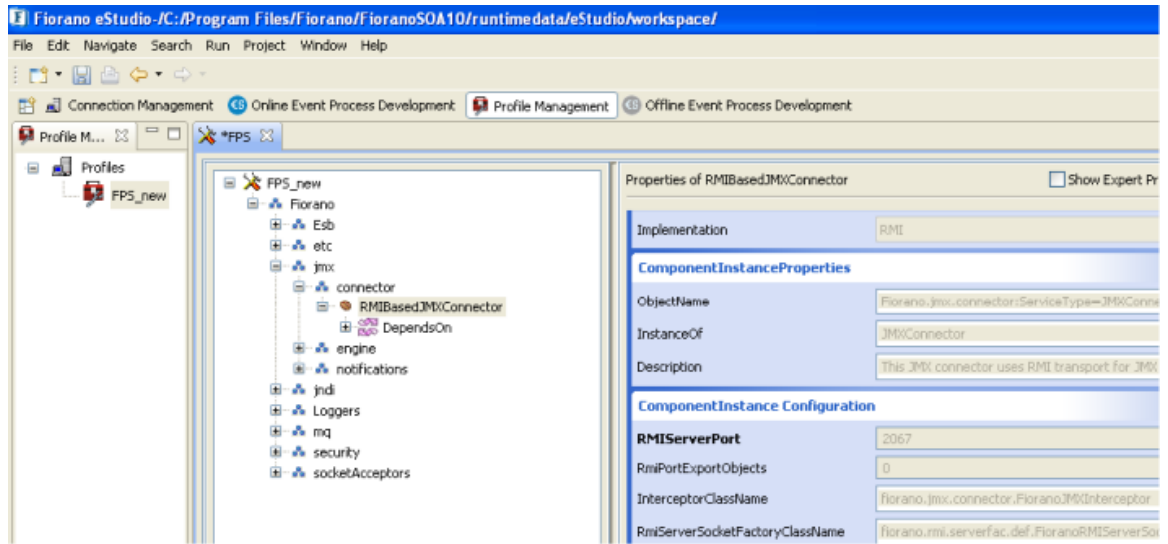
Figure 2.4.14: Changing RMI port
