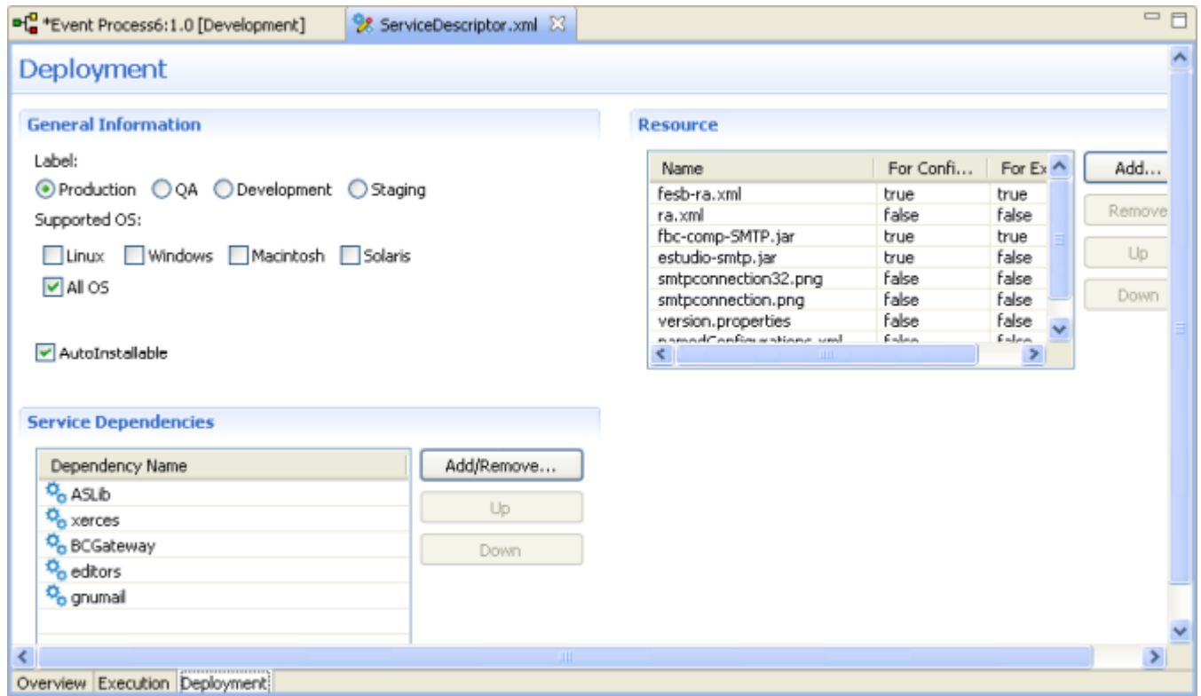
Figure 3.3.10: List of dependencies for SMTP component
