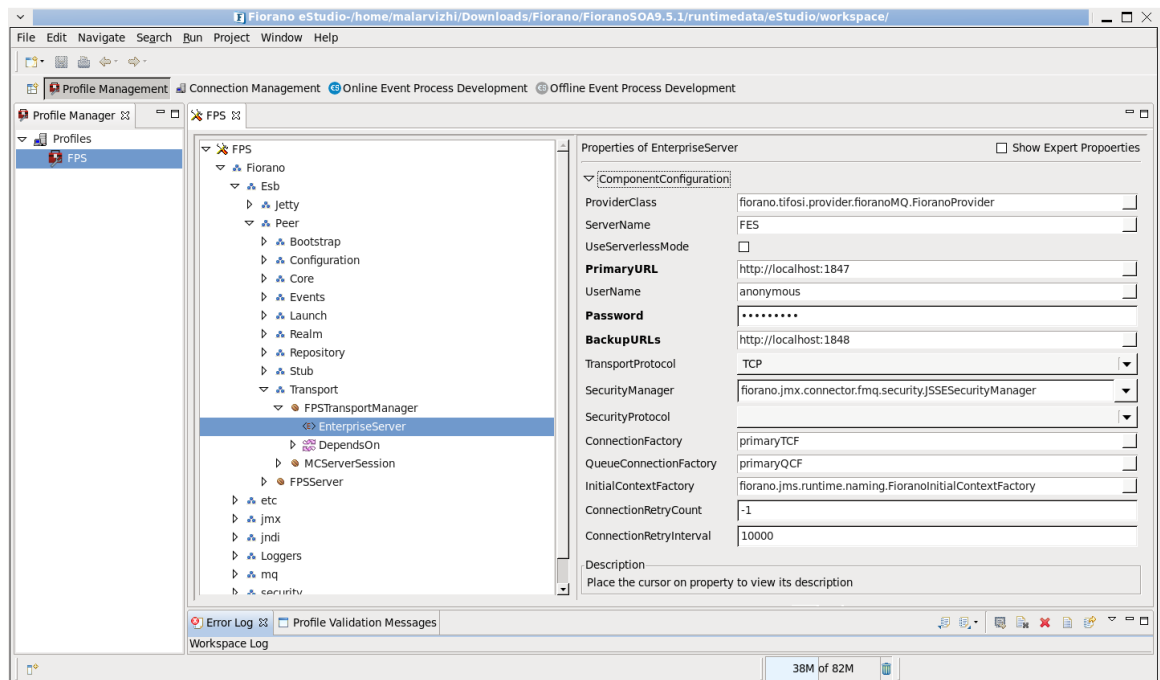
Figure 2.4.11: Configuration of Enterprise Server properties
