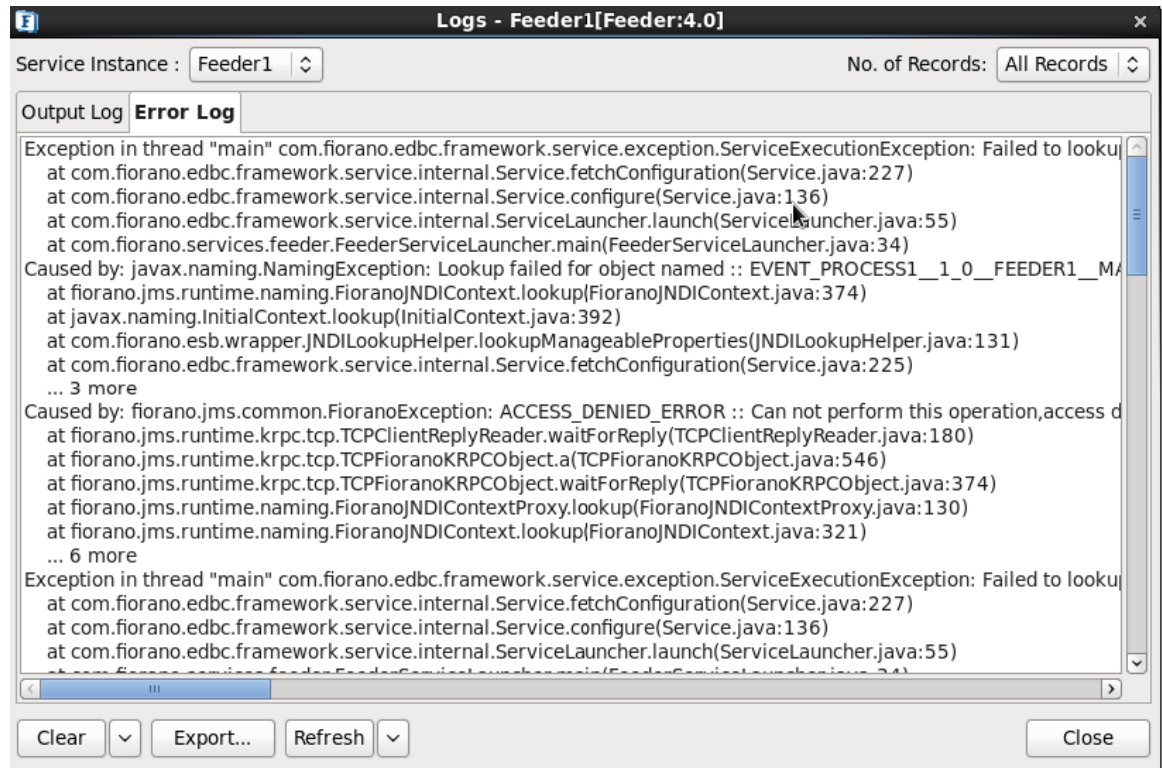
Figure 3.4.34: UI showing logs of the component
