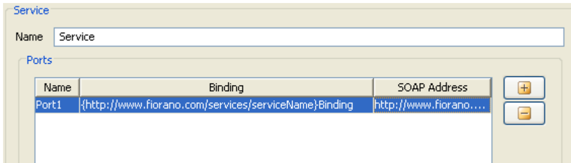
Figure 4.512: Service and ports configuration
