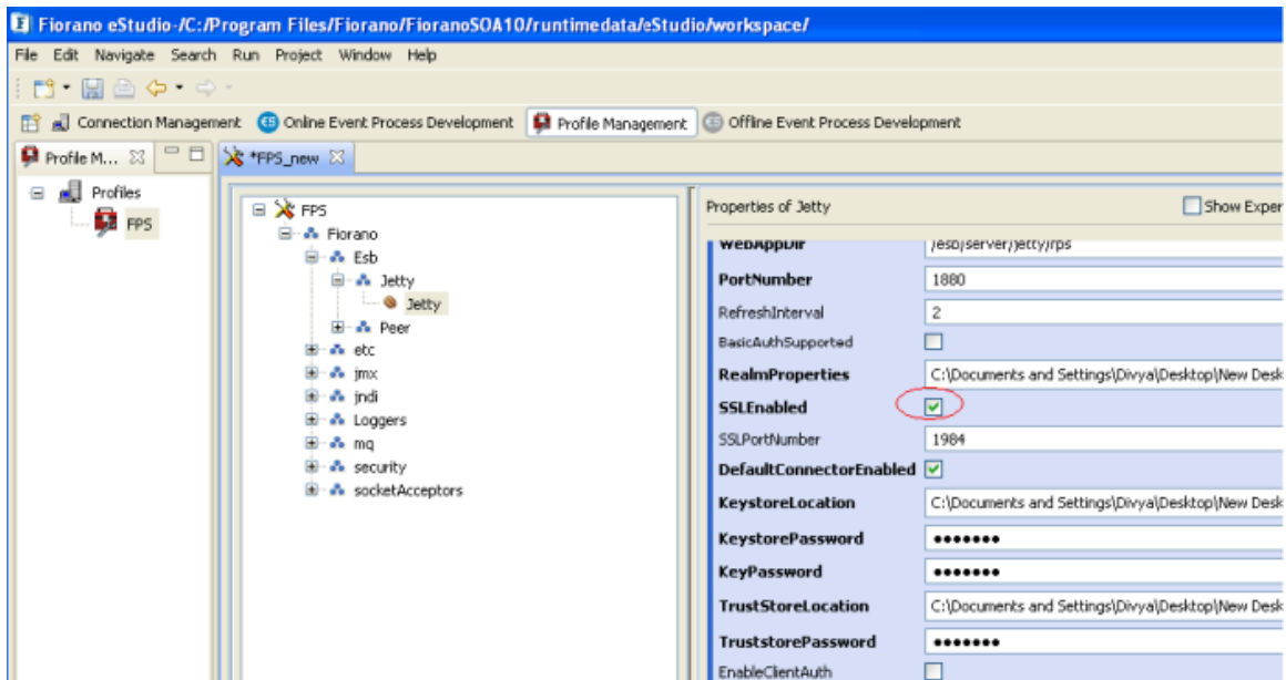
Figure 2.6.3: Configuring Jetty for FPS
