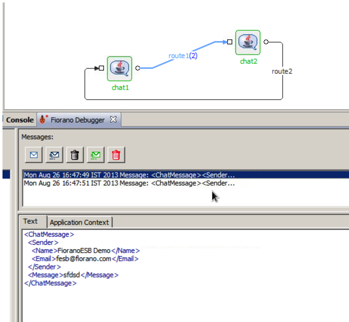
Figure 5.5.11: Message Interceptor View Screen
