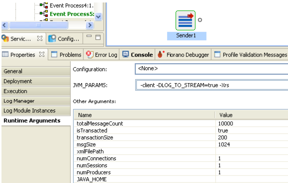
Figure 3.3.7: Fiorano eStudio showing runtime arguments in properties window
