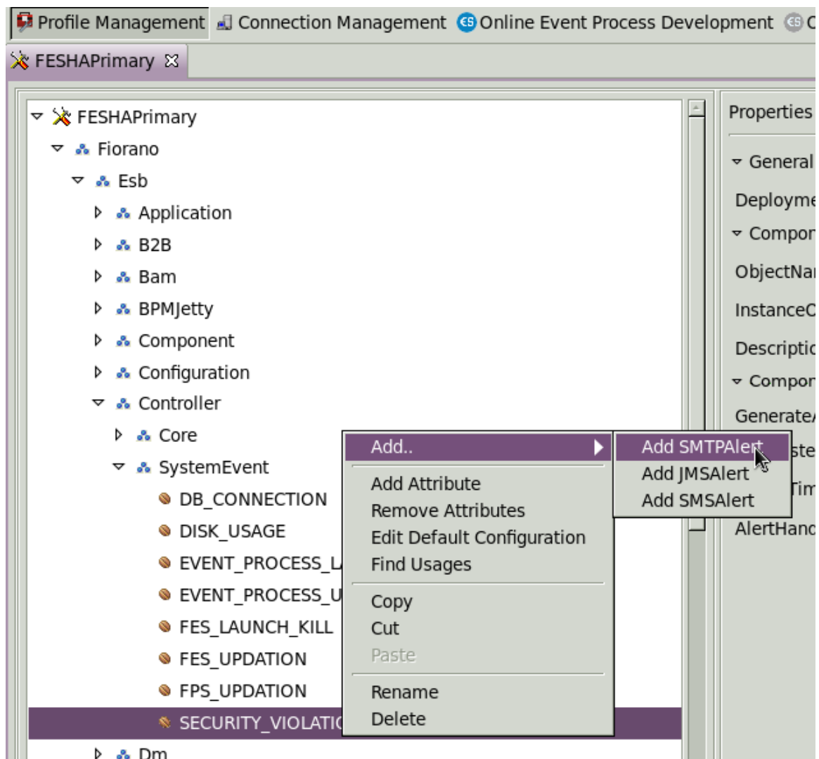
Figure 5.3.11: Adding new SMTPAlert
