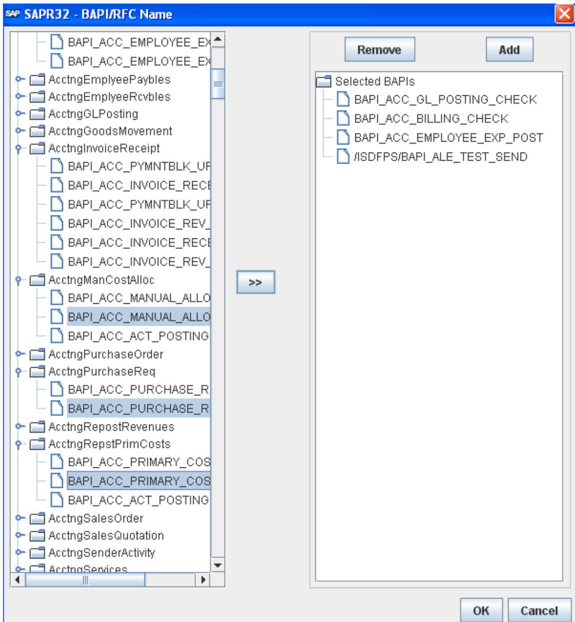
Figure 2: Dialog to select BAPI/RFC Name
