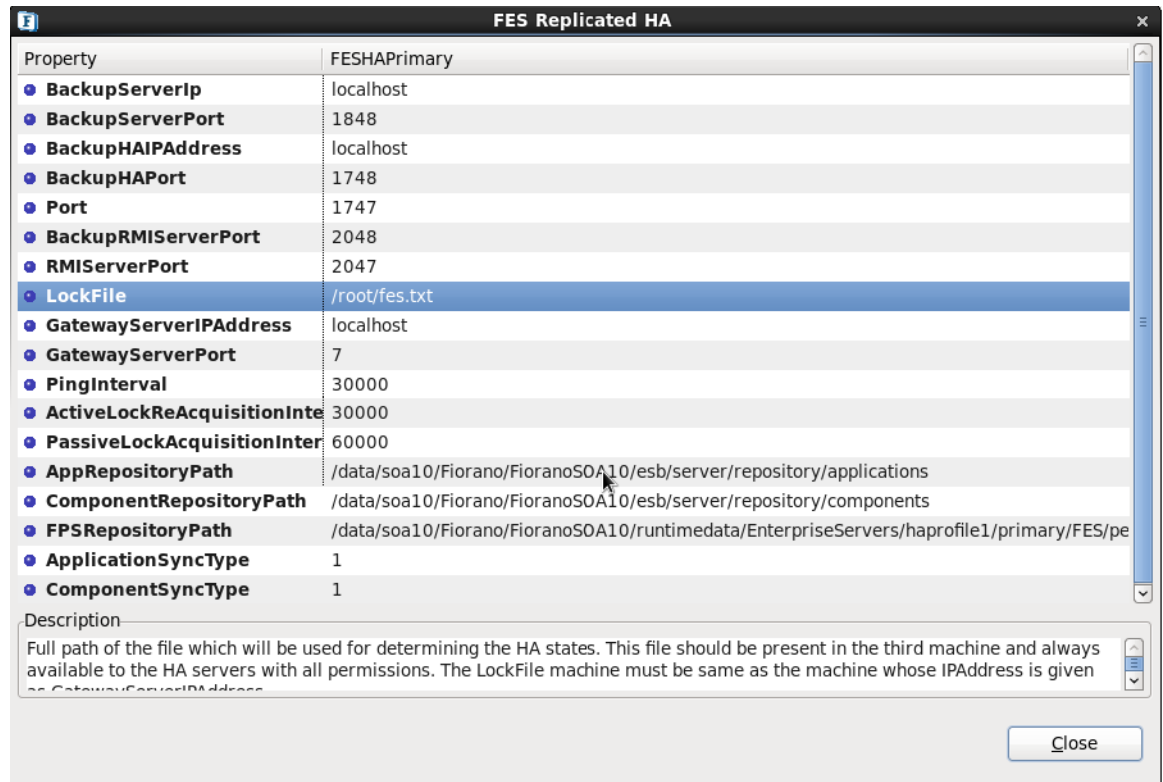
Figure 6: FES Replicated HA... dialog box
