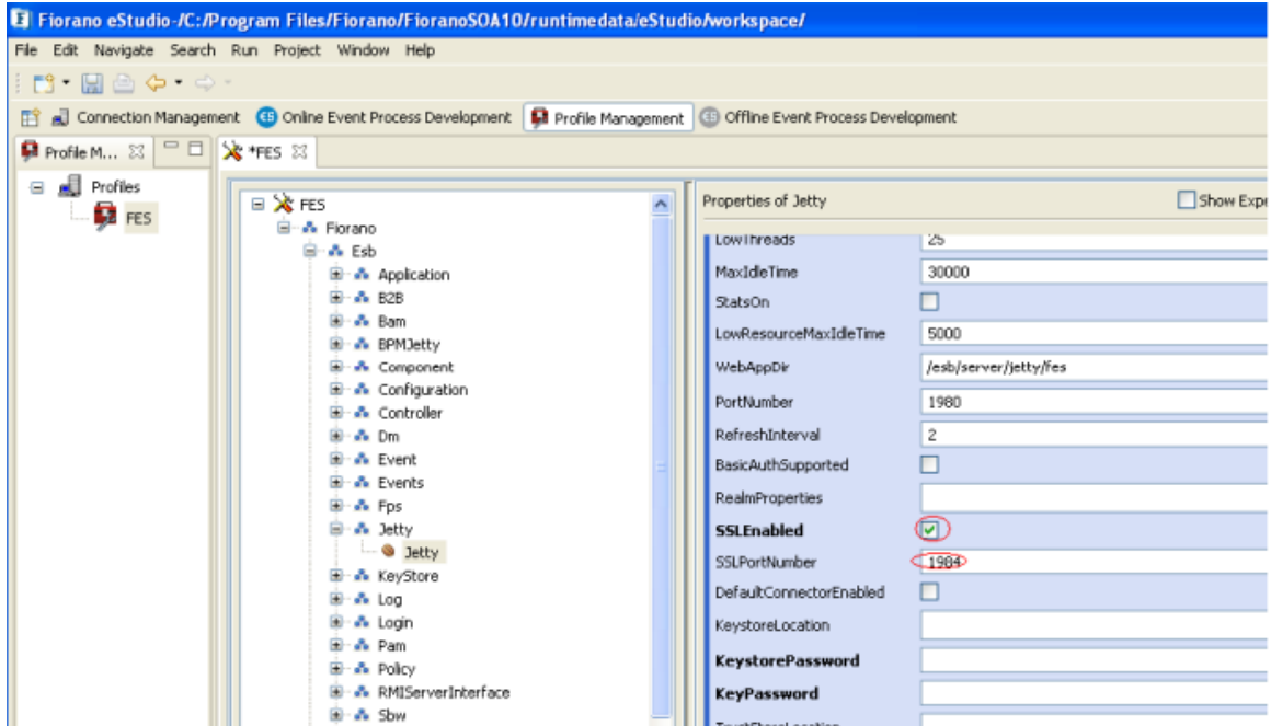
Figure 2.6.4: Configuring Jetty for FES
