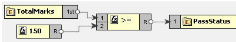
Figure 9.4.13: Linking the >= and PassStatus nodes
