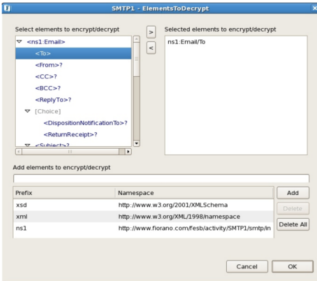
Figure 45: Encrypt/Decrypt Configuration page in SMTP
