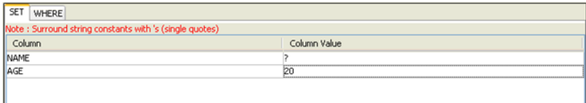
Figure 4.128: Specifying constant value for a column in SET clause
