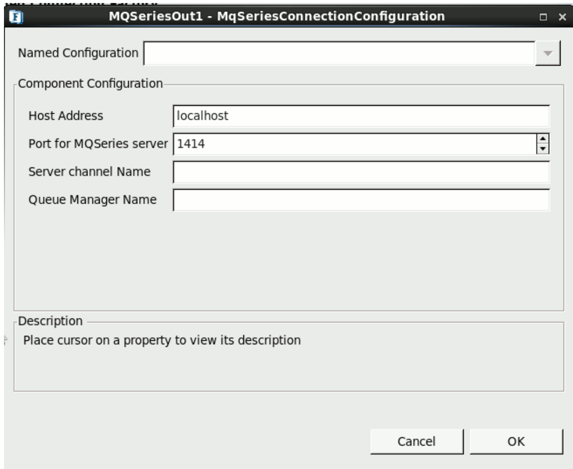
Figure 12: Connection configuration details in MCF panel
