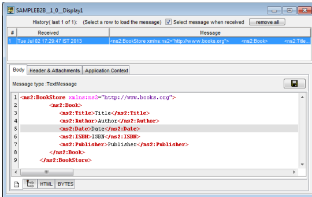
Figure 9: Message received from the Core B2B Event Process
