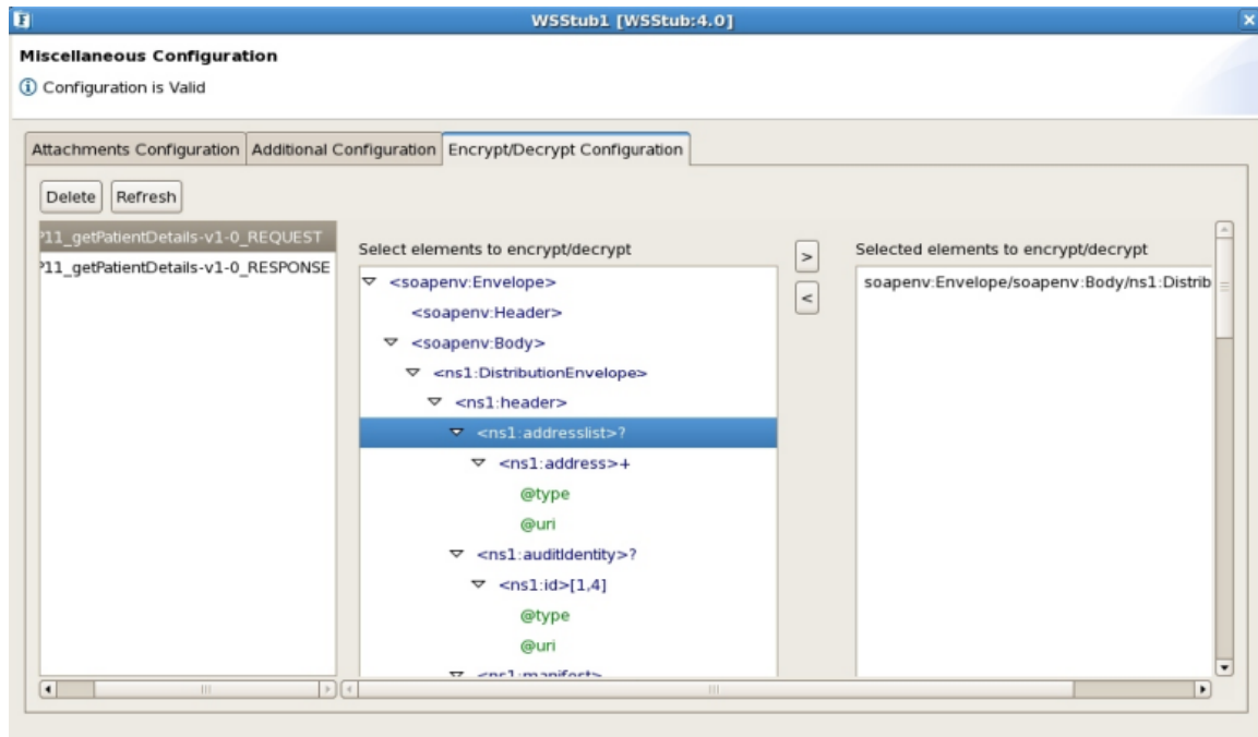
Figure 48: Encrypt/Decrypt Configuration Page in WSStub with Single Operation
