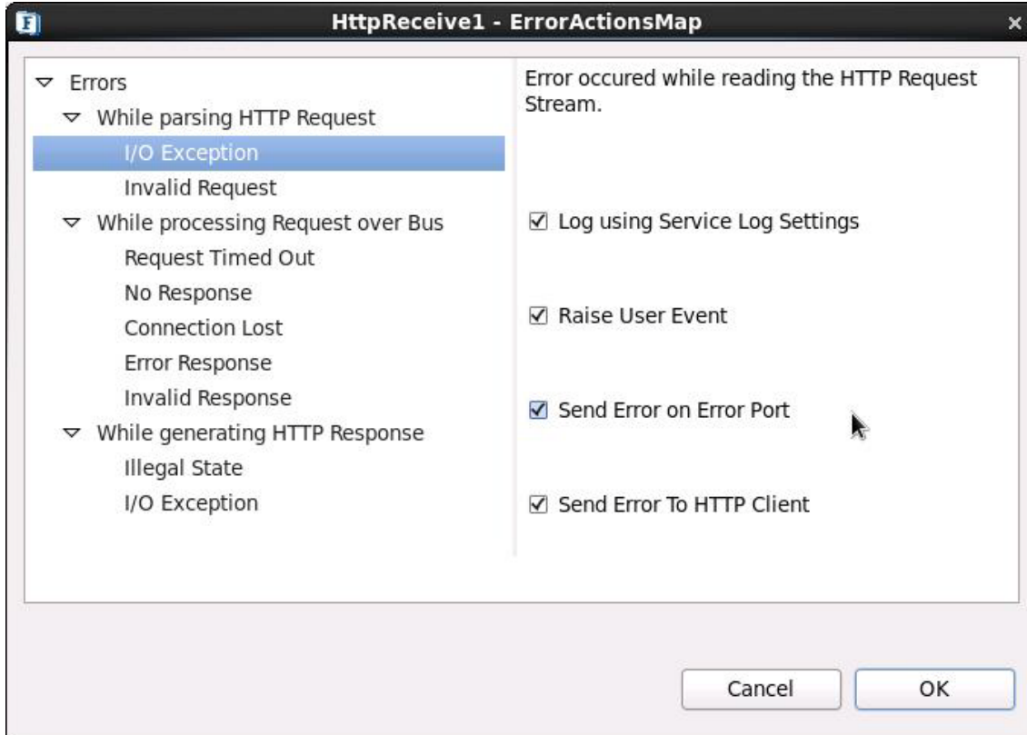
Figure 8: Configuration of Error Actions Map
