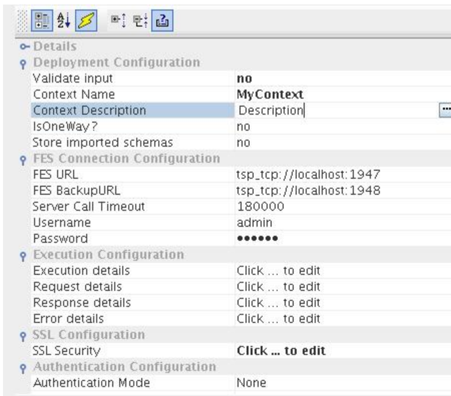
Figure 1: Configurable properties for HTTPStub component
