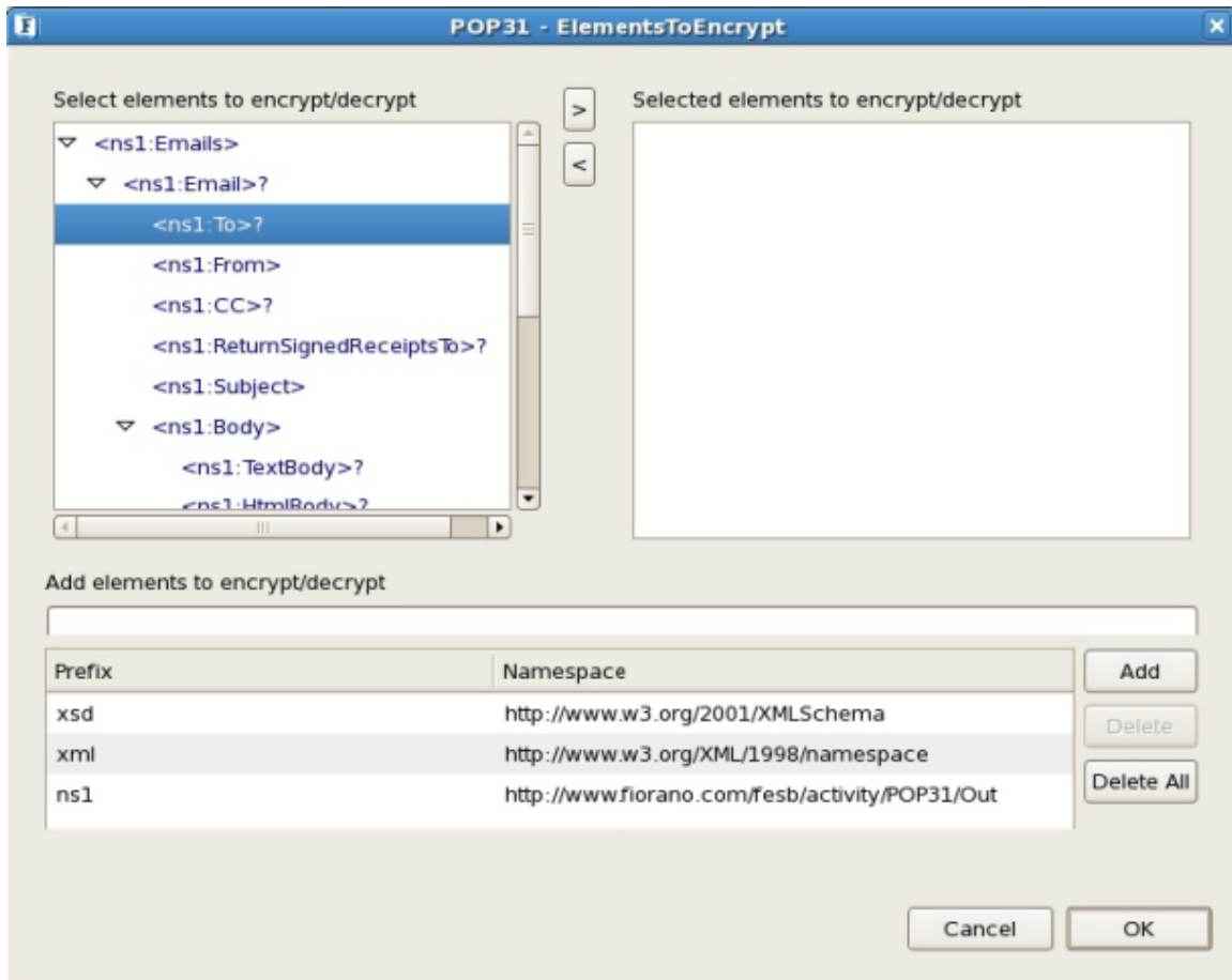
Figure 44: Encrypt/Decrypt Configuration Page in POP3
