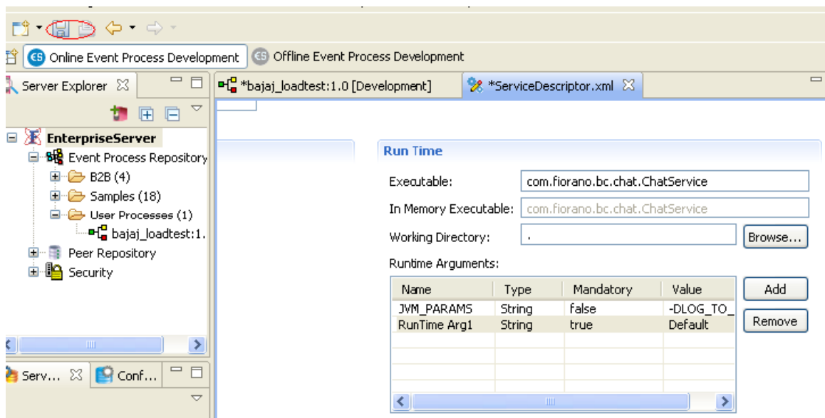
Figure 3.4.14: Save new Component
