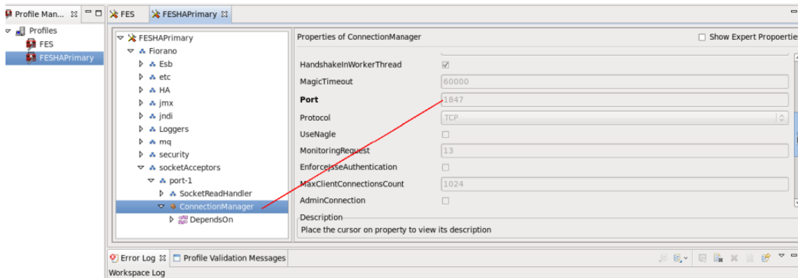
Figure 7: Configuration of the Fiorano ConnectionManager
