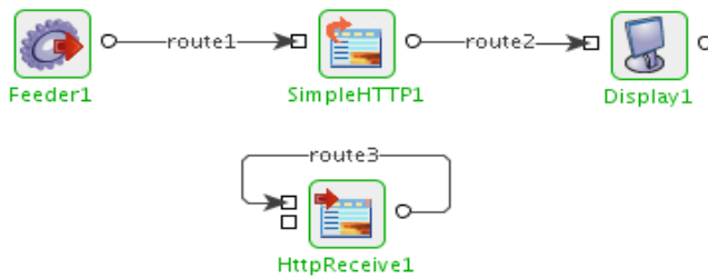
Figure 4.489: Demonstrates using SimpleHTTP component to post data
