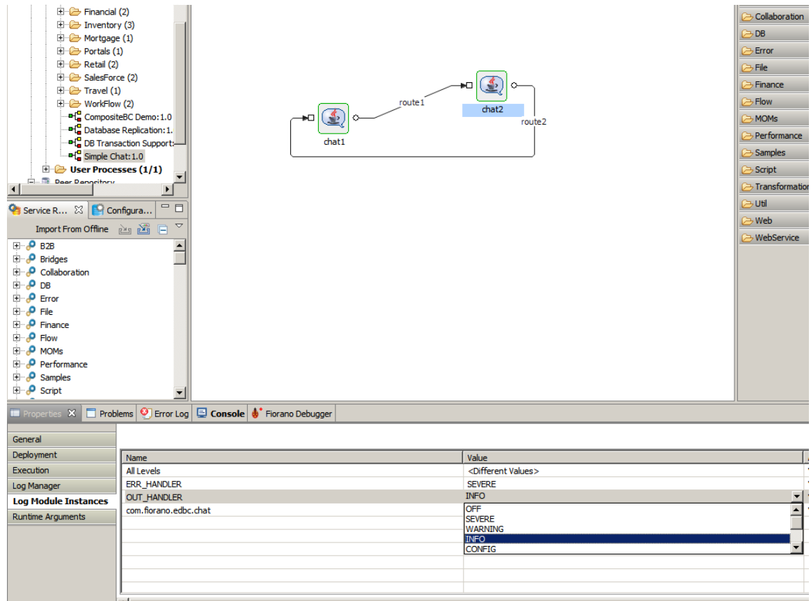
Figure 5.5.1: Configuring Log Module
