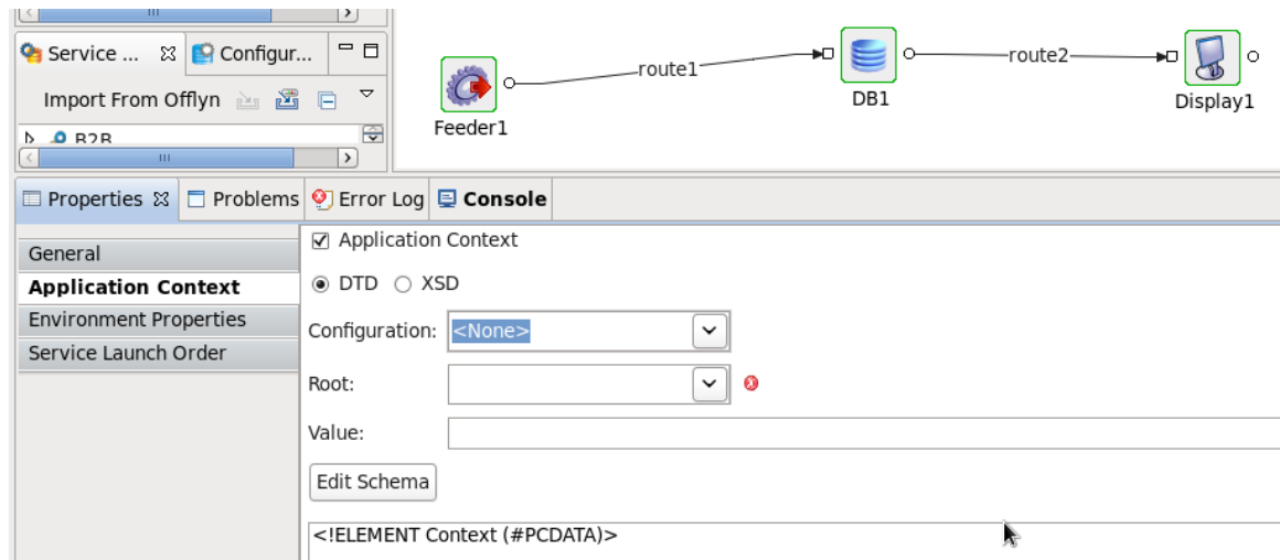
Figure 5.3.13: Adding Application Context
