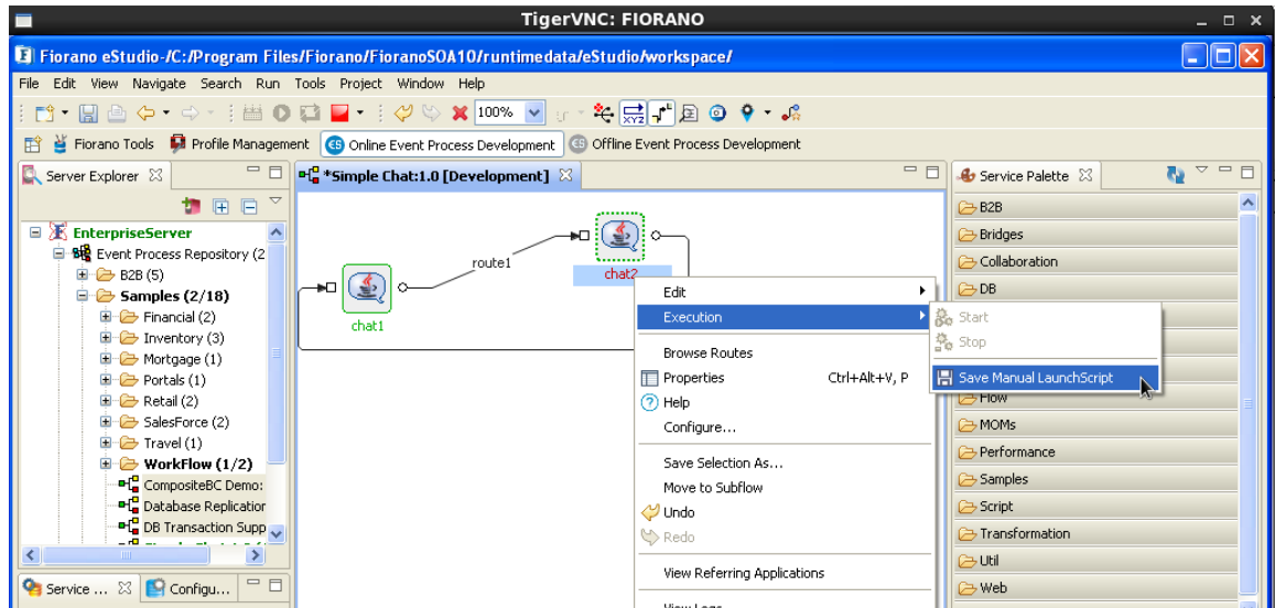
Figure 5.11.4: Save Manual Launch Script
