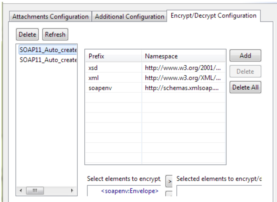
Figure: Encrypt/Decrypt Configuration
