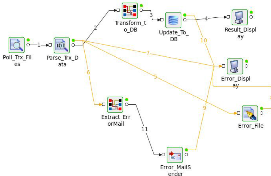
Figure 5.14.8: Revenue Control Packet Event Process Diagram
