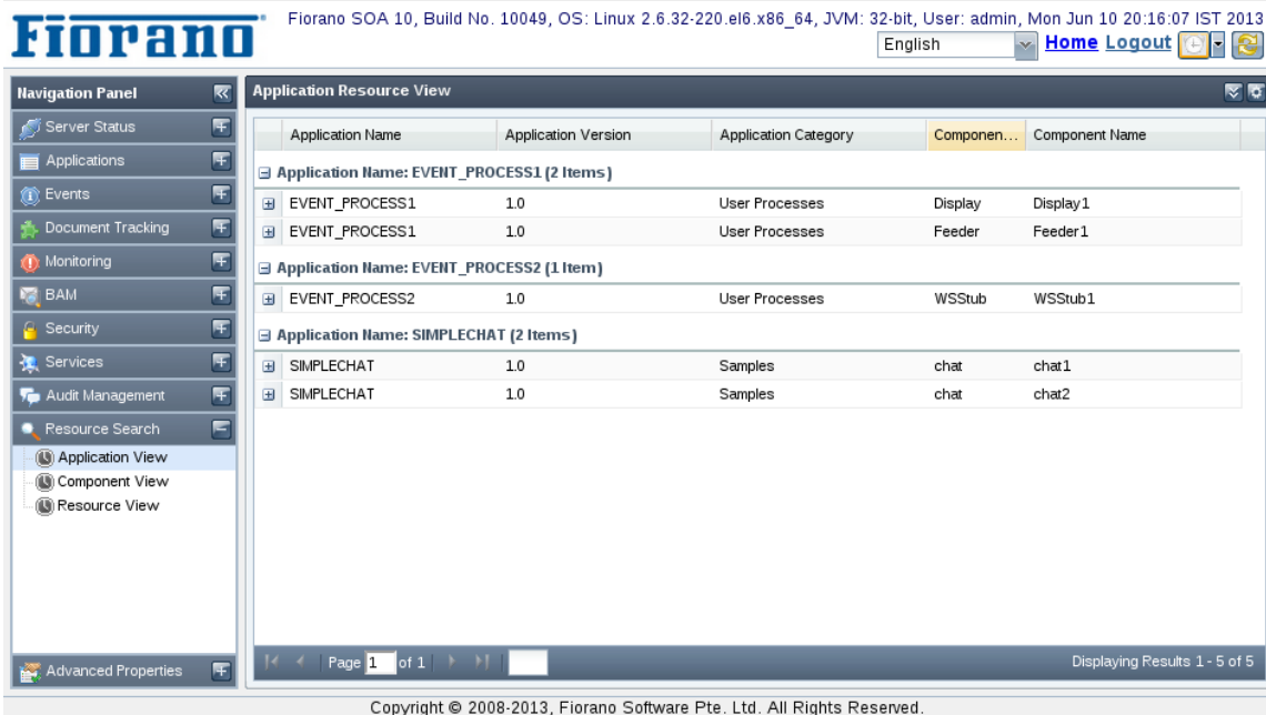
Figure 2.5.33: Searching configured resources based on application view
