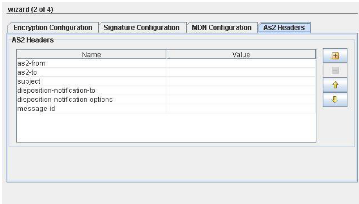
Figure 7: AS2 Headers details
