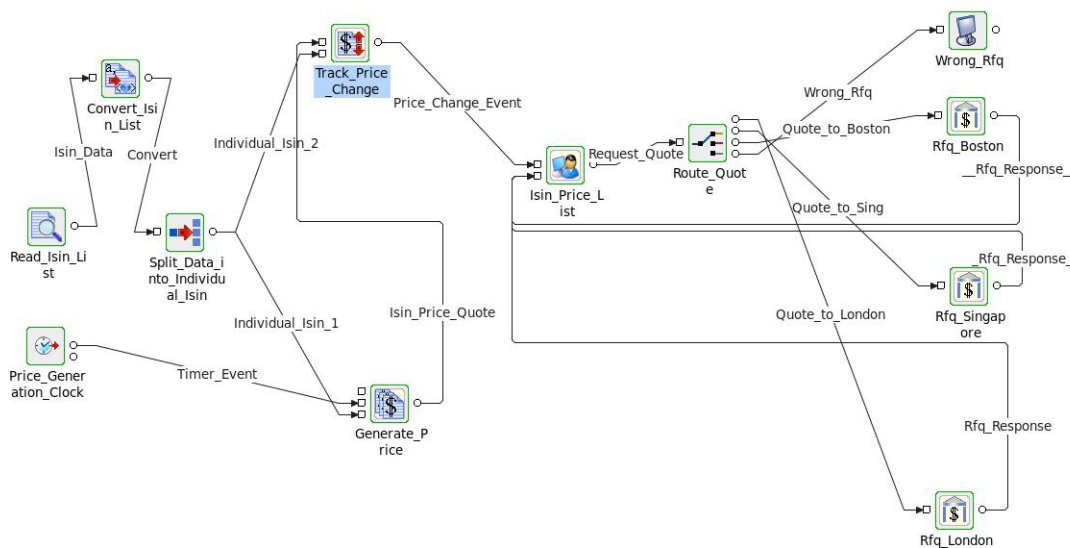
Figure 5.14.1: Bond Trading Event Process Diagram
