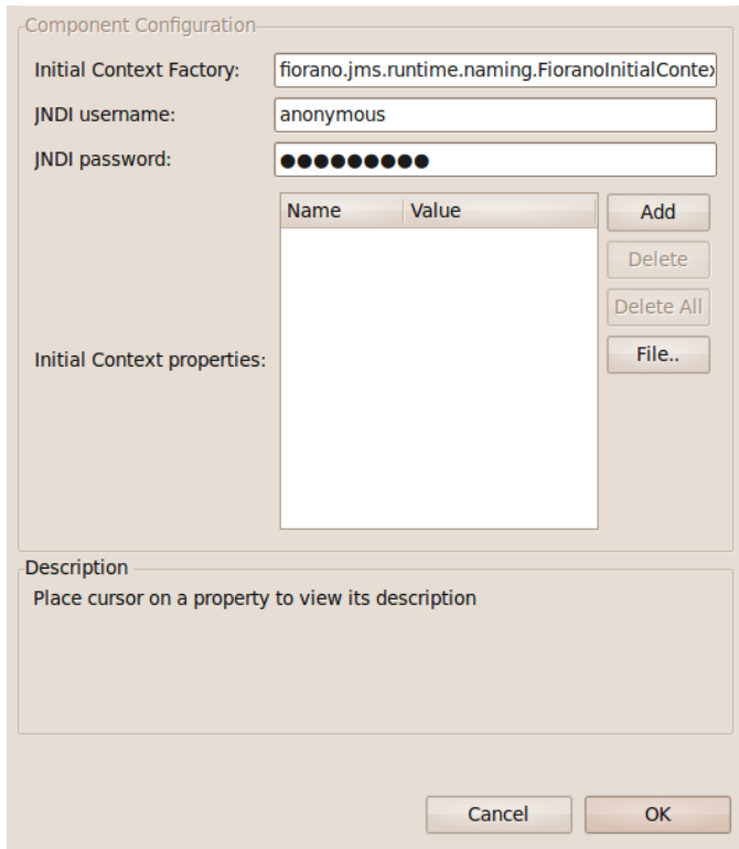
Figure: JNDI Settings
