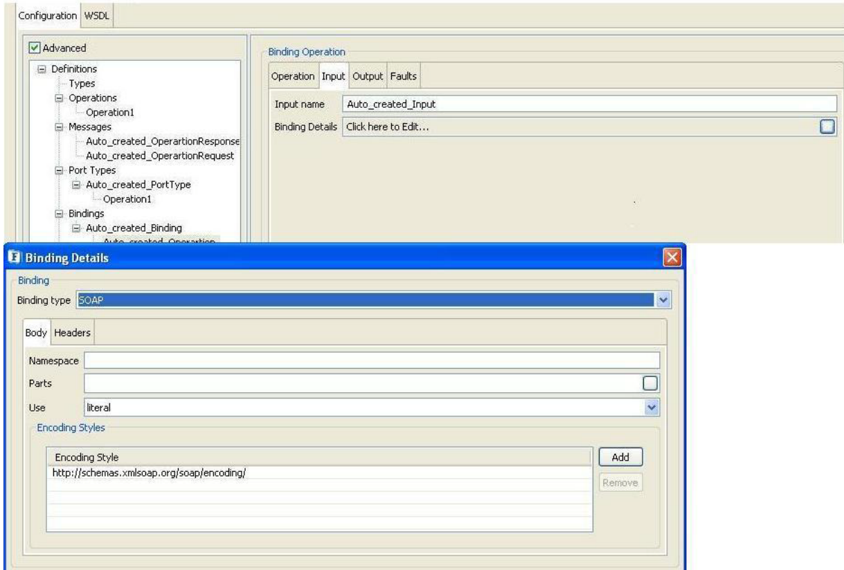
Figure: Binding input Configuration
