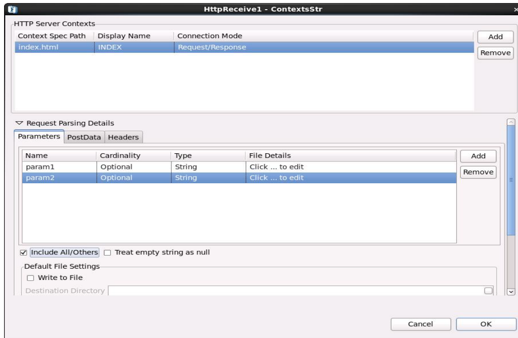
Figure 3: Configuration of Request Parsing Details
