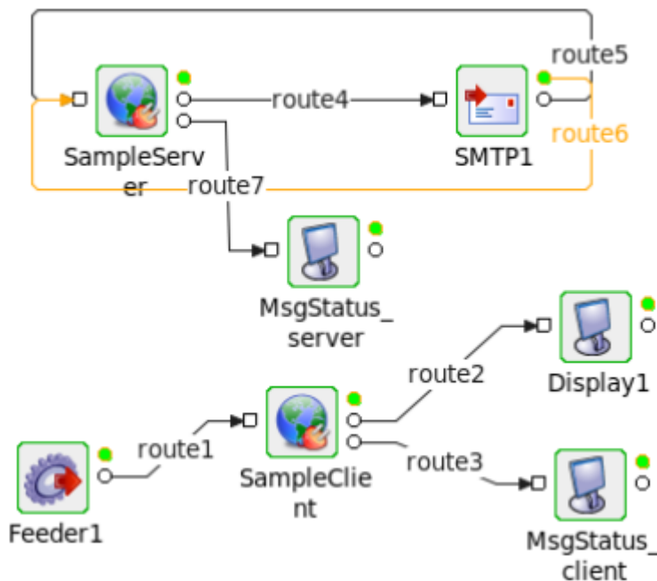
Figure 3: Socket Adapter Configuration in Server mode
