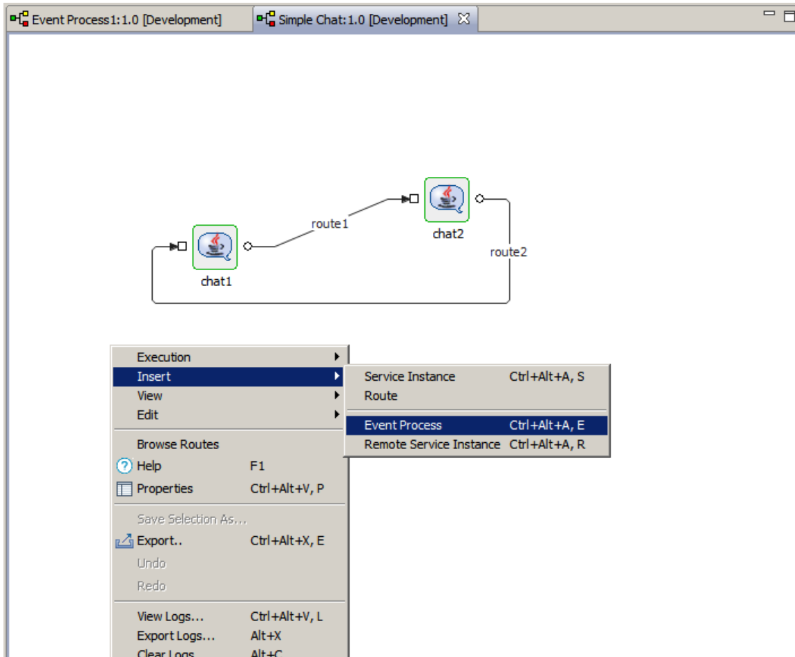
Figure 5.4.5: Adding Event Processes
