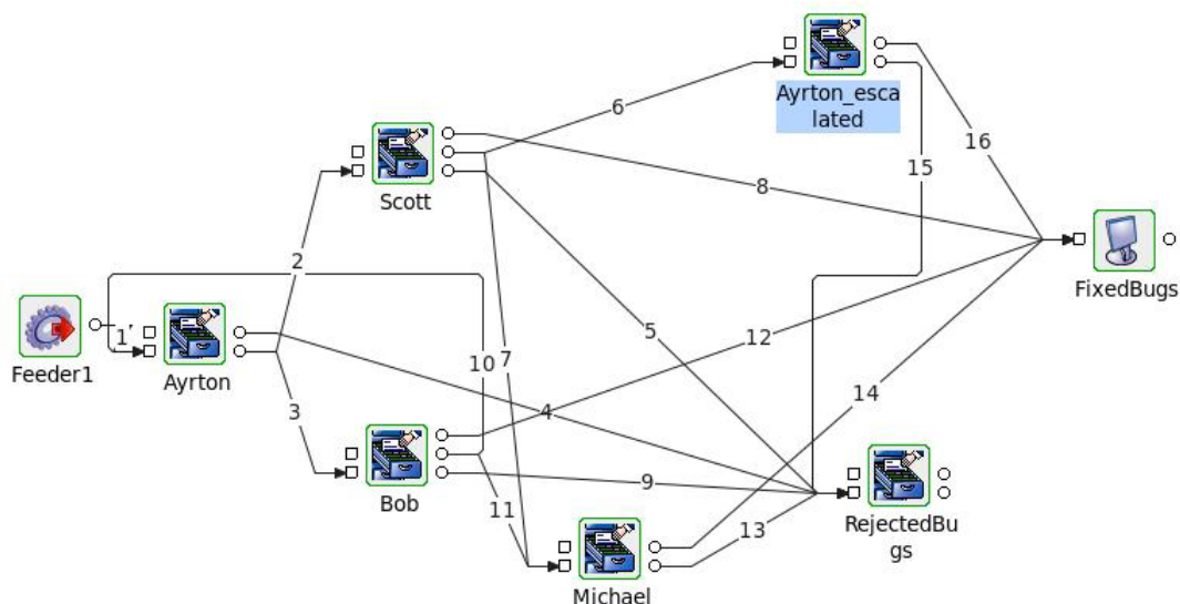
Figure 5.14.10: WorkList Sample Event Process Diagram
