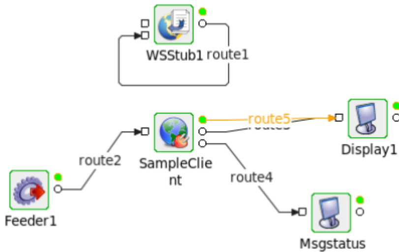
Figure 8: Sample Event Process
