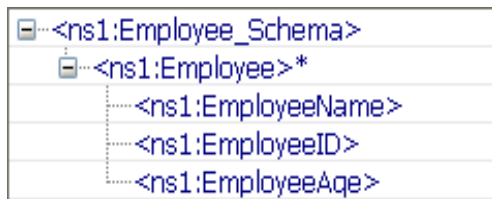
Figure 3: Schema for Employees details
