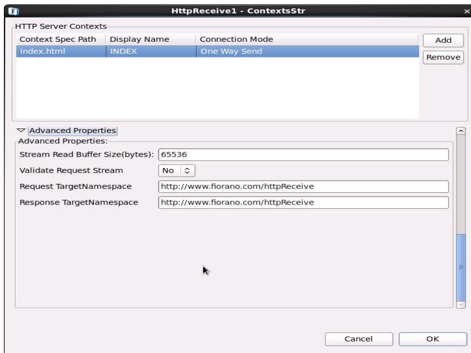
Figure 7: Advanced Properties - One Way Send
