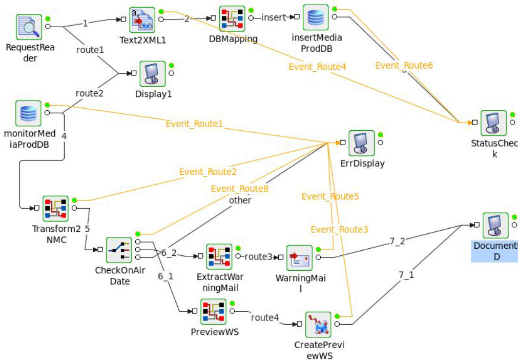
Figure 5.14.7: Retail Television Event Process Diagram
