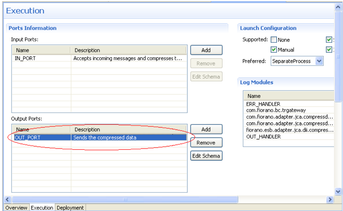
Figure 3.4.6: Modify the port properties required
