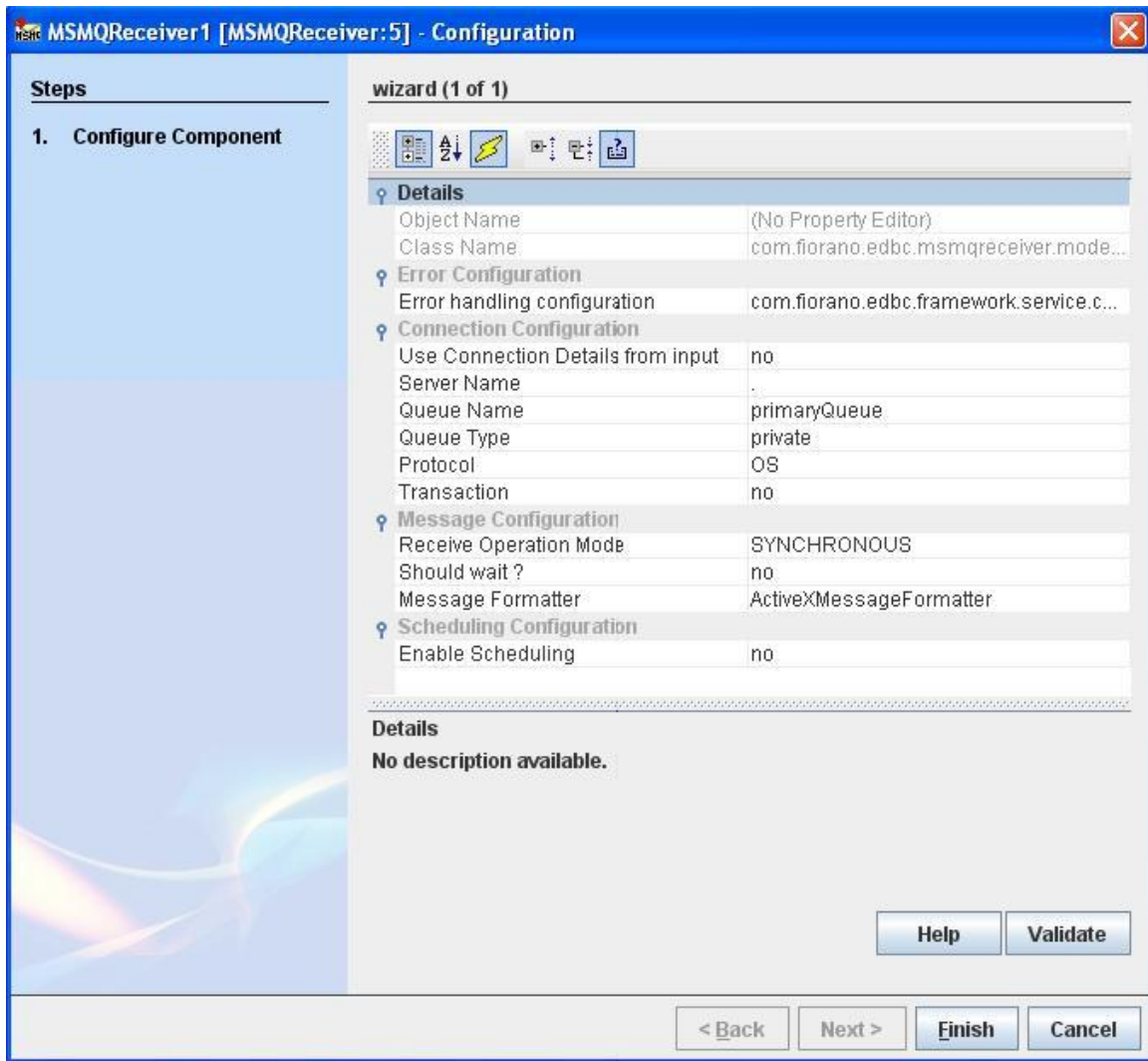
Figure 1: Sample MSMQ server configuration
