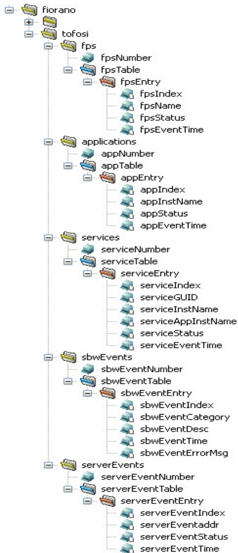
Figure 2.6.22: Fiorano Platform MIB tree
