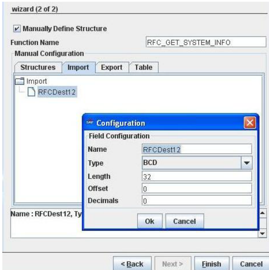
Figure 3: Defining parameters manually
