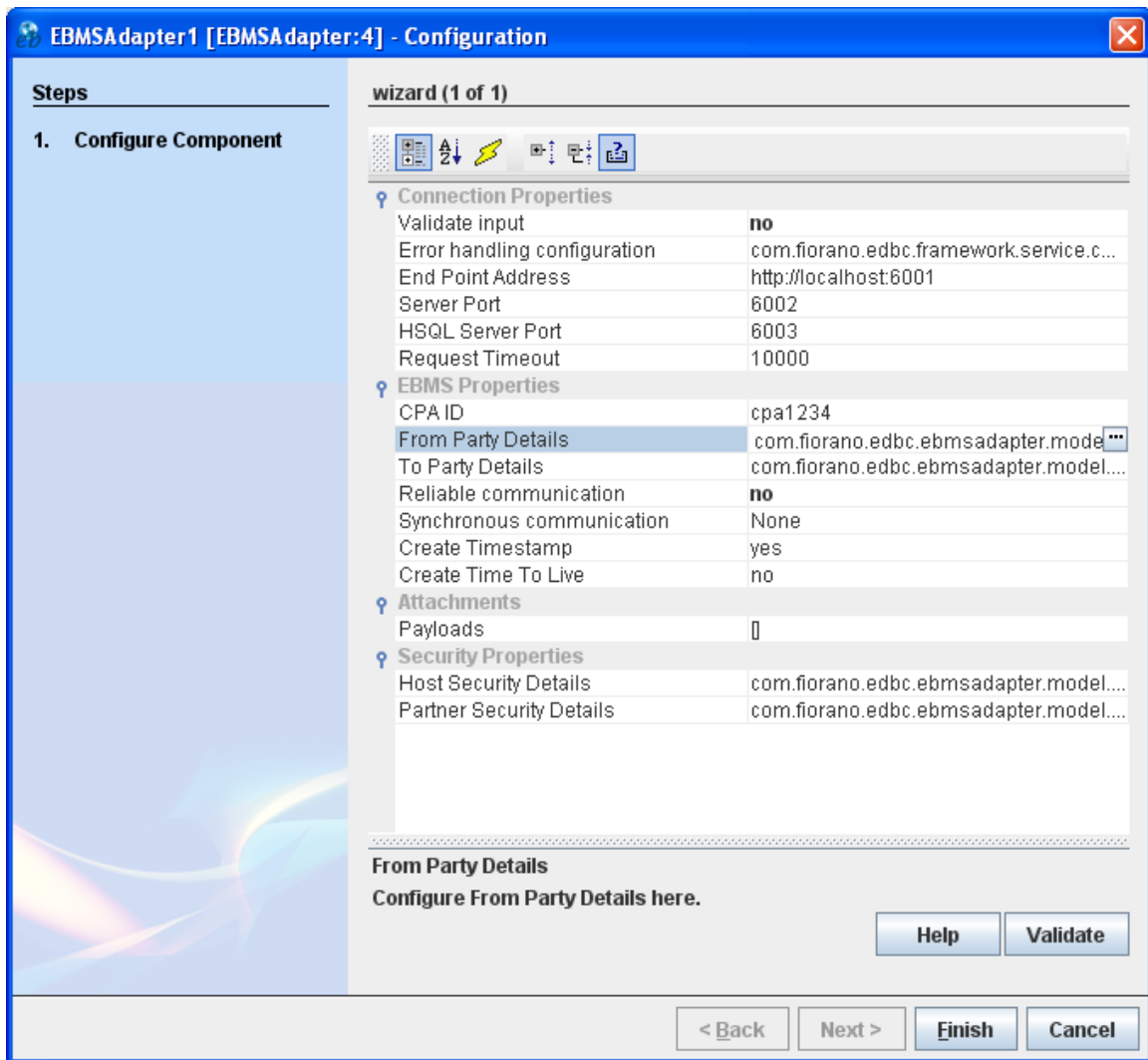
Figure 1: Configuration Property Sheet
