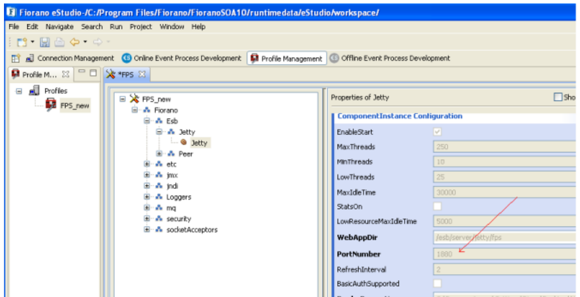
Figure 2.4.15: Changing Jetty port
