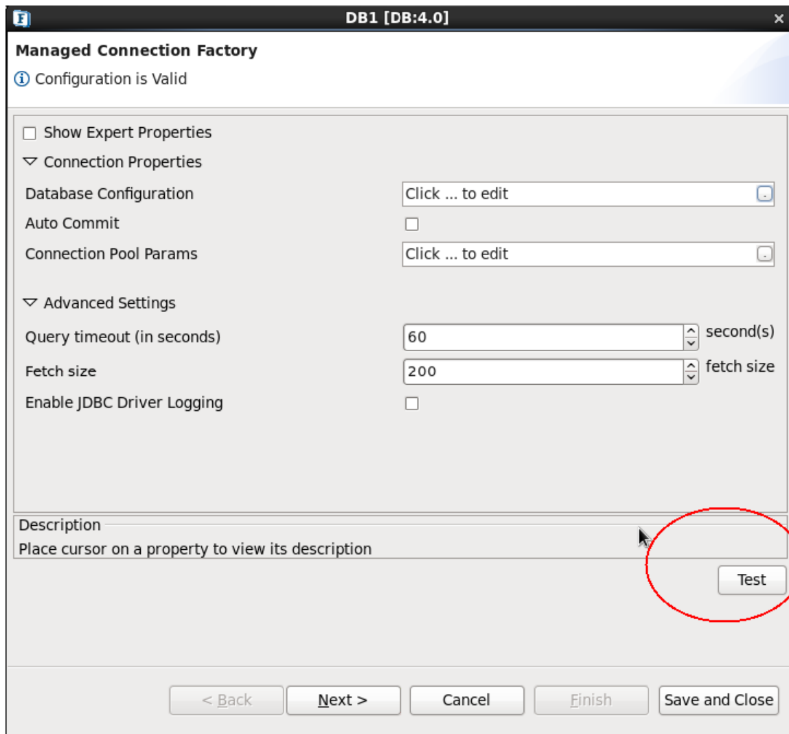
Figure 3.7.1: Managed Connection Factory (MCF) panel showing the connection details and Test button
