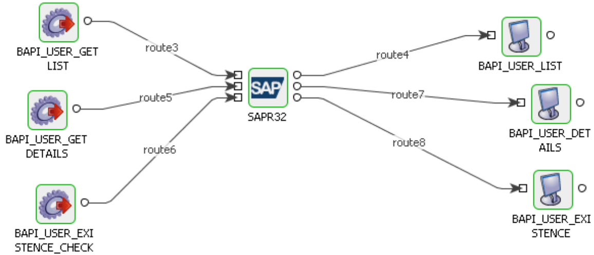
Figure 4: SAPR3 Component configured to invoke multiple BAPIs
