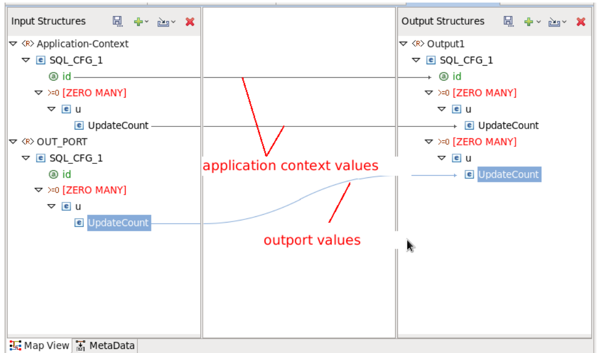
Figure 5.3.17: Demonstrates the Transformation
