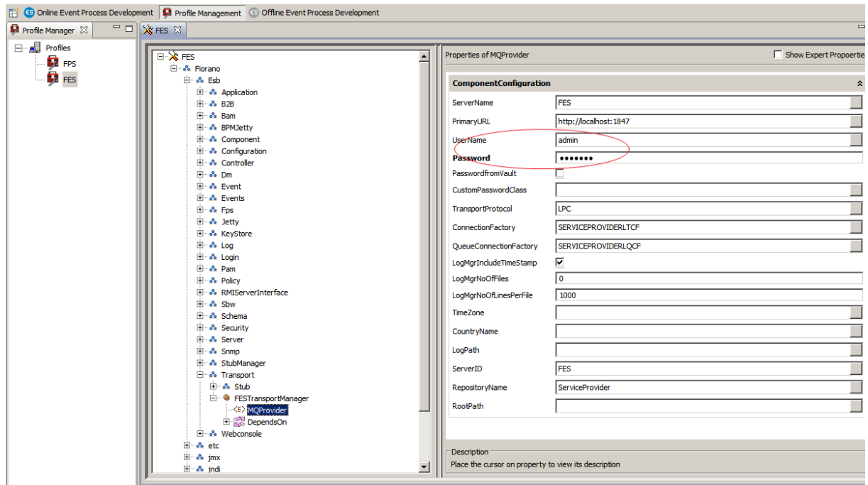
Figure: Changes to reflect password change for Admin user
