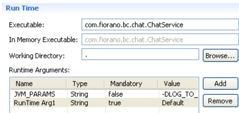
Figure 3.4.12: Menu to add additional parameters to execution
