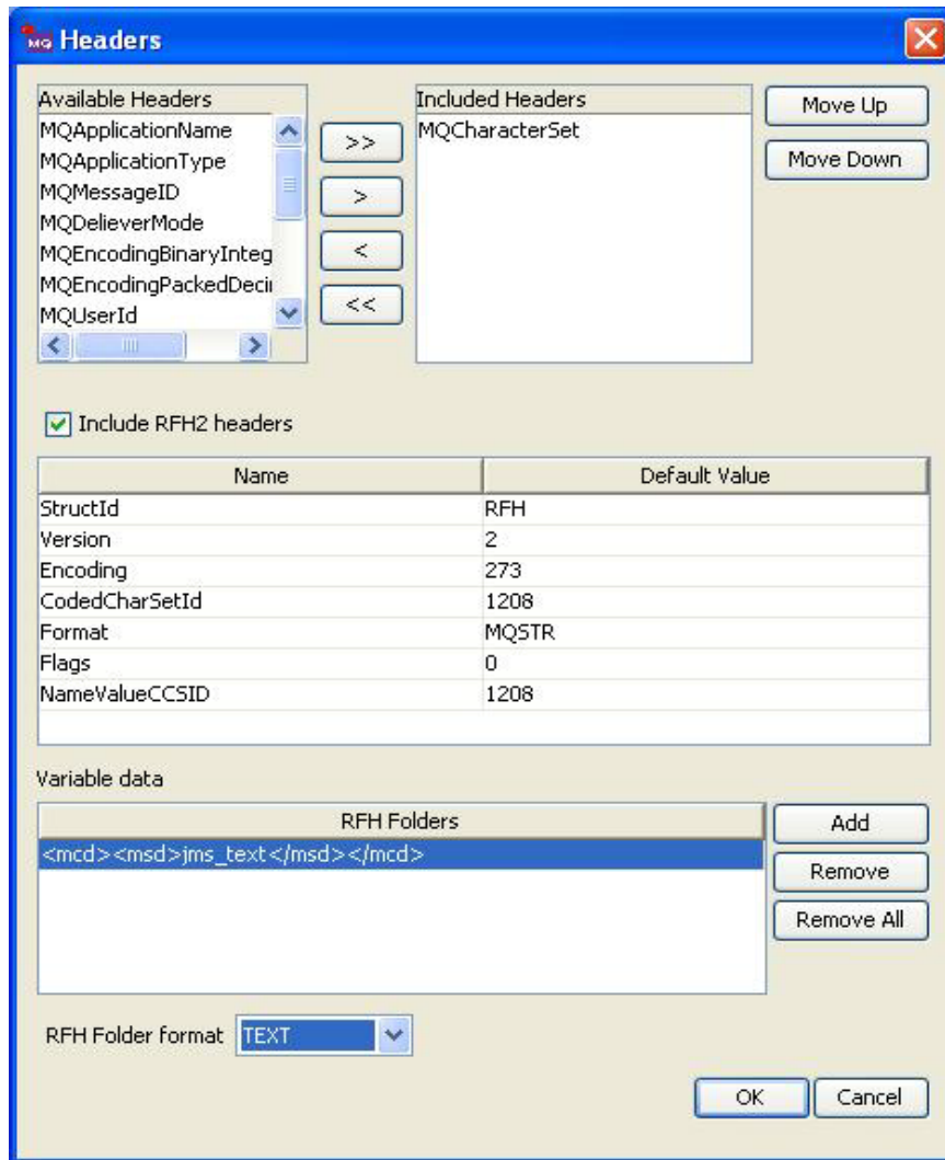
Figure 31: Headers defined for scenario 2
