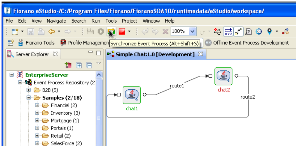
Figure 5.10.5: Event Process Synchronization
