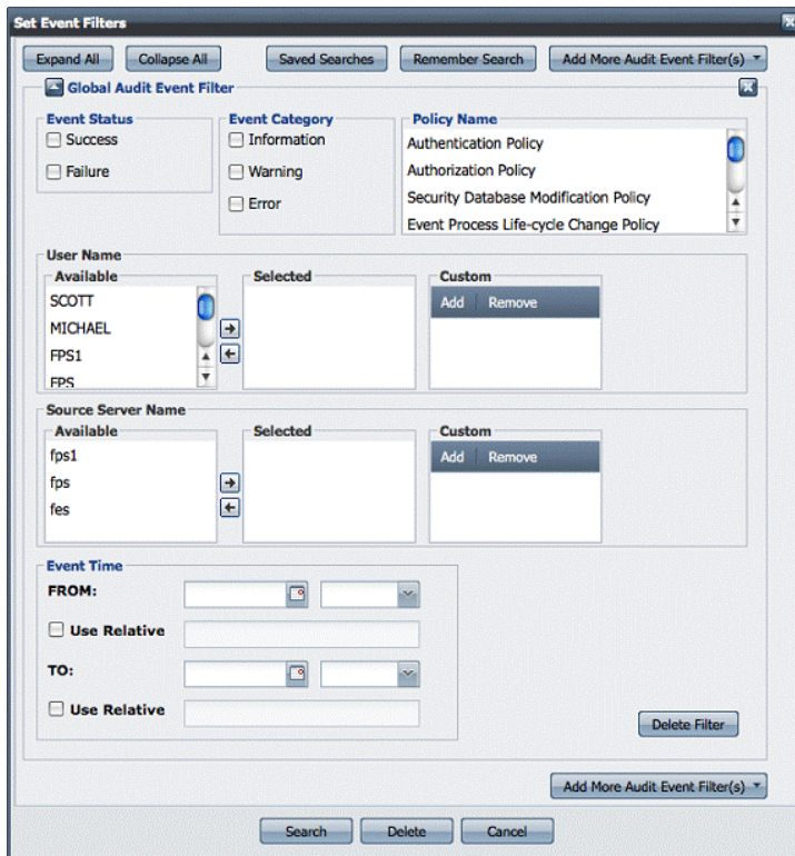
Figure 12.3: Set Event Filters
