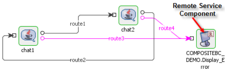
Figure 5.4.3: Using a Remote Service Component in an Event Process
