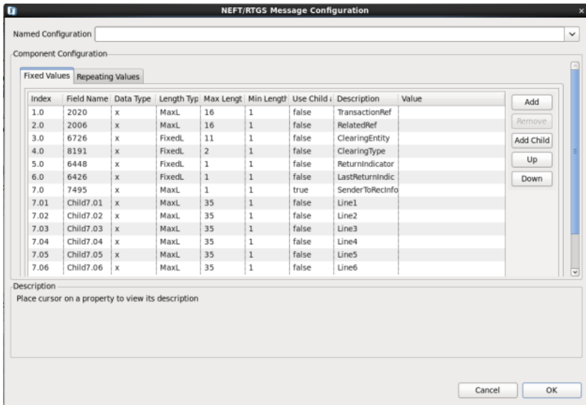
Figure 3: NEFT/RTGS Block4 (Body) Message panel
