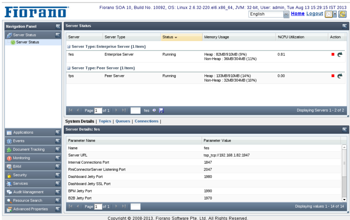
Figure 2.5.2: Server Status tab showing System details
