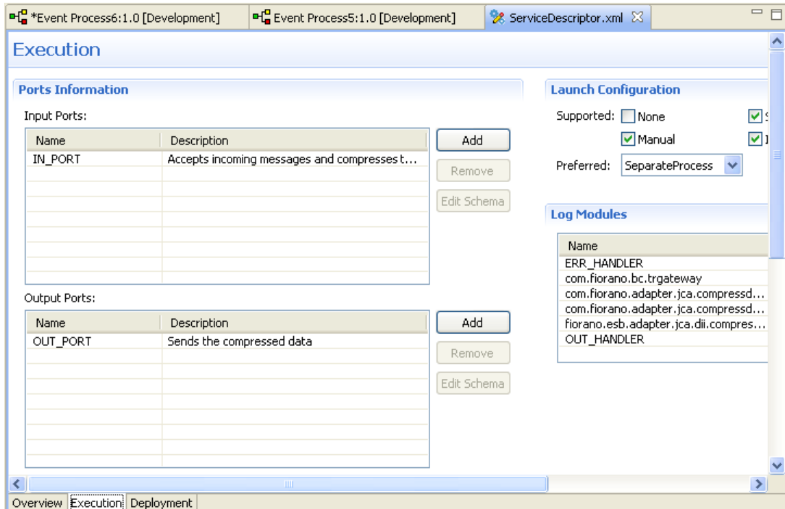
Figure 3.4.3: Execution information for new component registration
