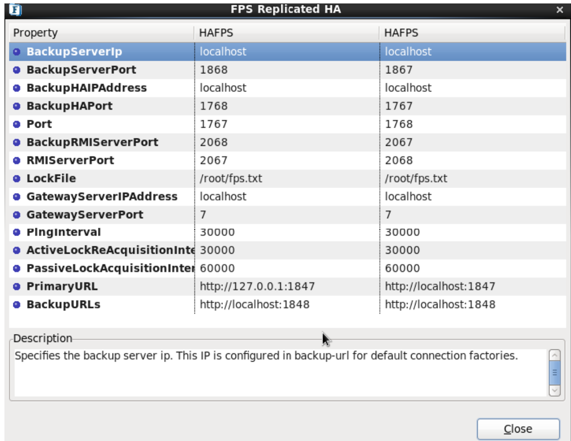
Figure 10: FPS Replicated HA dialog box
