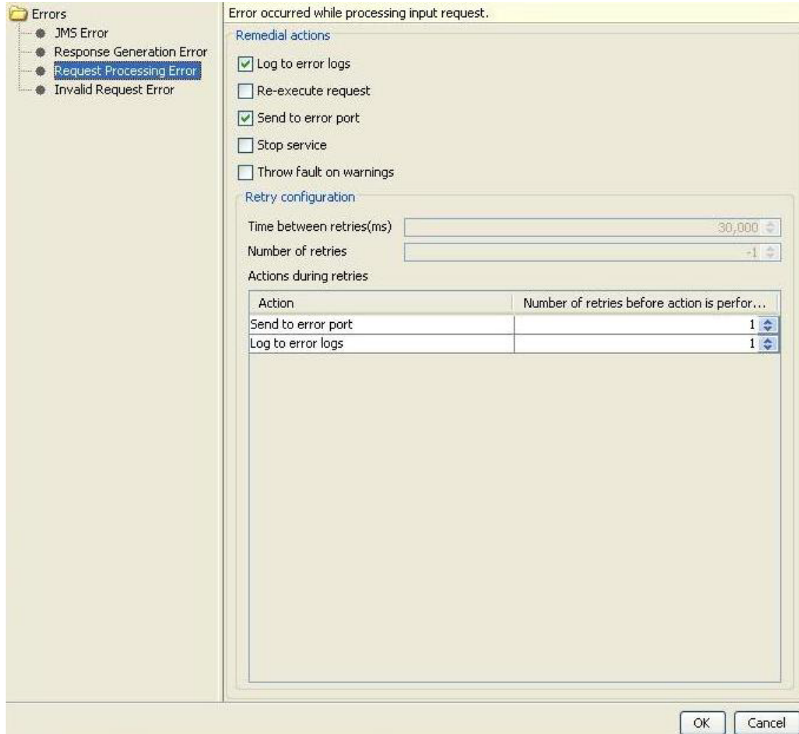
Figure 3: Error Handling Configuration
