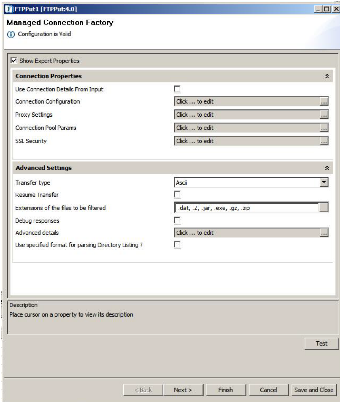
Figure 1: Managed Connection Factory panel
