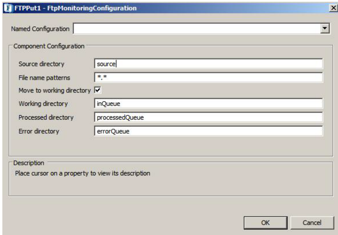
Figure 15: Sample monitoring configuration
