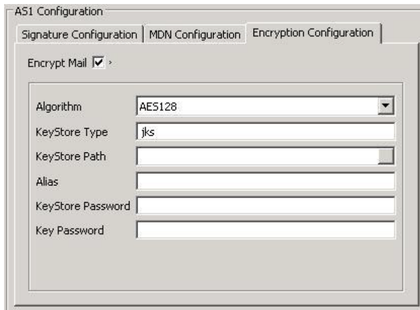
Figure: Encryption configuration details
