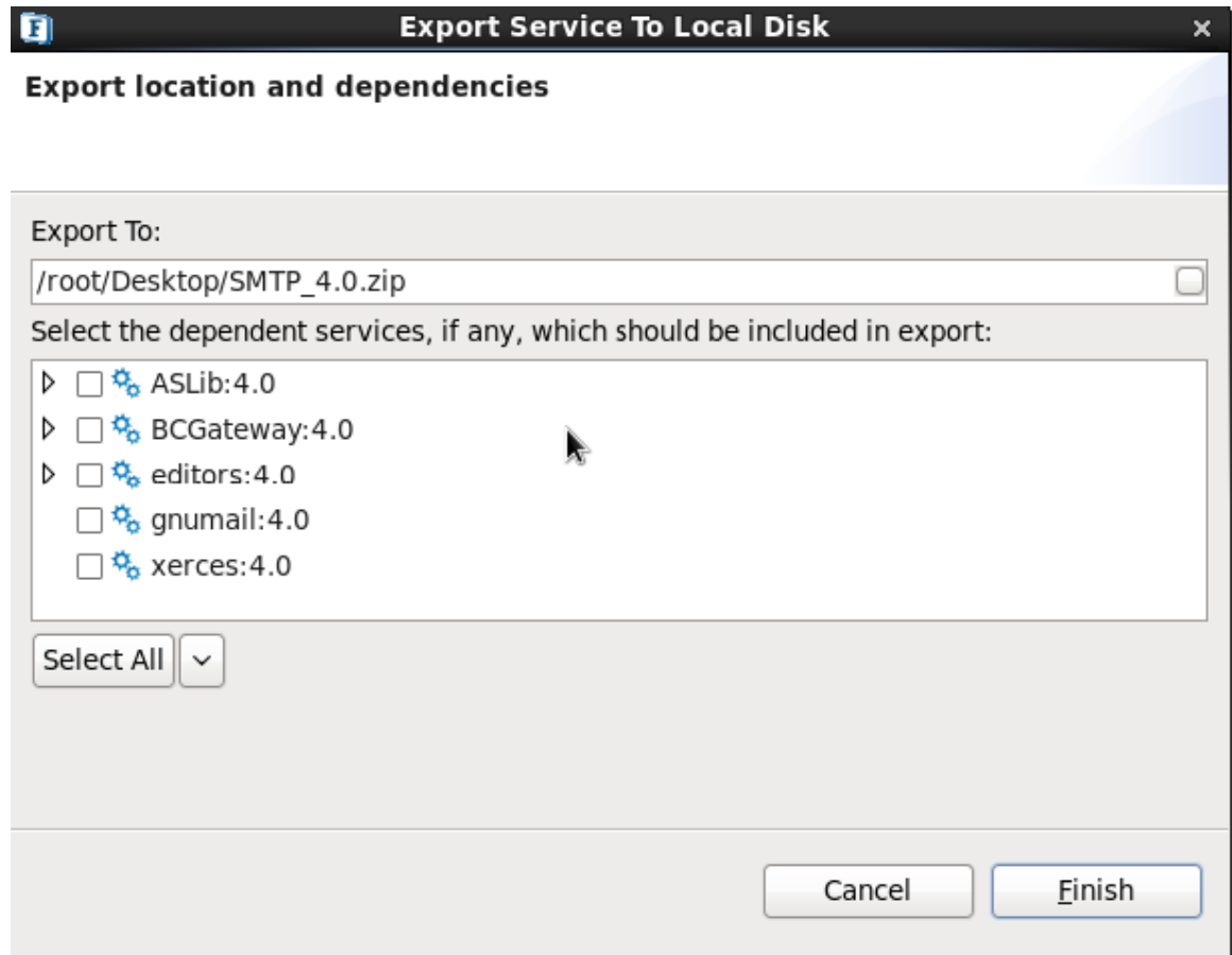
Figure 3.5.2: UI to save the exported component and its libraries
