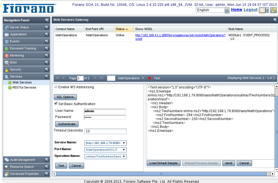
Figure 2.5.32: Web Services tab
