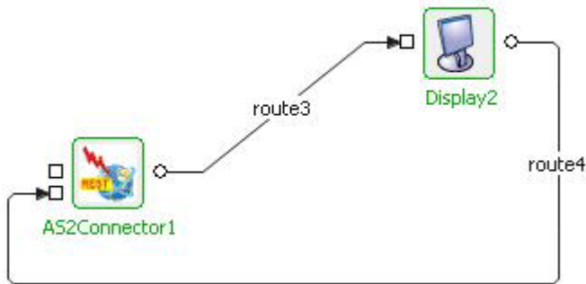
Figure 13: Sample Event Process demonstrating RECEIVE mode
