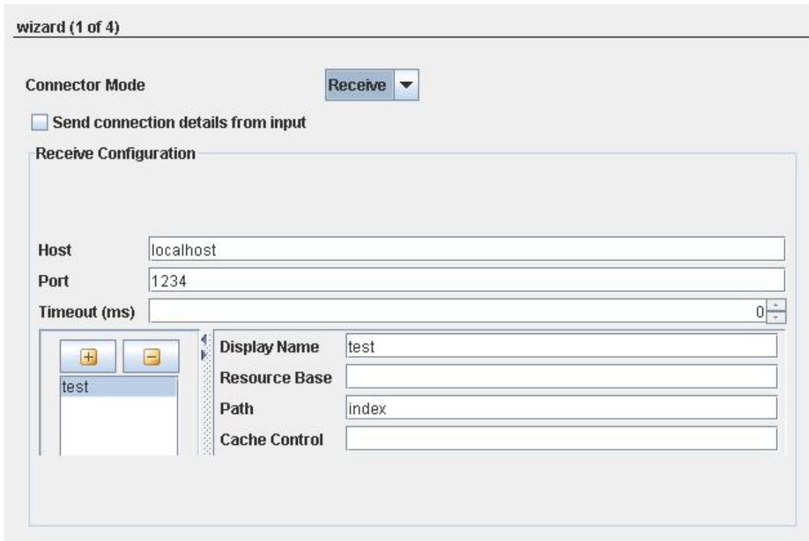
Figure 3: Receive configuration details
