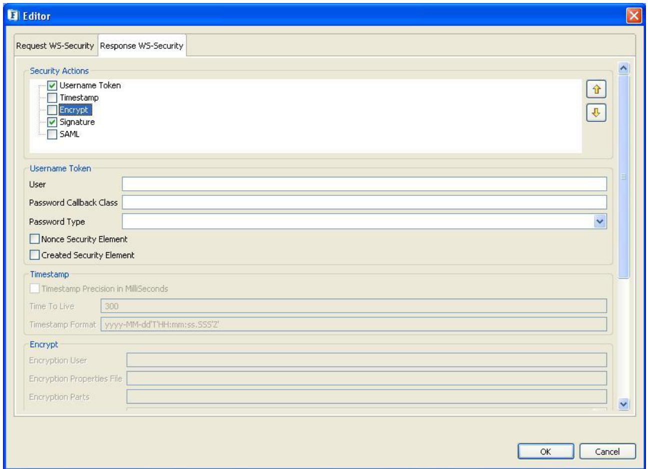
Figure 4.516: WS Request Security
