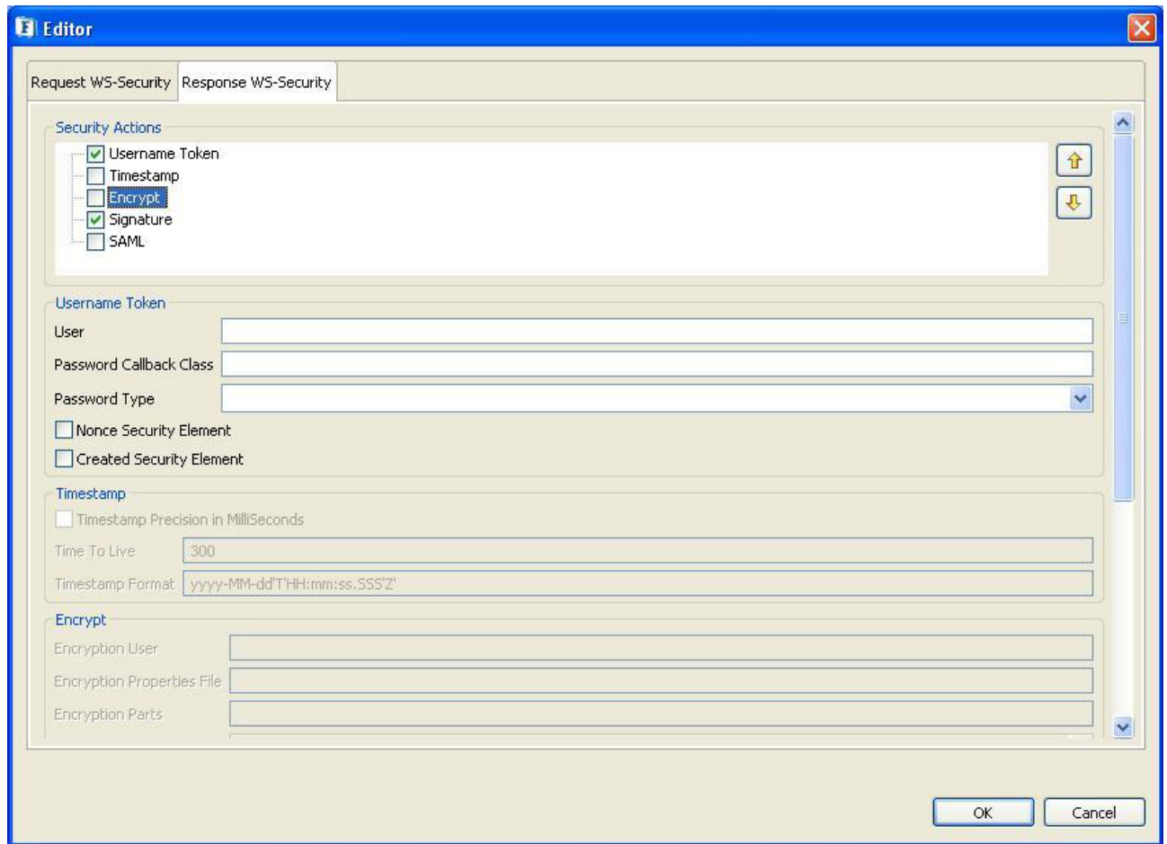
Figure 4.517: WS Response security
