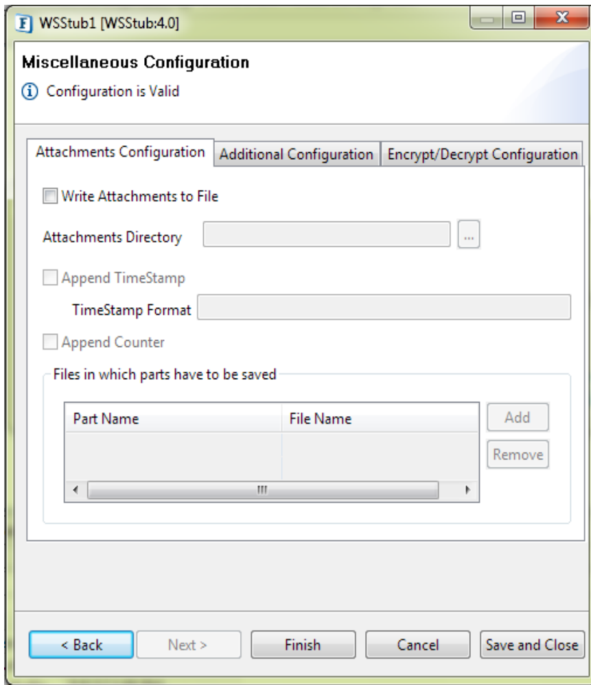
Figure: Attachments Configuration
