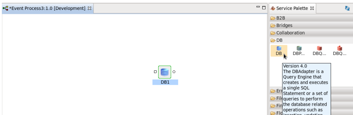
Figure 5.2.1: Drag-drop service component
