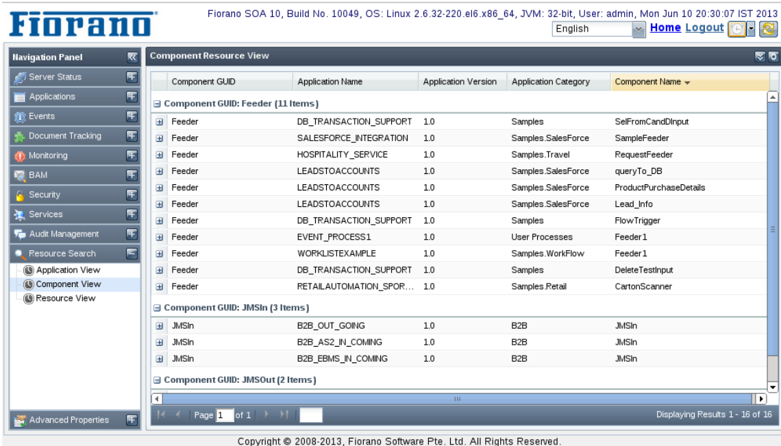
Figure 2.5.34: Searching configured resources based on component view
