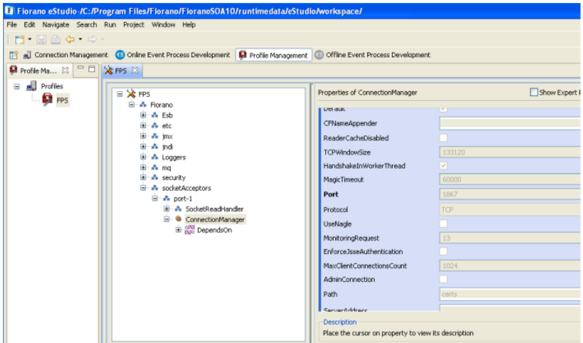
Figure 2.4.3: FPS Server Port
