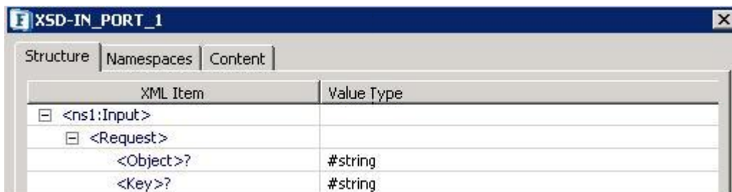
Figure 6: Input Schema for Select/Delete operation when Use Connection Details from input is set to "no".
