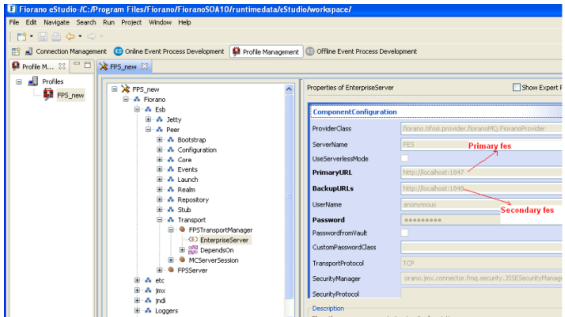
Figure 2.4.16: Enterprise server properties
