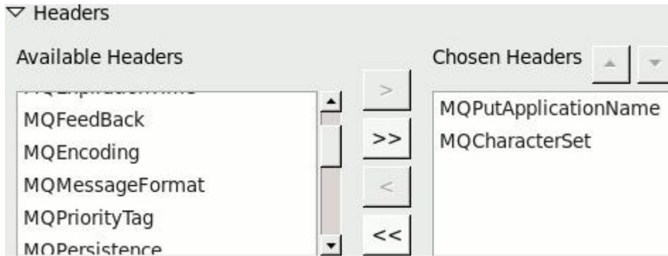
Figure 23: Selecting MQMD headers whose values have to be taken from input XML
