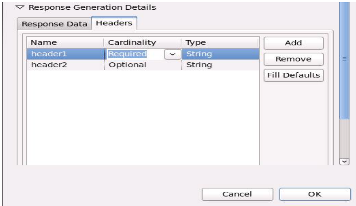
Figure 9: Sample Configuration of Response Generation Details – Headers
