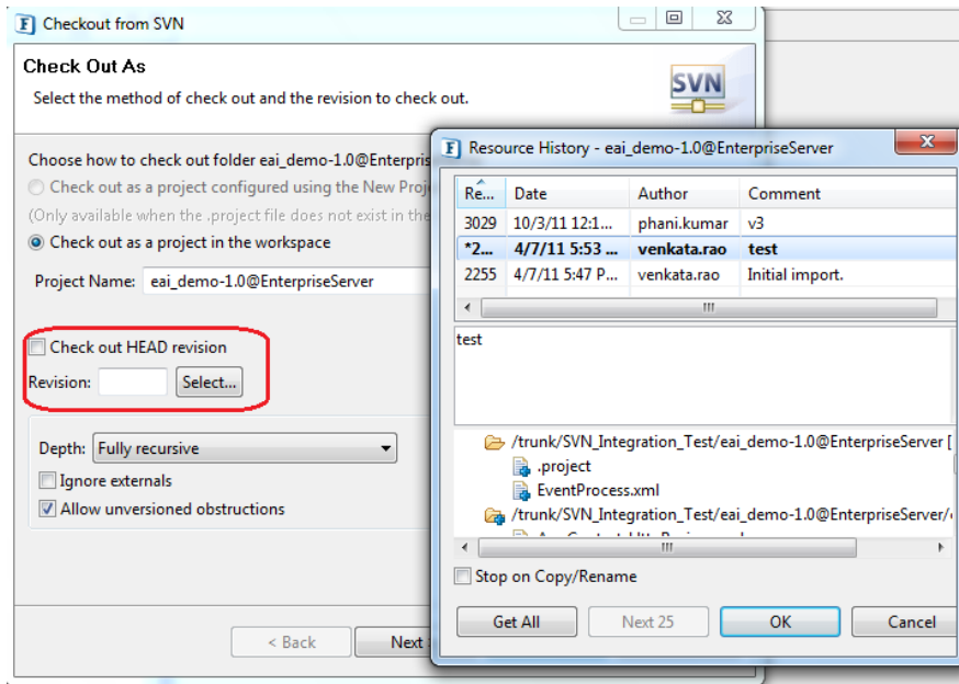
Figure 10: Checking out a selected version
