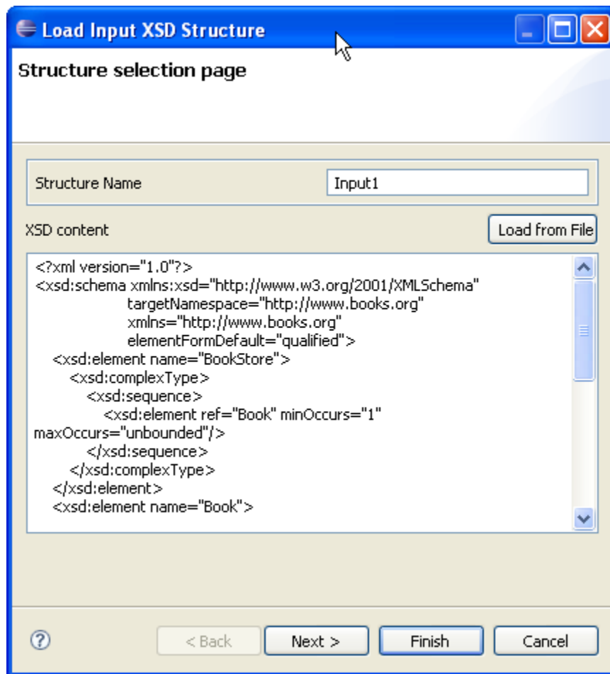
Figure 10.3.1: Structure Selection Page
