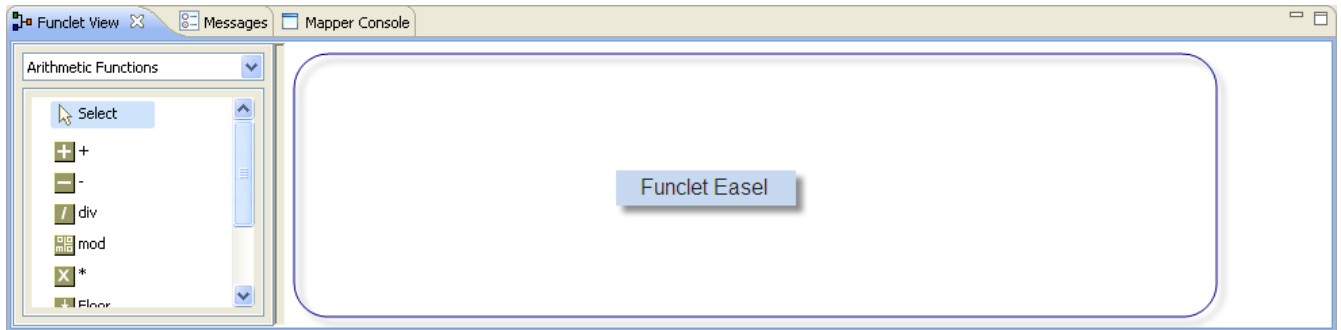
Figure 10.4 Funclet View
