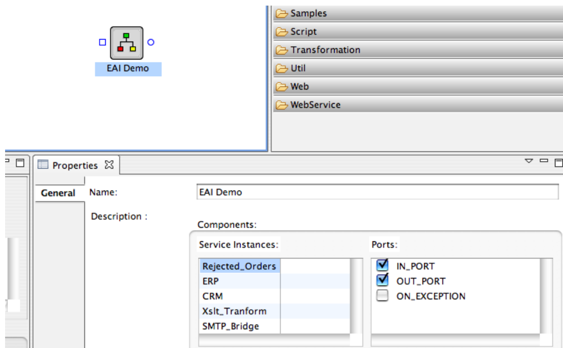
Figure 5.6.5: Properties tab
