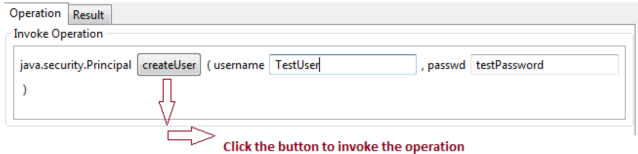
Figure 14: Operation signature
