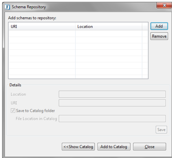
Figure 13.1.1: Schema Repository
