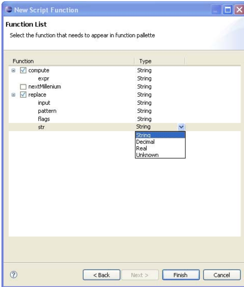
Figure 10.8.3 Function Page
