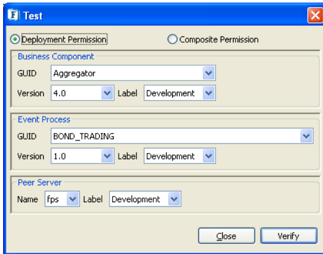
Figure 13: Test dialog
