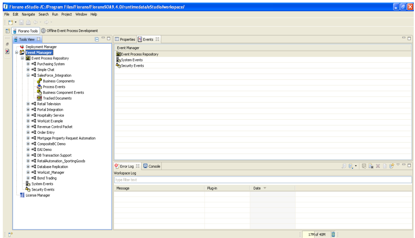
Figure 15: Events View
