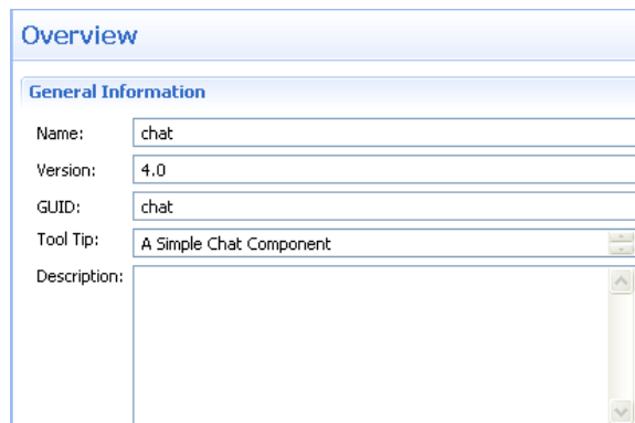
Figure 8.1.4: General Information
