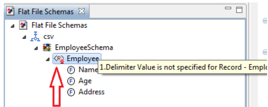
Figure 19.18: Schema Errors
