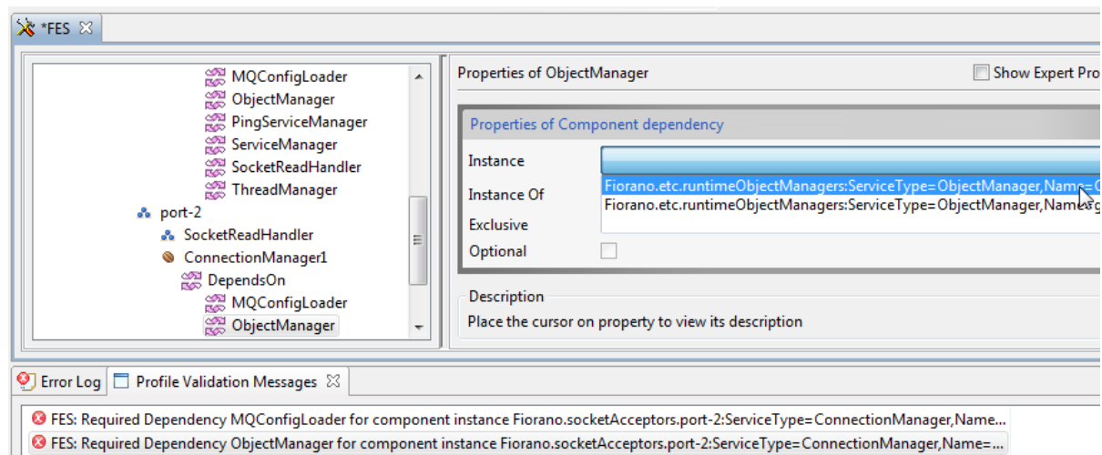
Figure 9: Resolving dependencies
