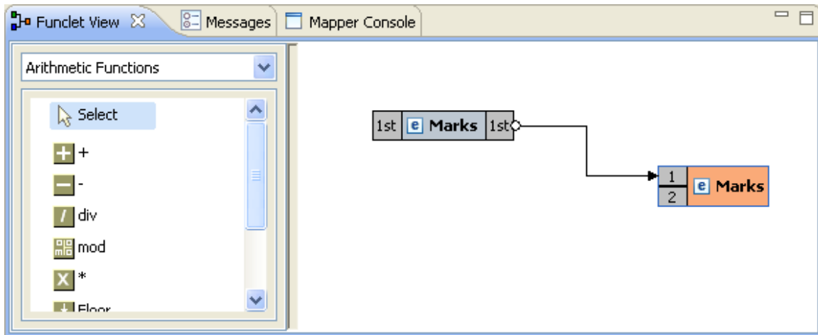
Figure 10.4.24: Funclet easel
