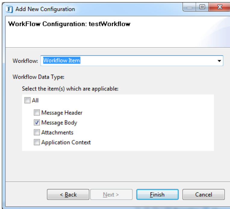
Figure 29: Workflow Configuration
