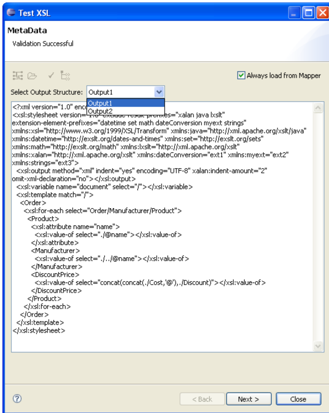
Figure 10.9.2: Metadata Page
