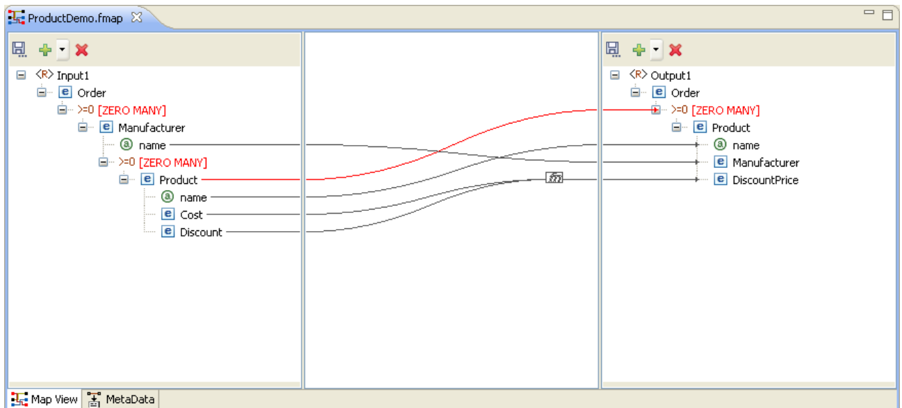
Figure 10.5.6: Name-to-name Mapping
