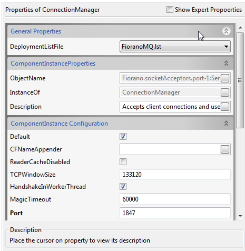
Figure 4: Properties UI
