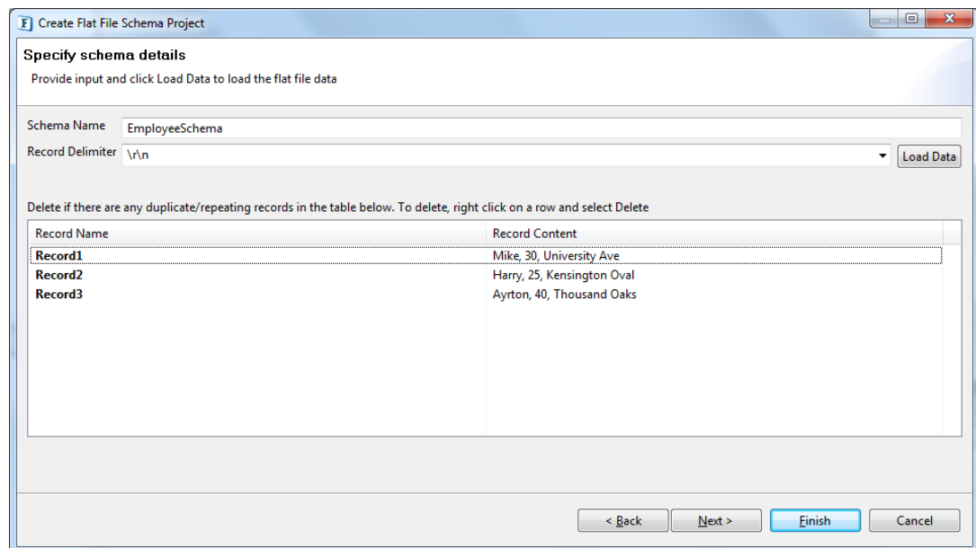
Figure 19.11: Schema configuration
