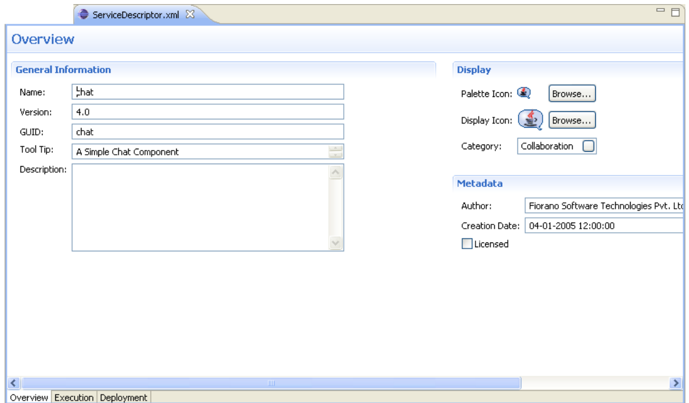
Figure 8.1.2: ServiceDescriptor.editor
