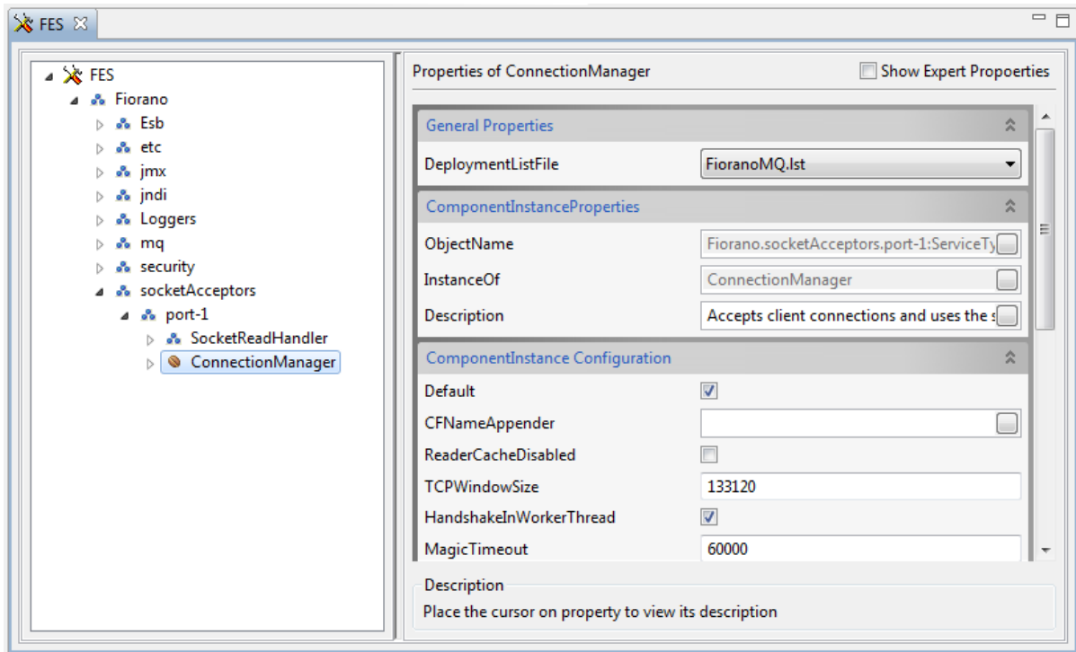
Figure 3: Profile Editor
