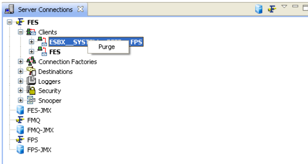
Figure 2: Purge Messages
