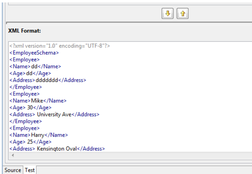
Figure 19.9: XML output
