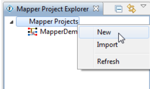
Figure 10.2.2: eMapper Projects
