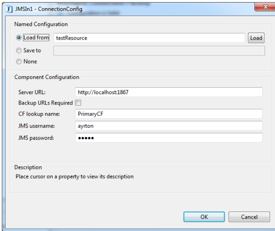
Figure 11: Loading Configuration
