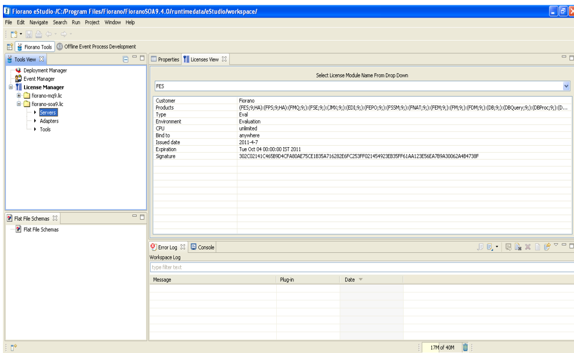
Figure 24: Licenses View
