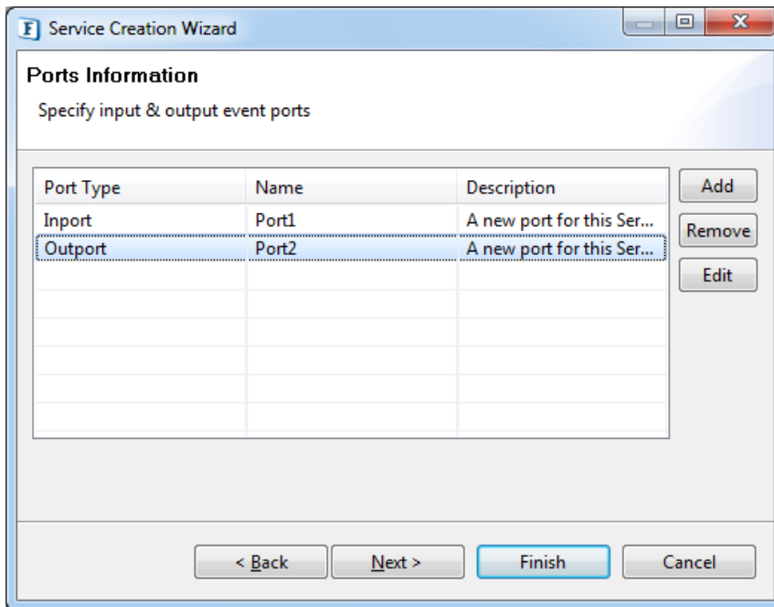
Figure 9.1.4: Ports Information
