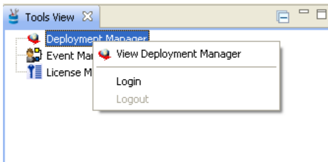
Figure 2: Tools View
