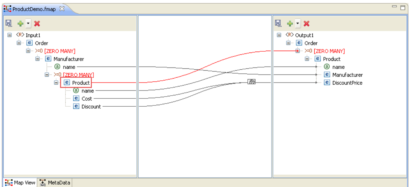
Figure 10.5.7: For-Each Mapping
