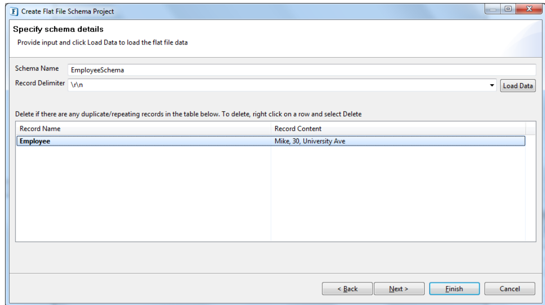
Figure 19.12: Configuring Records
