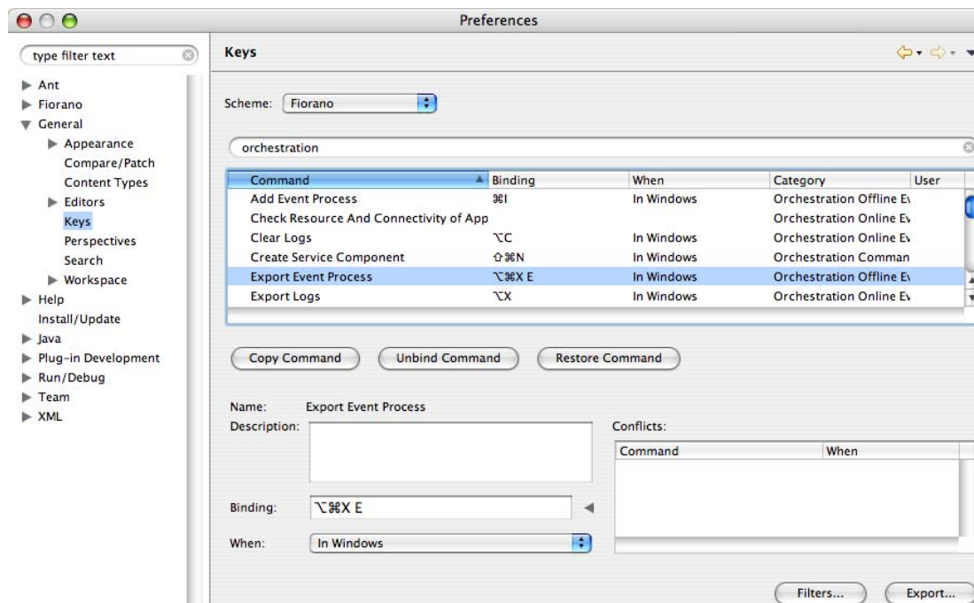
Figure 12.4.1: Key-binding preferences
