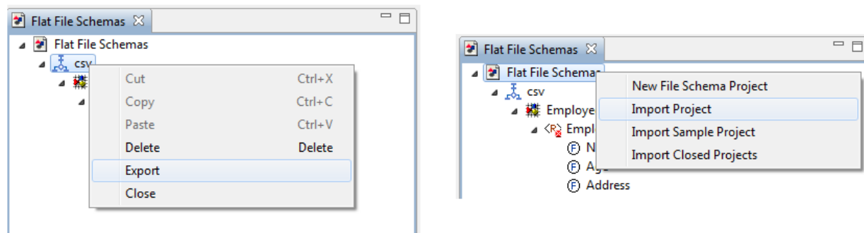
Figure 19.20: Import/Export project
