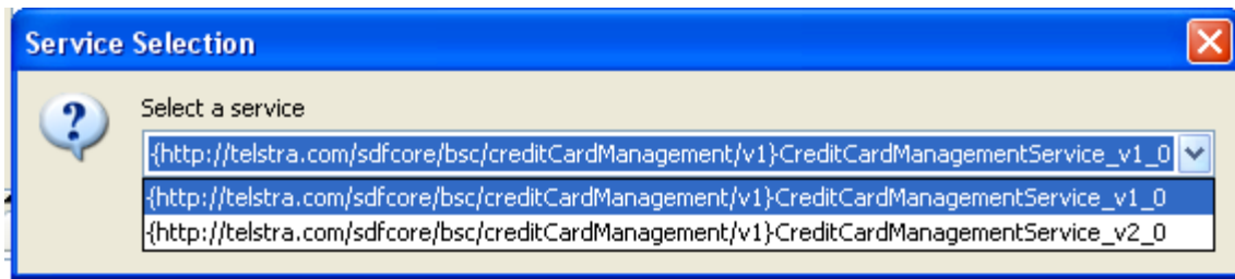
Figure 4.492: Service selection
