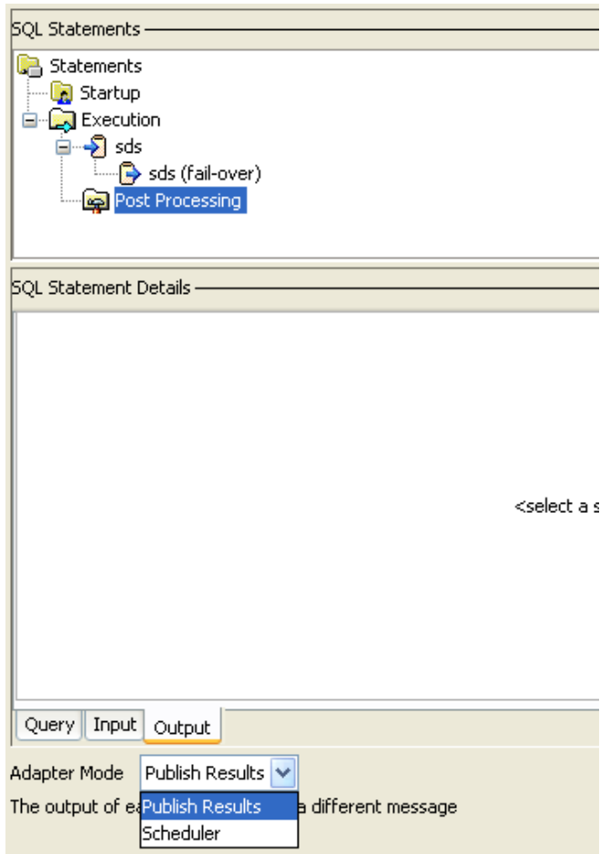
Figure 4.192: Adapter Mode
