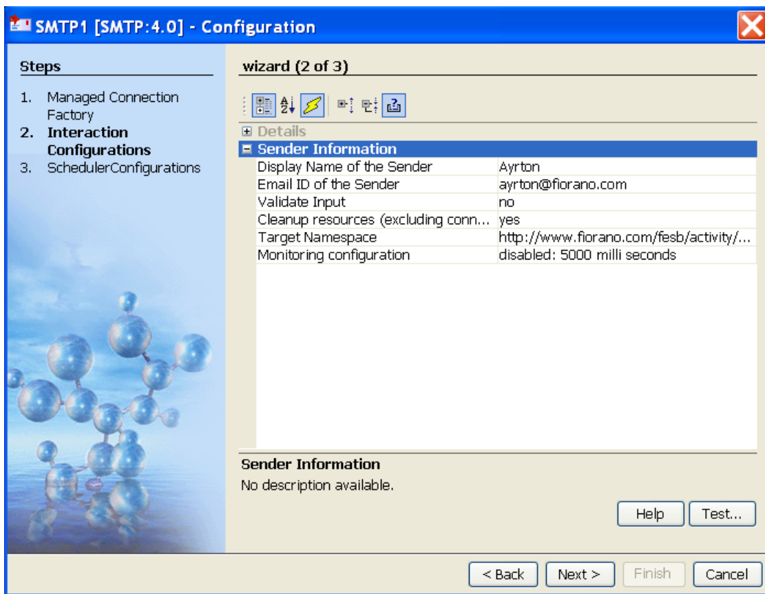
Figure 2: Interaction Configurations
