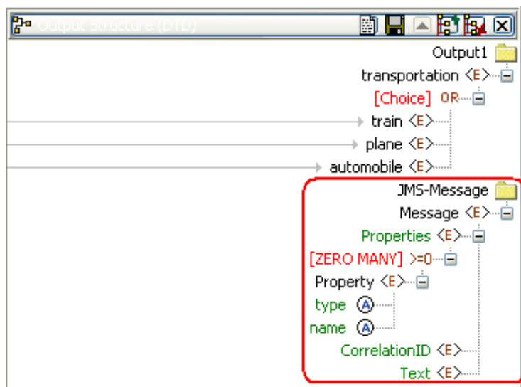
Figure 6: JMS-Message Structure loaded on output
