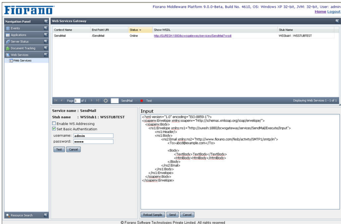
Figure 2.5.24: Web Services tab
