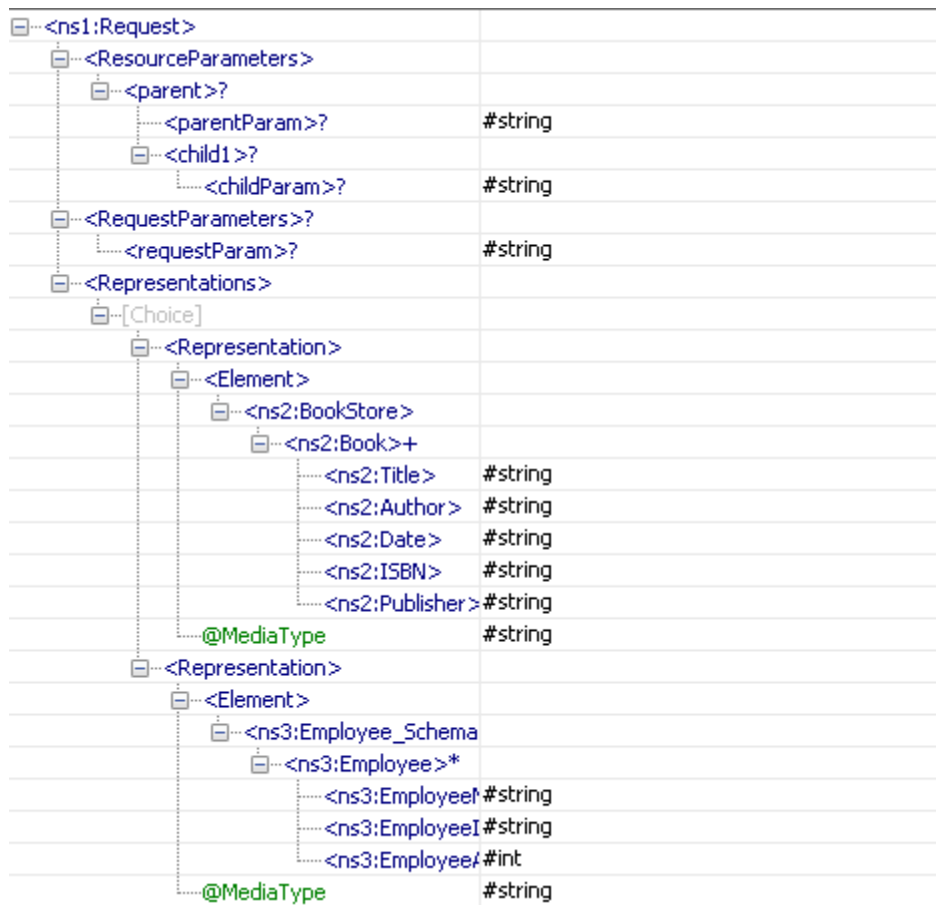
Figure 26: Schema of port parent__POST_Request
