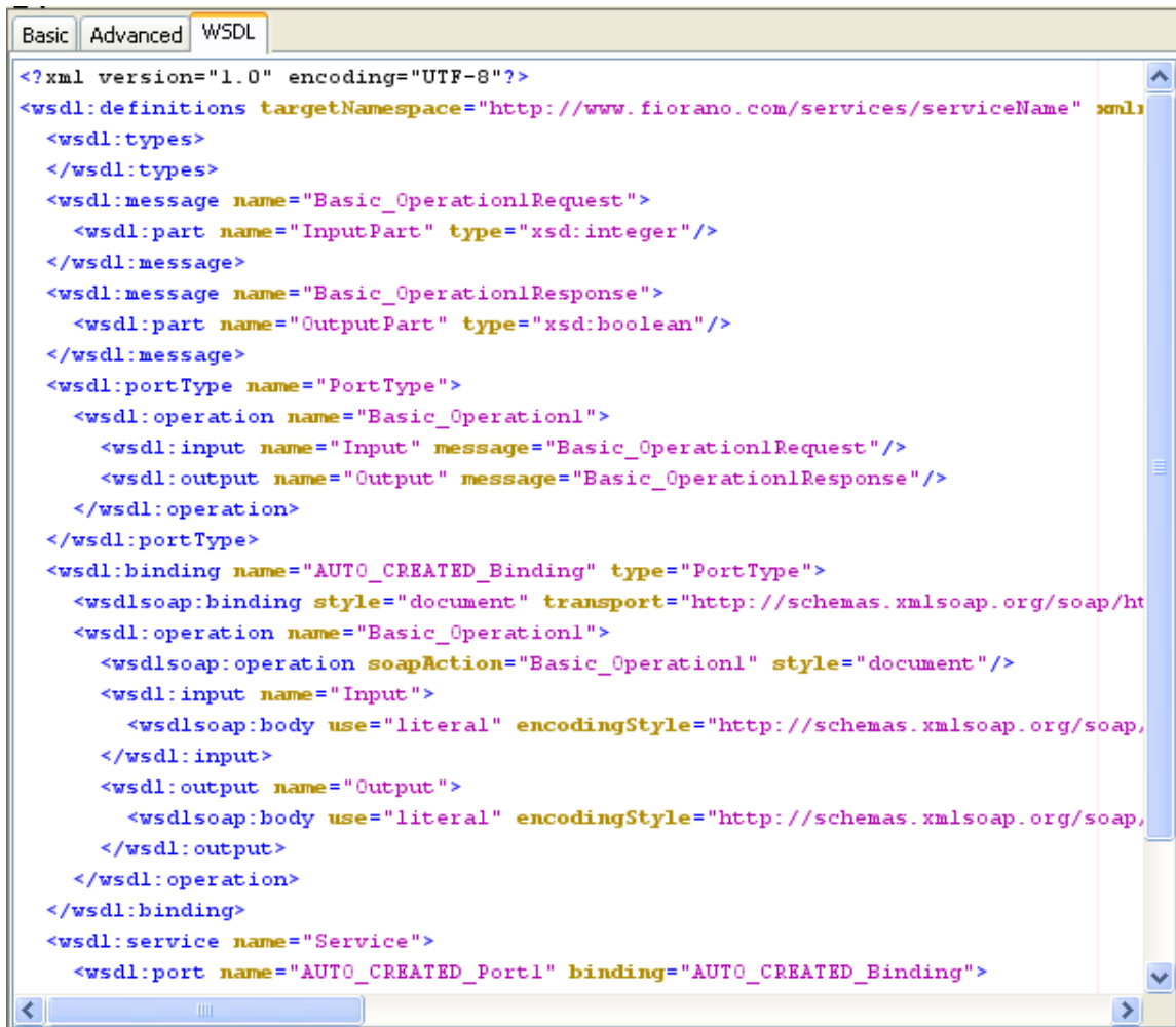
Figure 4.513: WSDL view
