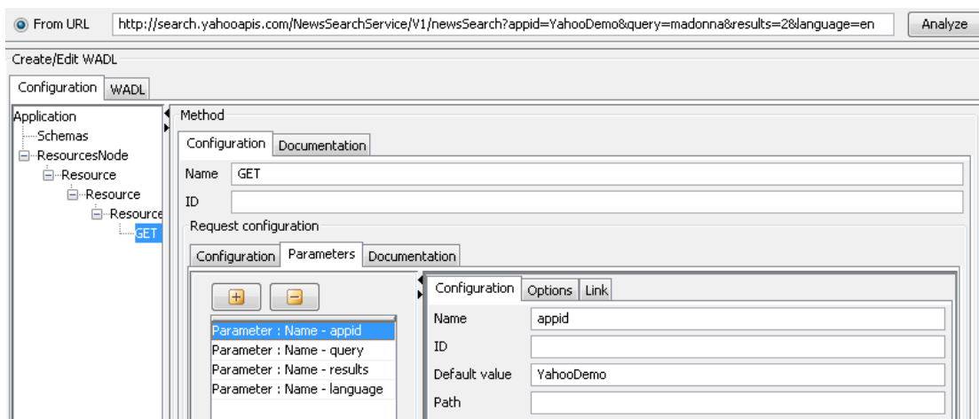
Figure 4: Analyzing URL
