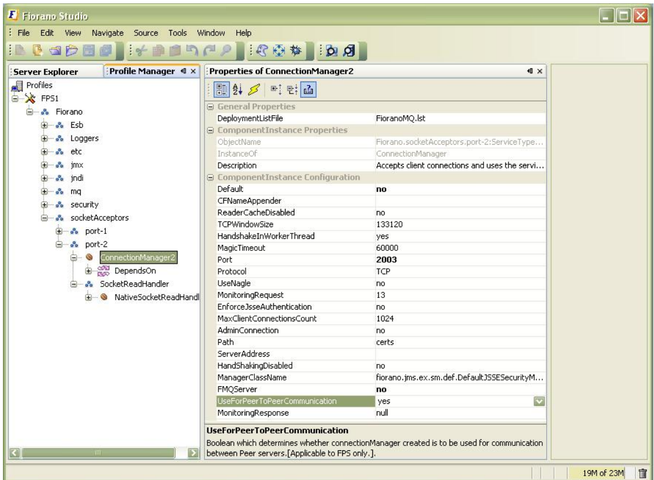
Figure 2.6.18: Adding Components
