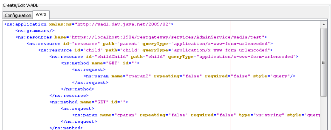
Figure 18: WADL view
