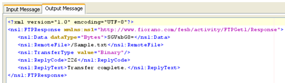
Figure 4.14: Sample output
