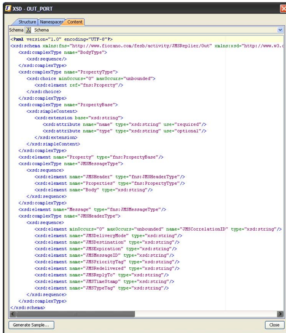
Figure 4.329: Output Schema
