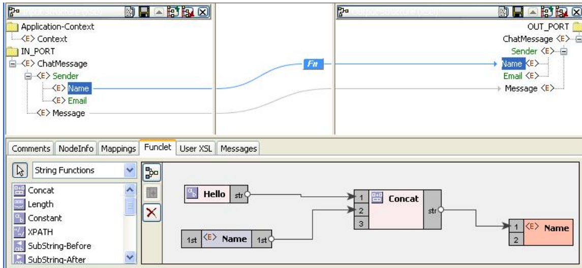
Figure 14: Mapping used
