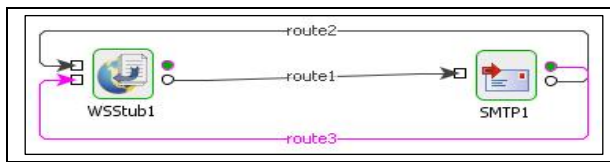
Figure 4.522: Scenario demonstration
