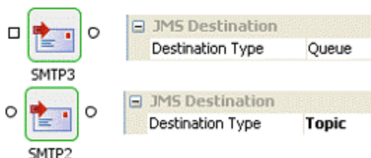
Figure 10: Input port as queue and as topic
