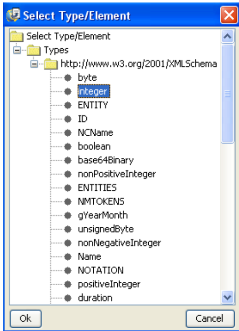
Figure 4.496: Type/Element Selection
