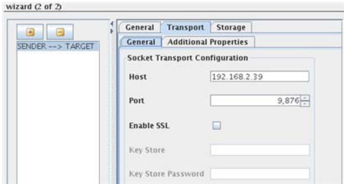
Figure 4: Transport Configuration
