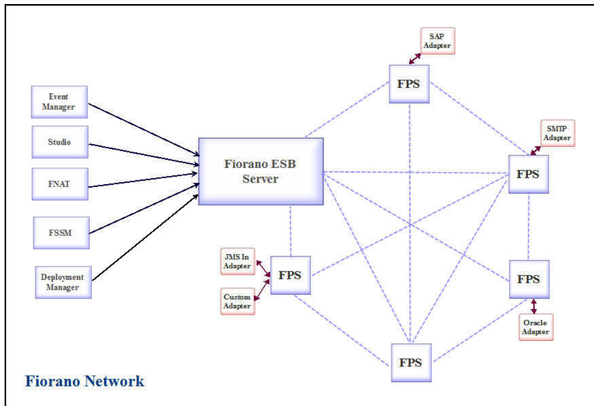
Figure 2.3.1: Fiorano Network
