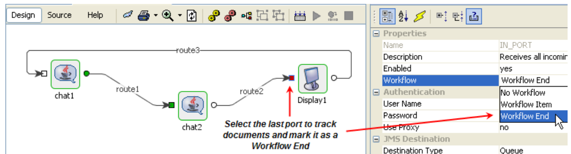
Figure 5.7.2: Workflow End
