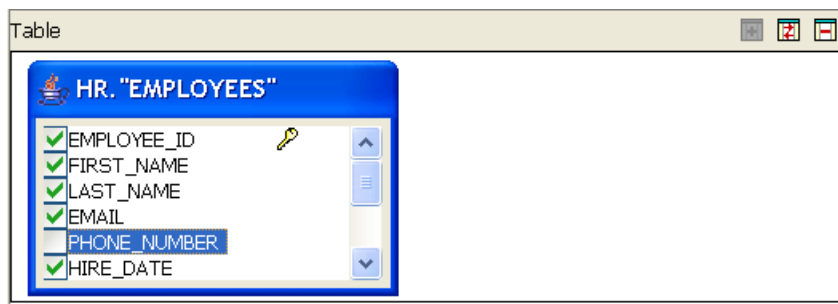
Figure 8: Ignoring column for insertion
