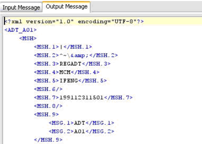
Figure 4.402: Response Generated
