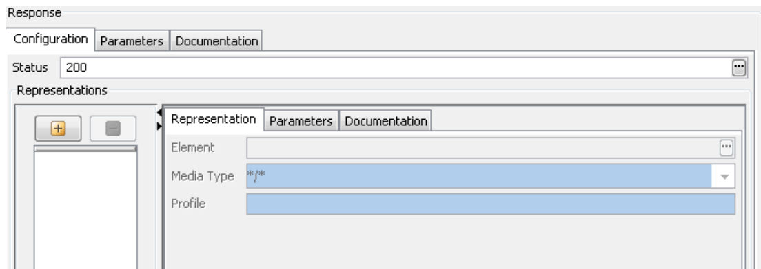
Figure 10: Response configuration
