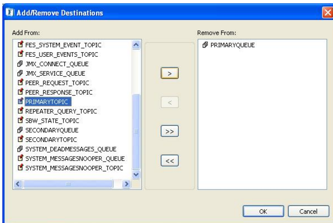
Figure 10: Add/Remove destinations
