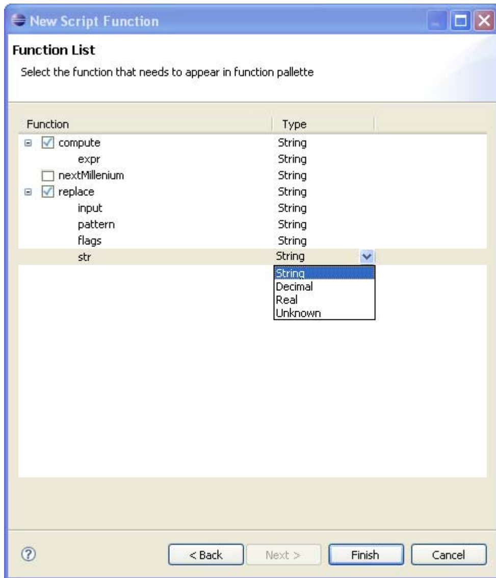
Figure 10.8.3 Function Page
