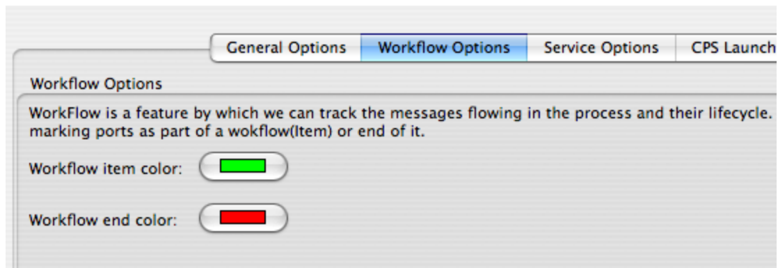
Figure 12.2.2: Workflow options
