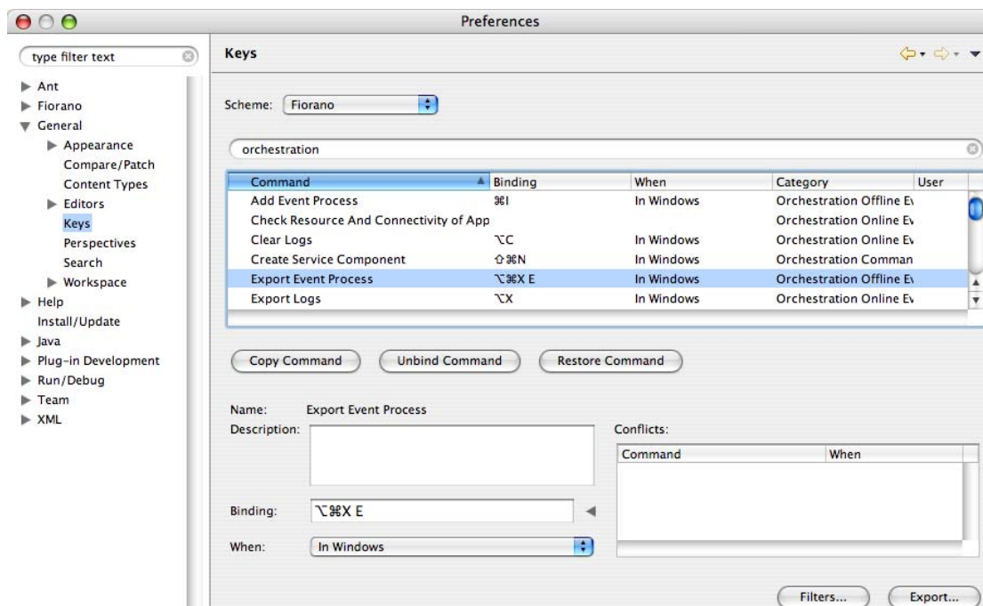
Figure 12.4.1: Key-binding preferences
