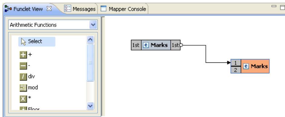
Figure 10.2.4: Funclet View
