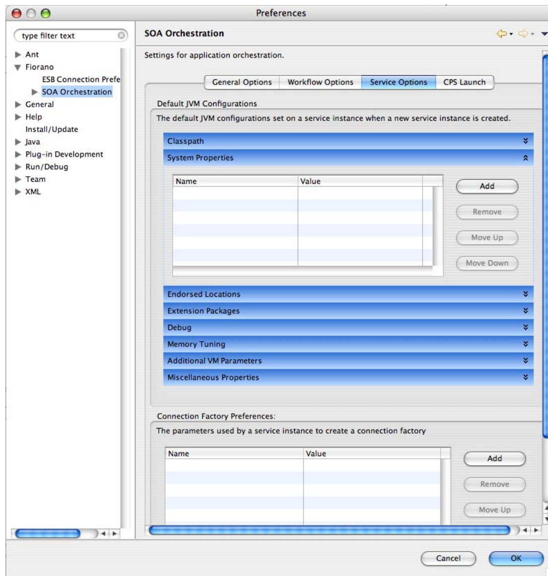
Figure 12.2.3: Service options
