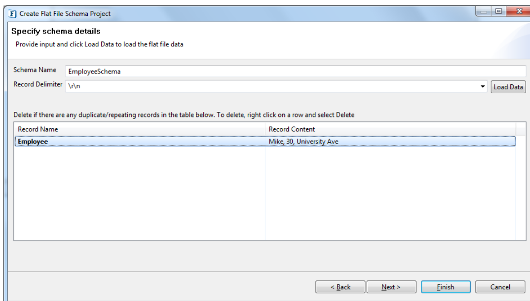
Figure 19.12: Configuring Records
