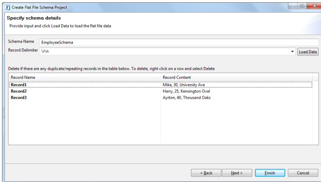
Figure 19.11: Schema configuration
