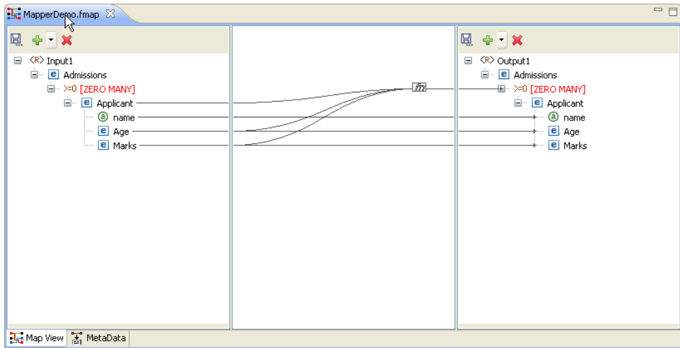
Figure 10.2.3: Map View
