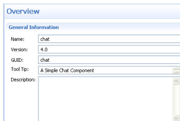
Figure 8.1.4: General Information
