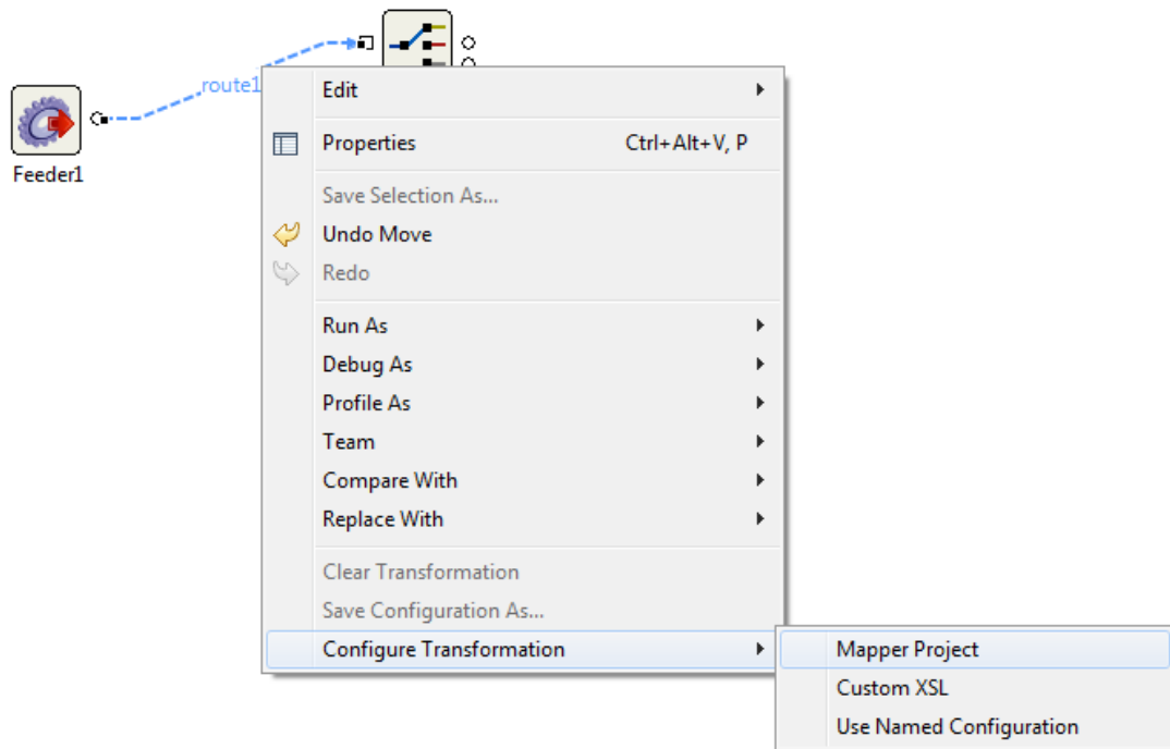
Figure 5.8.1: Route Transformation
