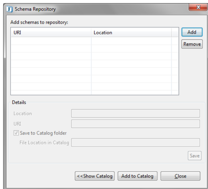
Figure 13.1.1: Schema Repository
