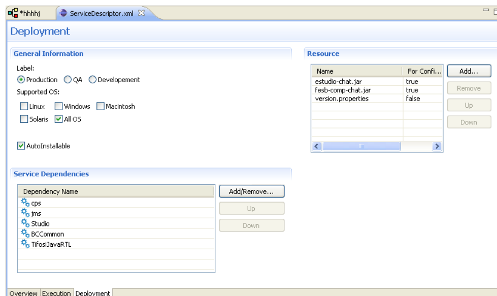
Figure 8.1.11: Deployment page
