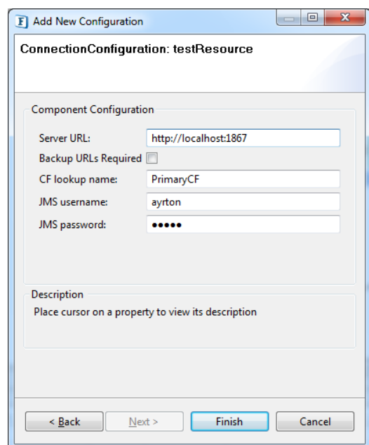
Figure 9: Connection Configuration
