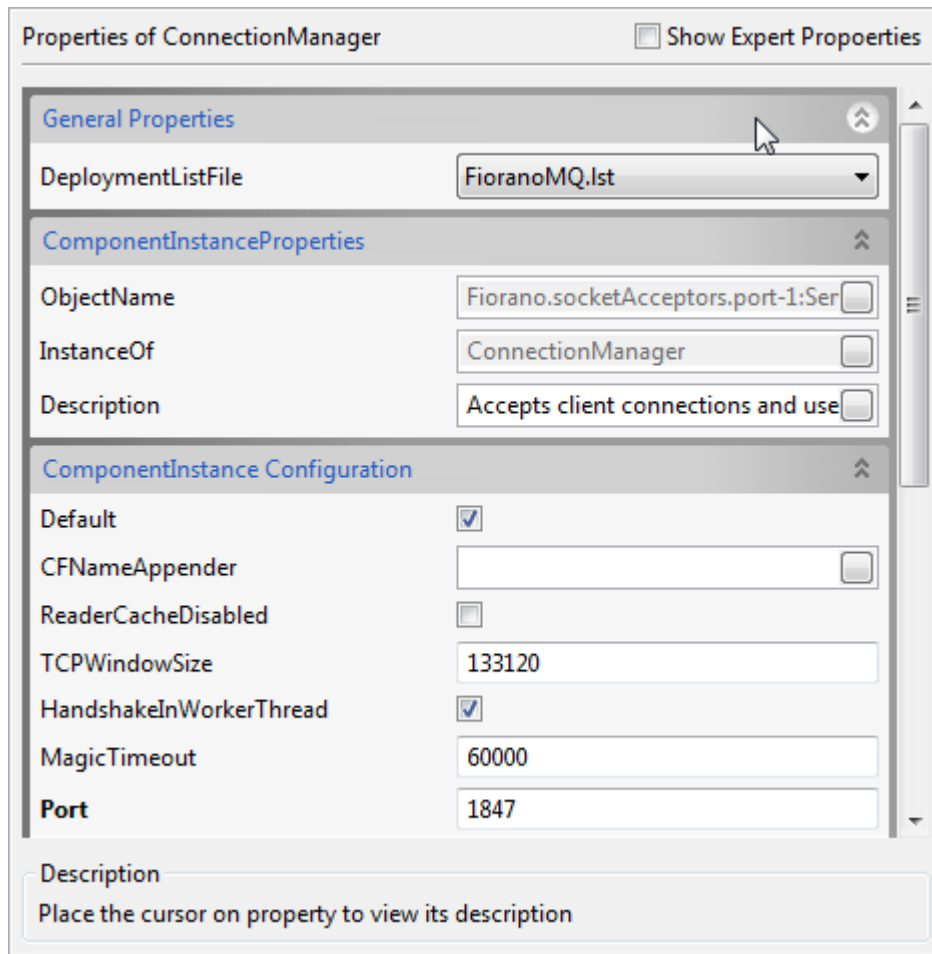
Figure 4: Properties UI
