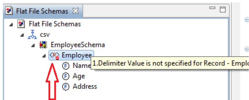
Figure 19.18: Schema Errors
