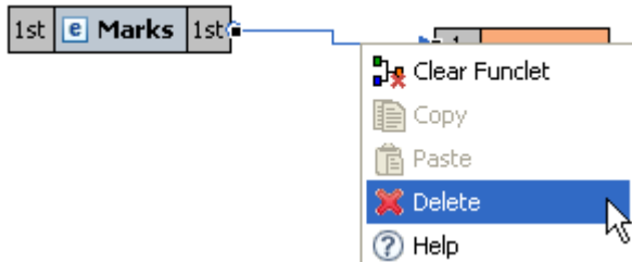
Figure 10.4.35: Deleting link
