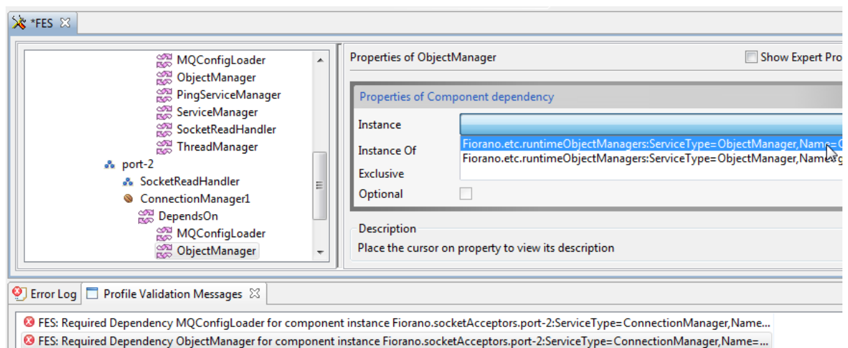
Figure 9: Resolving dependencies
