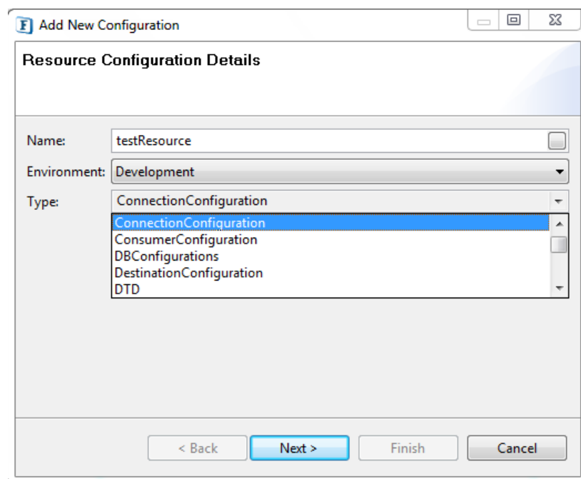
Figure 8: Resource Configuration
