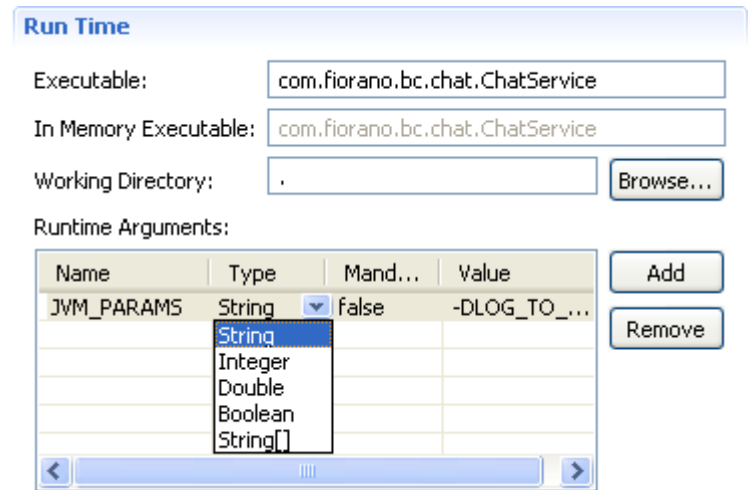
Figure 8.1.10: Runtime section
