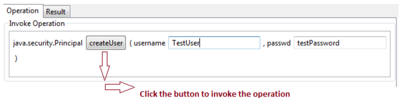
Figure 14: Operation signature
