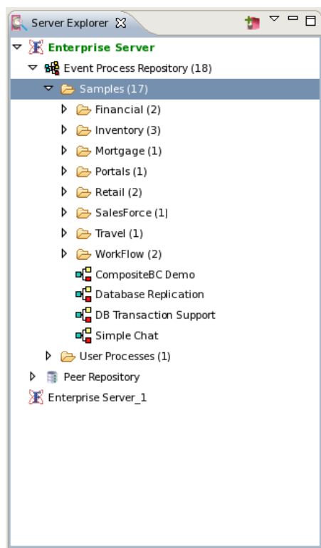
Figure 3.1.3: Server Explorer
