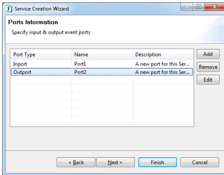
Figure 9.1.4: Ports Information
