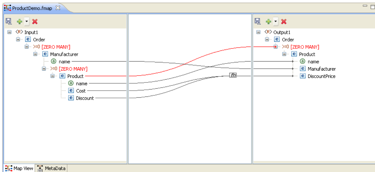
Figure 10.5.6: Name-to-name Mapping
