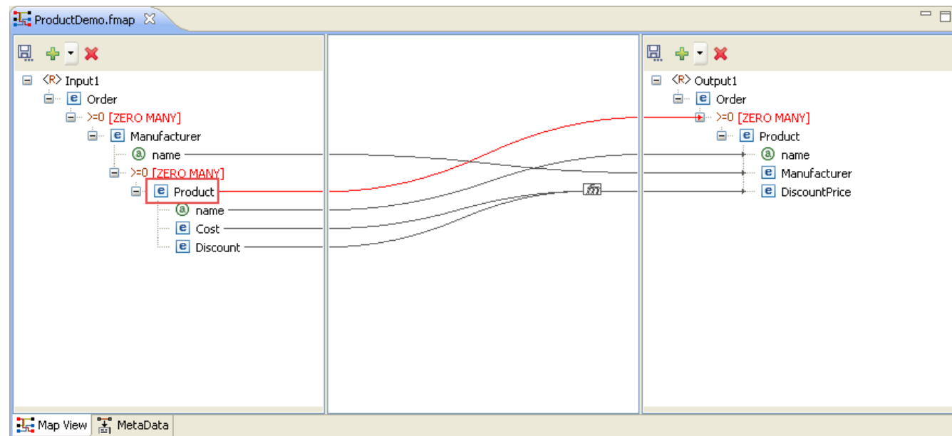
Figure 10.5.7: For-Each Mapping
