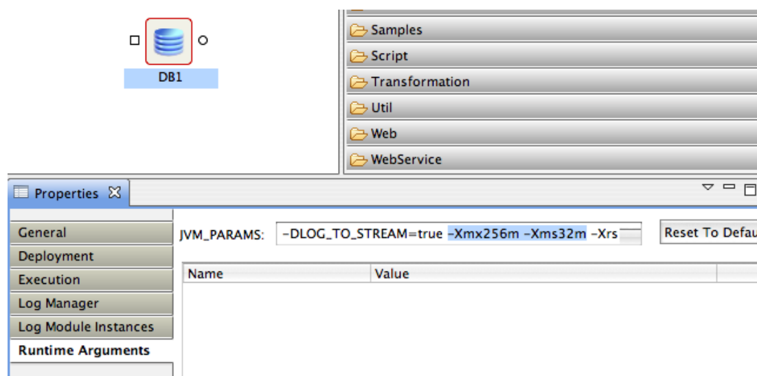
Figure 12.2.5: Runtime Arguments
