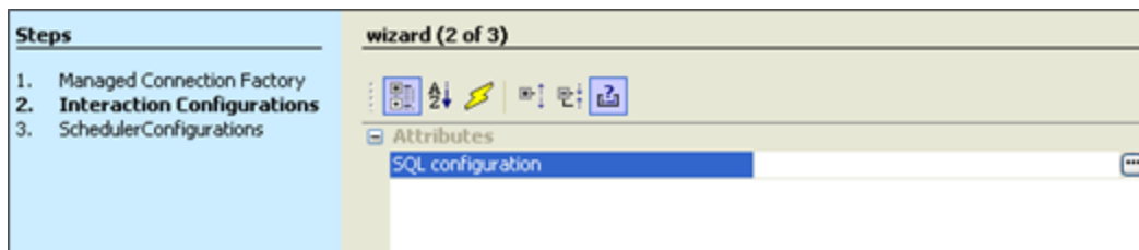
Figure 4.105: Interaction Configurations
