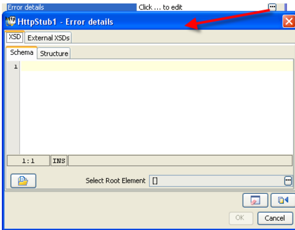
Figure 6: Error Details
