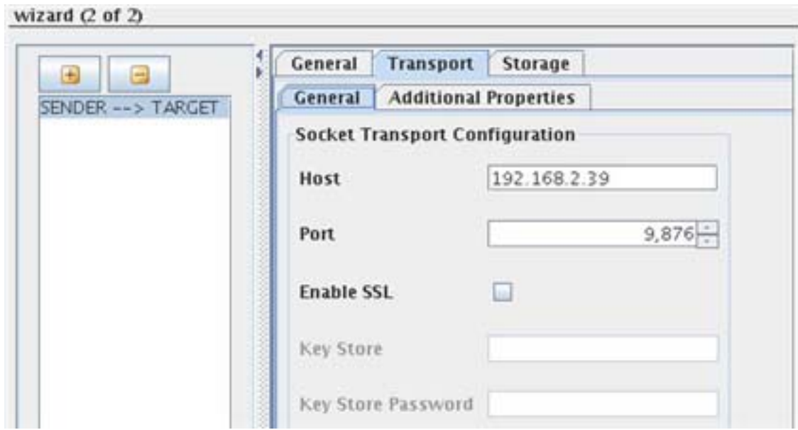
Figure 2: Transport Configuration
