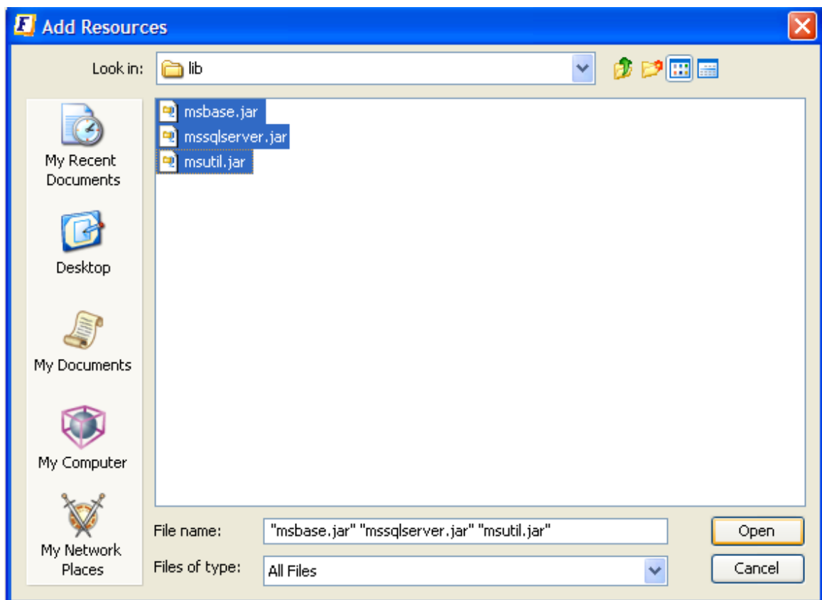
Figure 3.3.16: Add Resources
