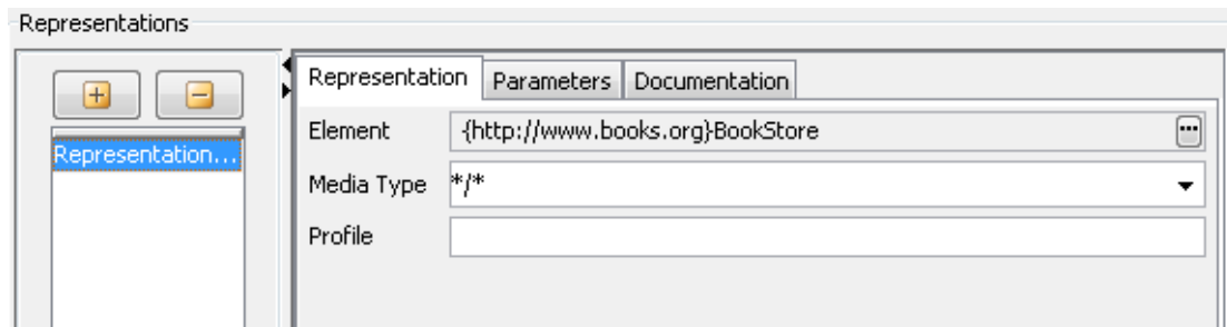
Figure 12: Representation Configuration
