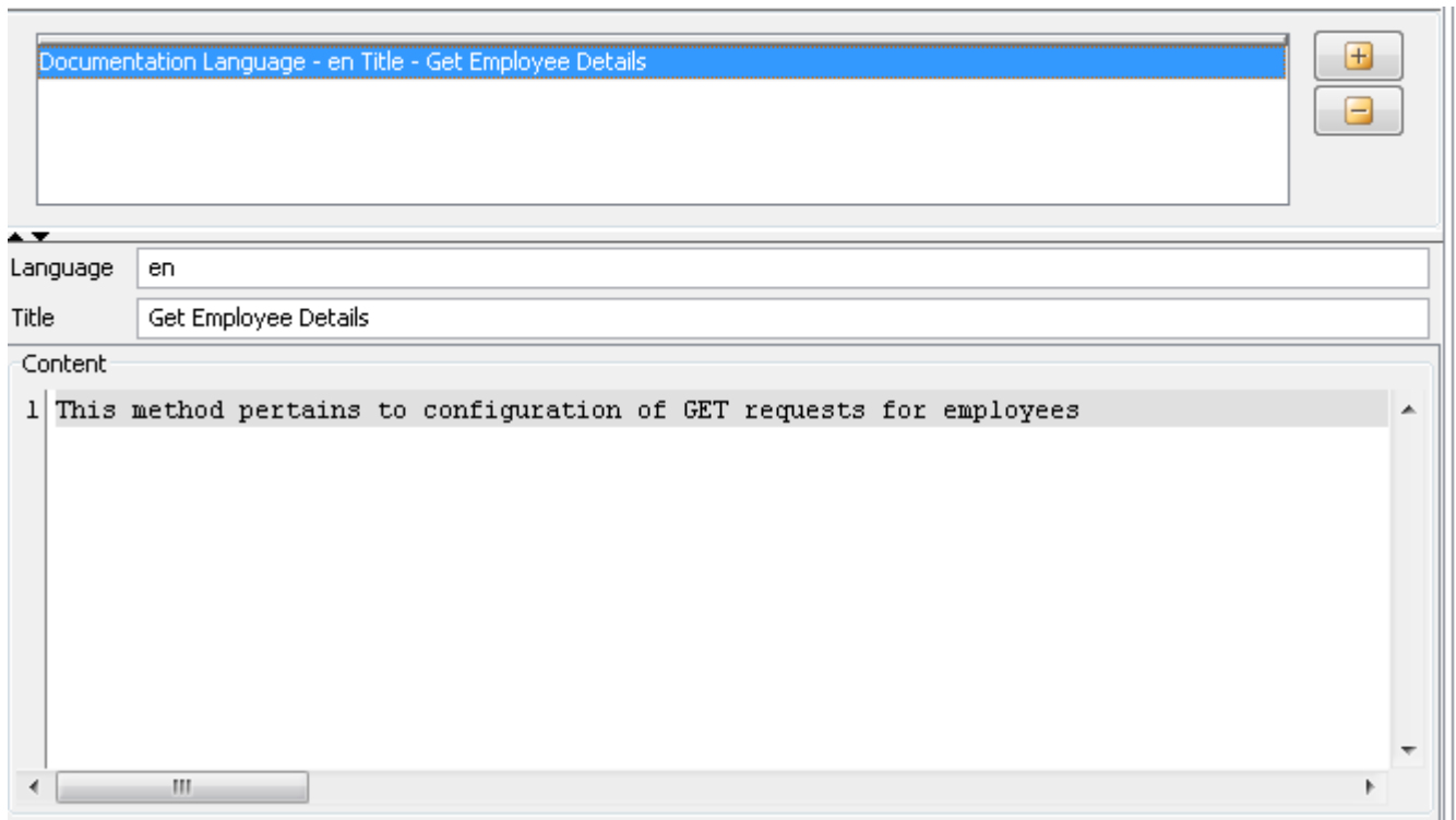
Figure 16: Configuring documentation.
