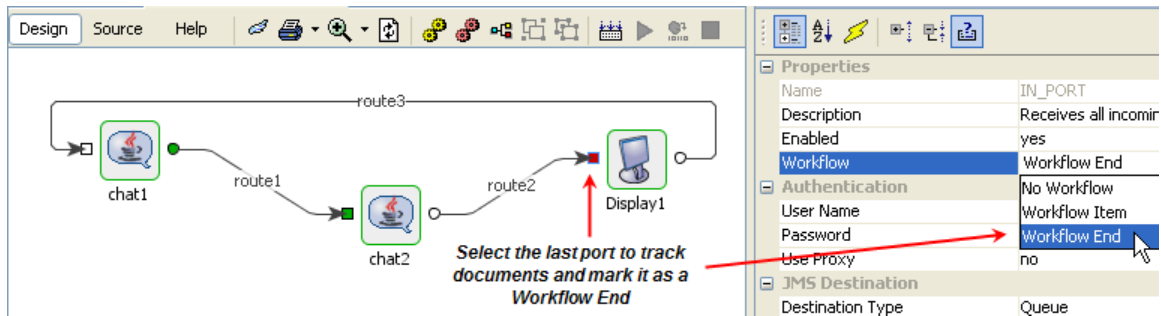
Figure 5.7.2: Workflow End
