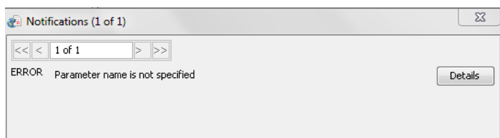
Figure 17: Error Notifications
