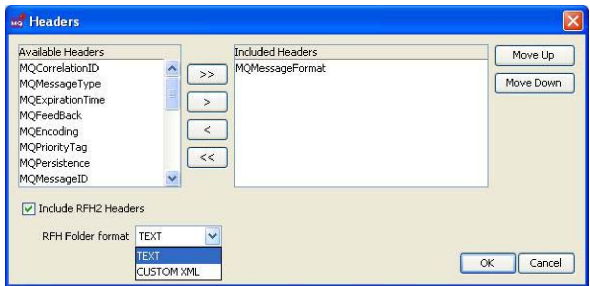
Figure 17: Headers editor
