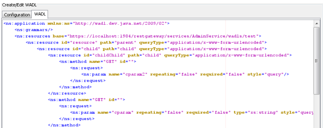
Figure 18: WADL view
