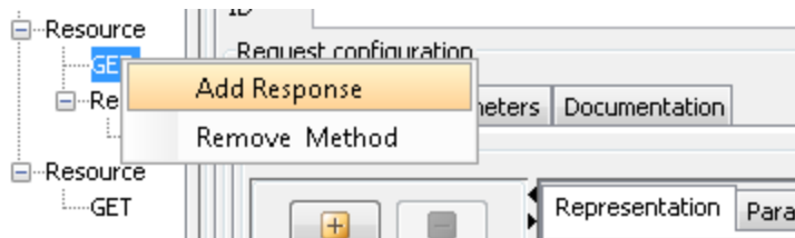
Figure 9: Adding Response
