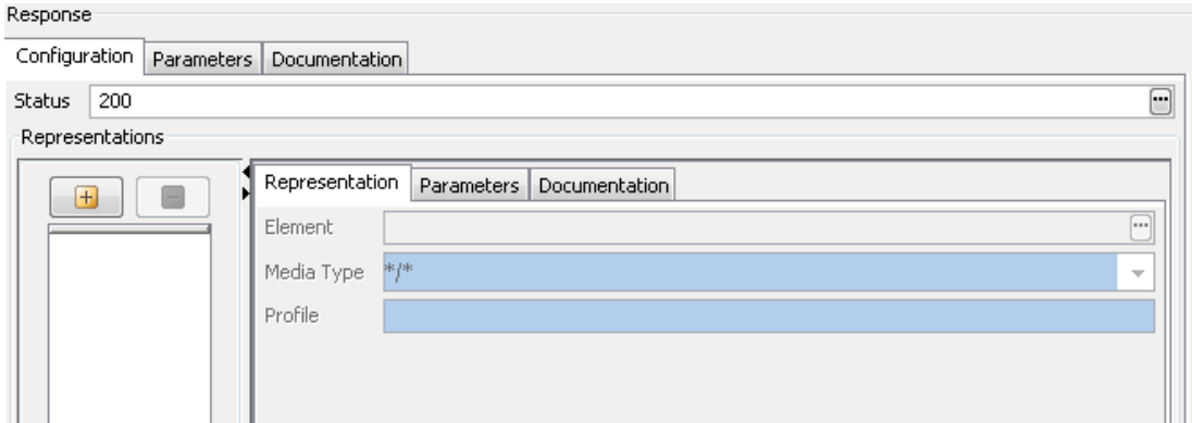
Figure 10: Response configuration
