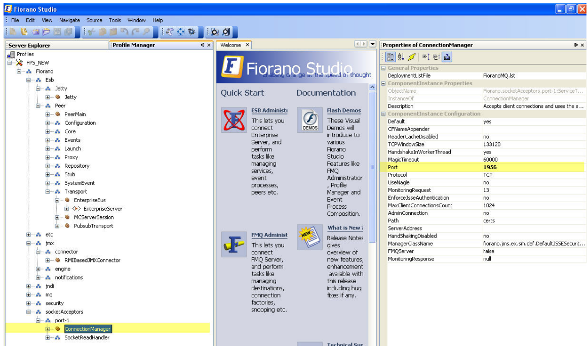
Figure 2.4.13: ConnectionManager
