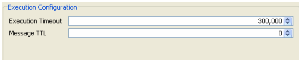
Figure 23: Execution Configuration
