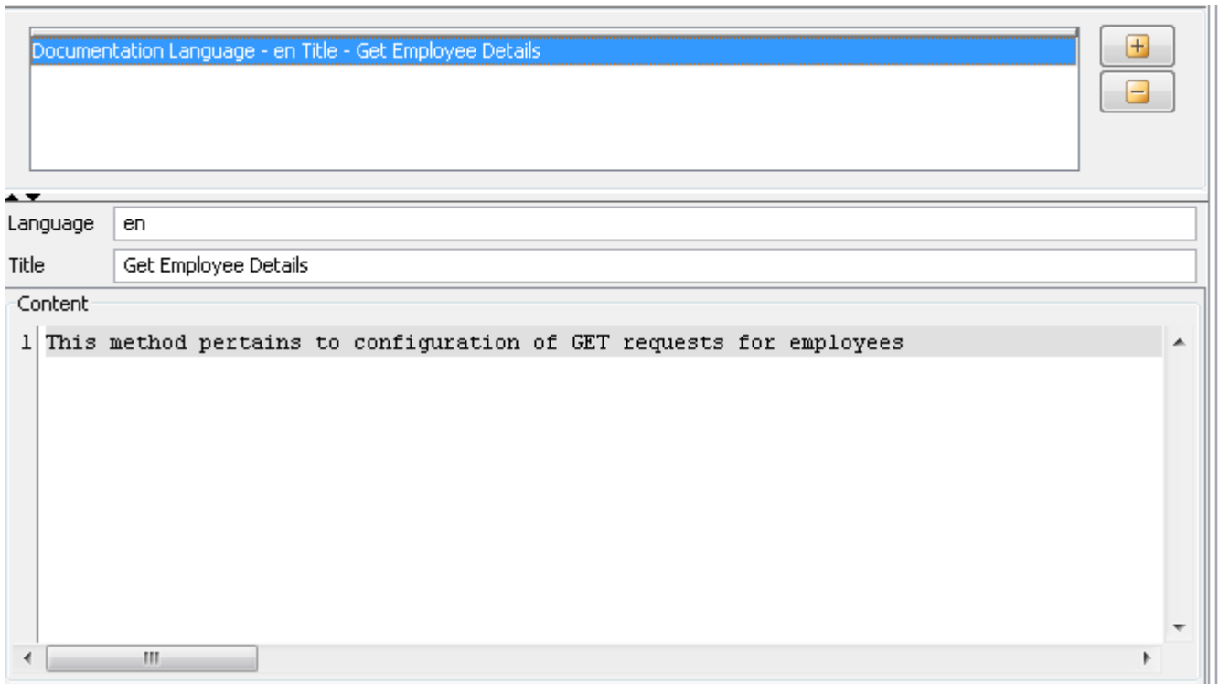
Figure 16: Configuring documenatation.
