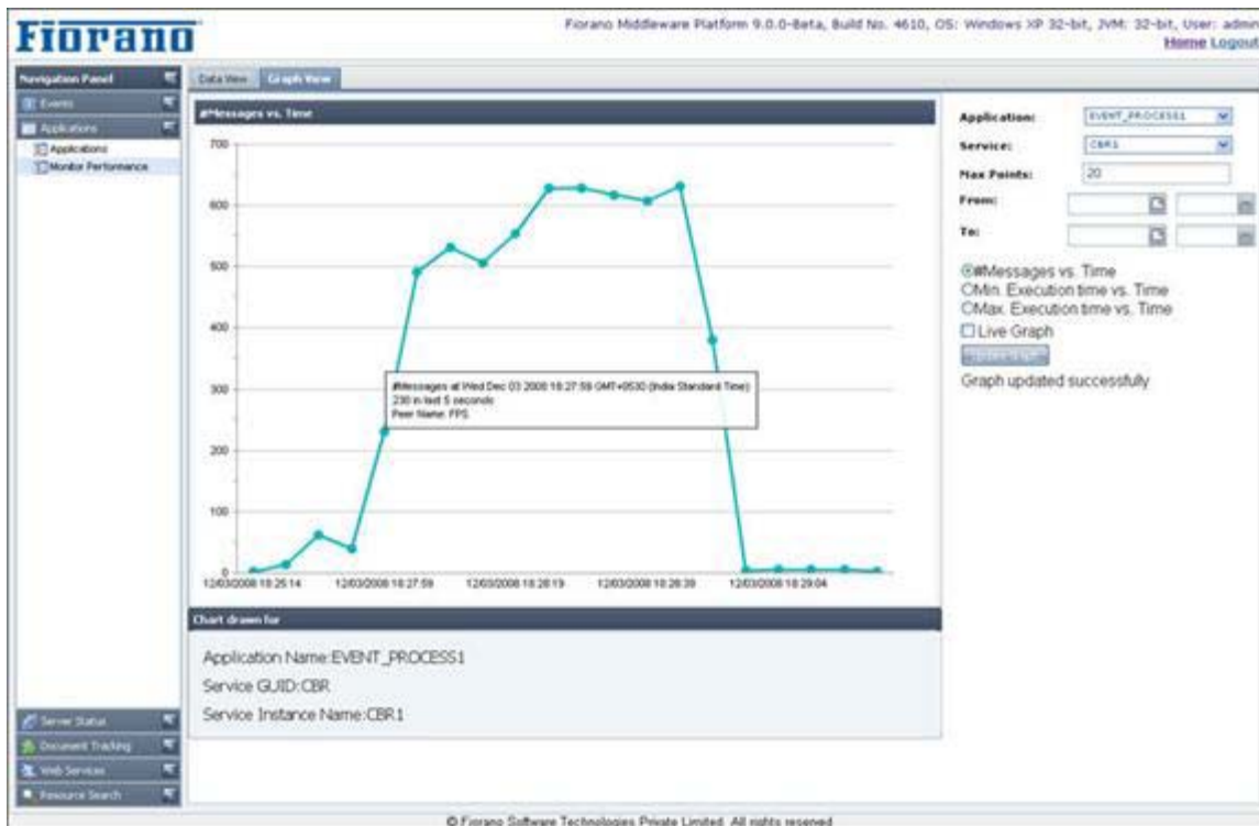
Figure 2.5.15: Graph View
