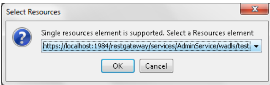
Figure 3: Resources selection
