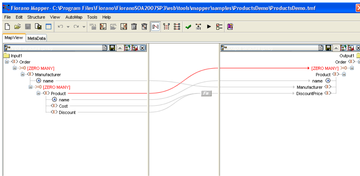
Figure 9.5.6: Name-to-name Mapping
