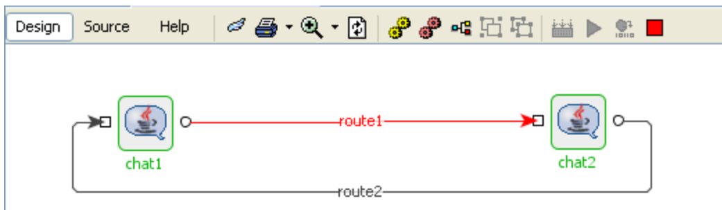
Figure 5.5.7: Route Color
