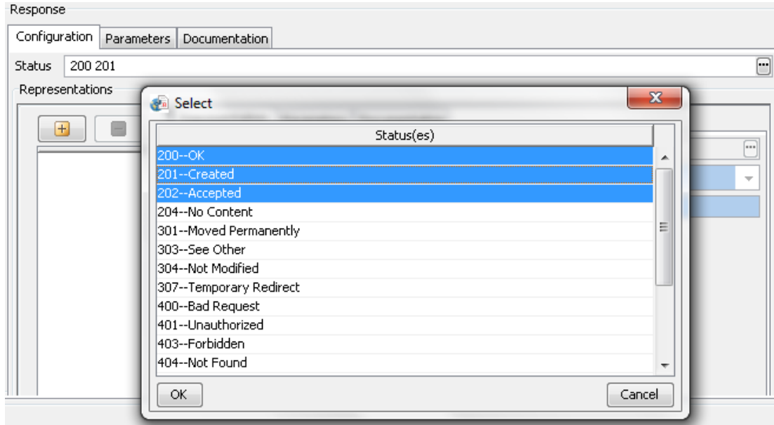
Figure 11: Configuring status
