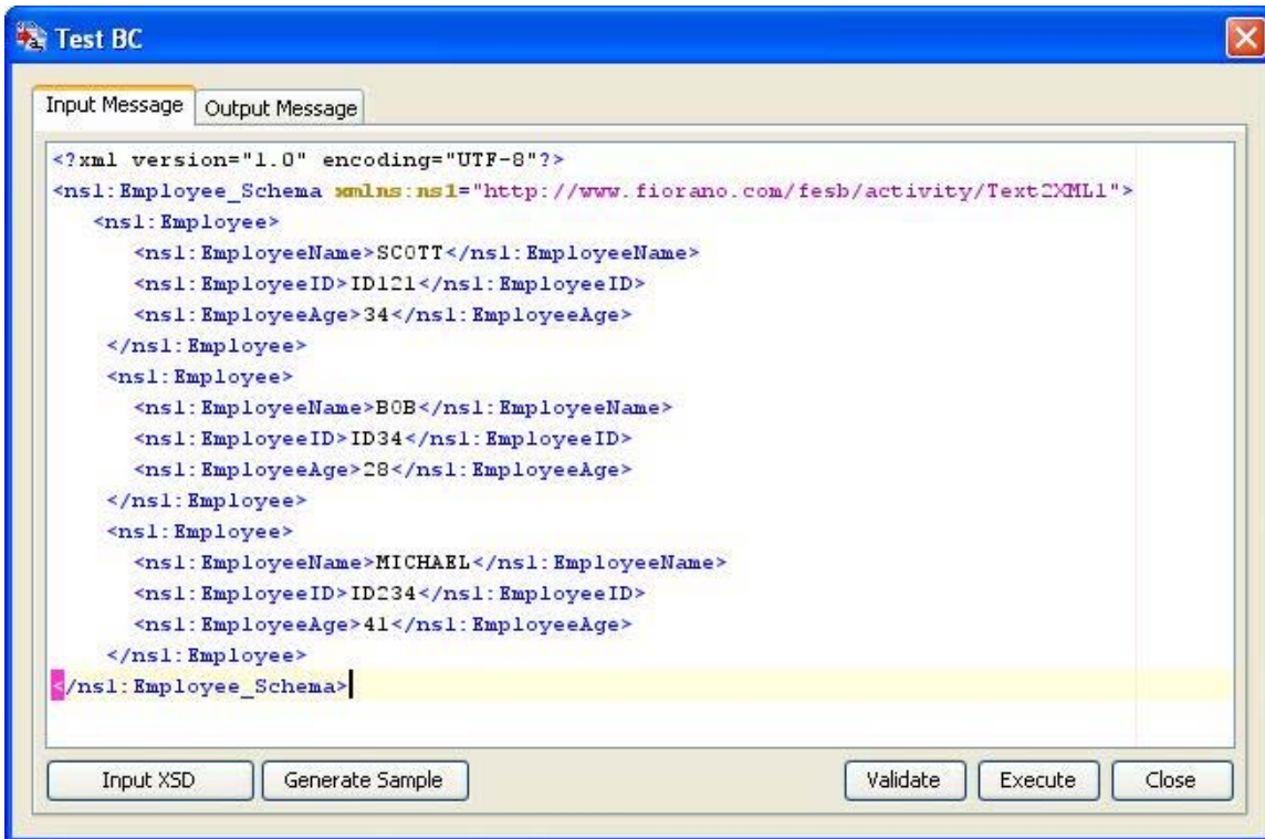
Figure 5: Sample Input
