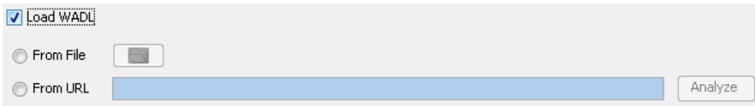
Figure 2: Loading WADL
