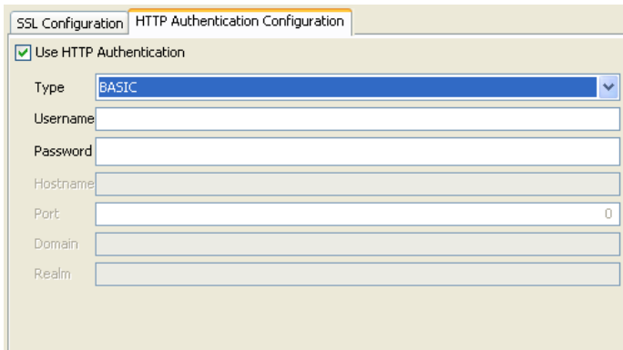
Figure 20: HTTP Authentication
