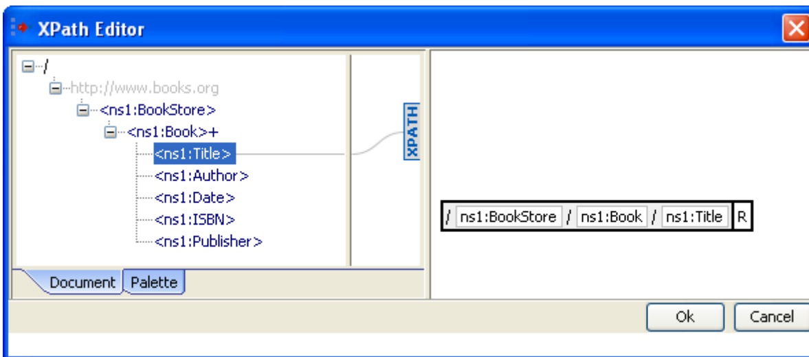
Figure 34: XPath Editor
