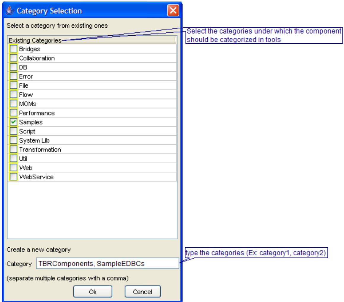
Figure 3.6.6: Specifying categories
