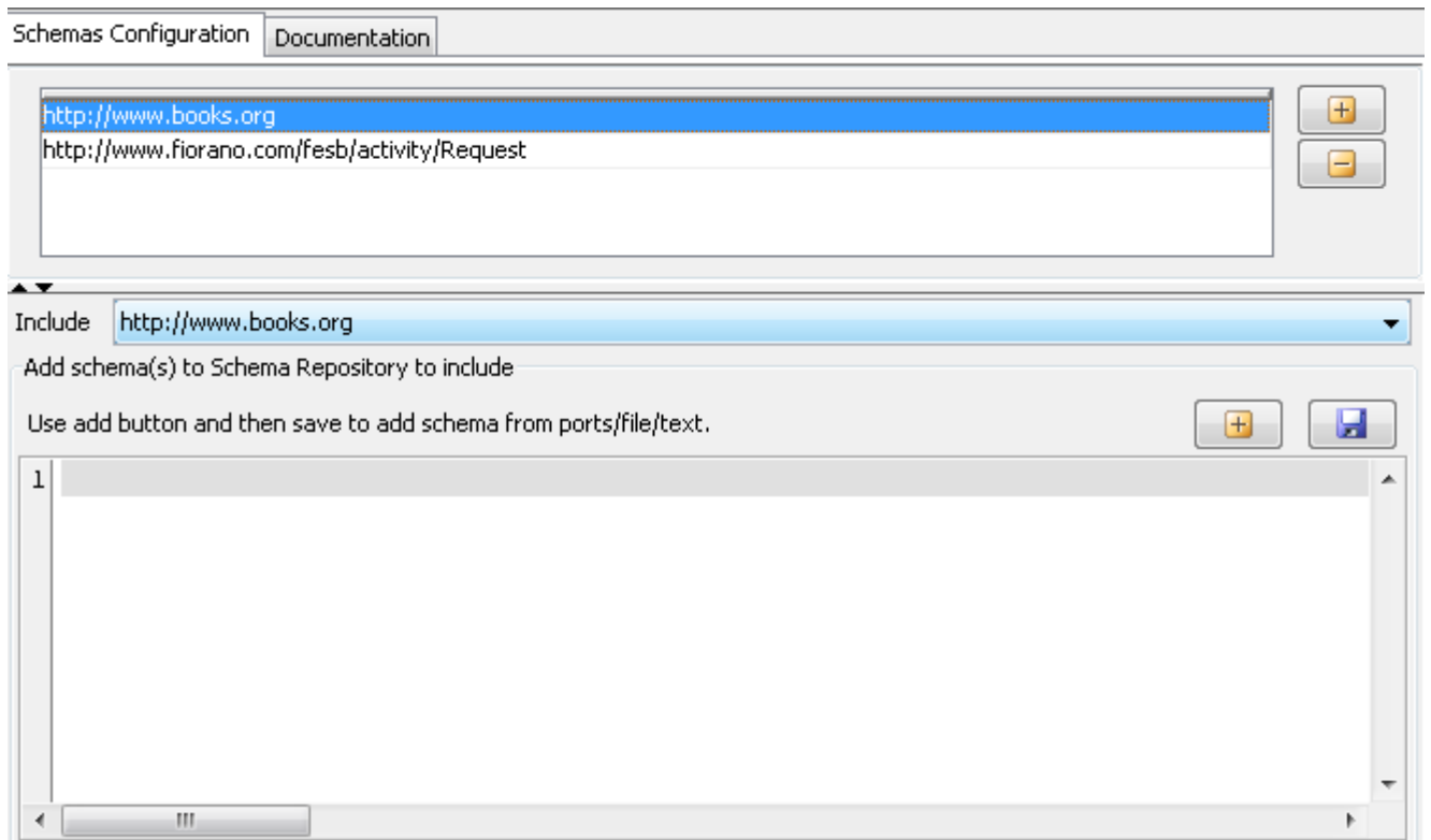
Figure 5: Schemas Configuration
