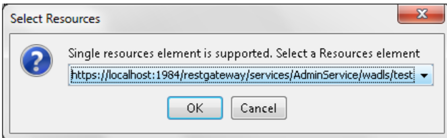
Figure 3: Resources selection
