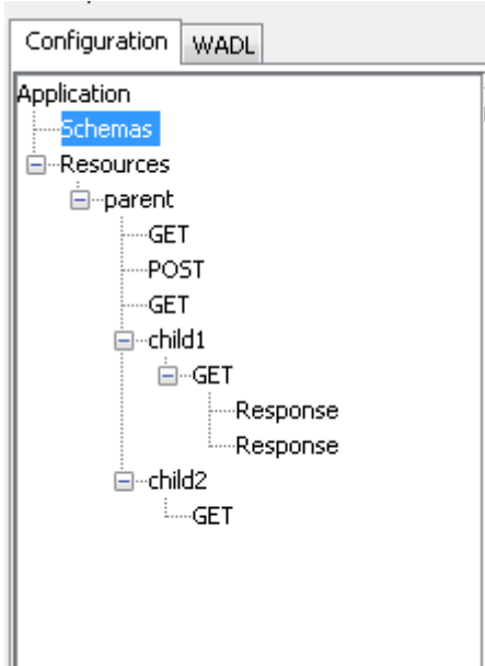
Figure 23: Sample Configuration
