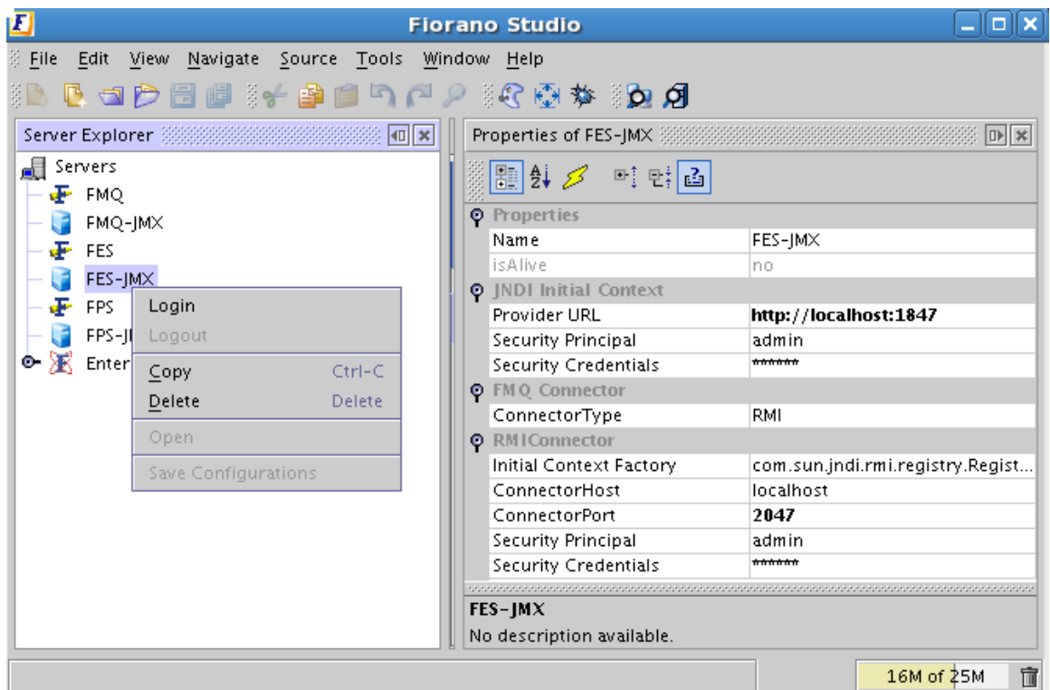
Figure 2.3.6: FES-JMX Server
