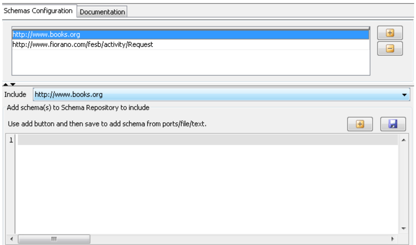
Figure 5: Schemas Configuration
