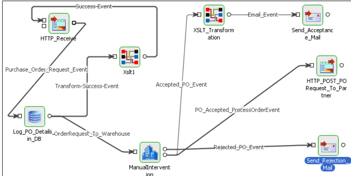
Figure 33: Order Entry
