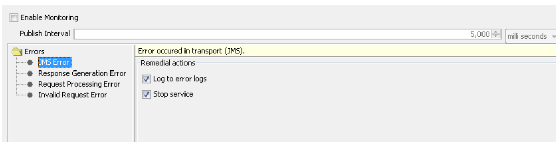
Figure 21: Additional Configuration
