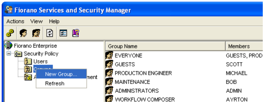
Figure 2.3.19: Adding Group
