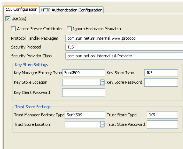
Figure 19: SSL Configuration
