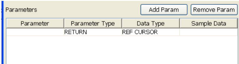
Figure 8: Populated Parameters
