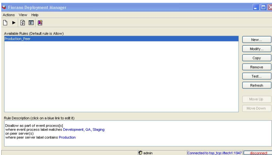
Figure 8.5.2: Sample Rule
