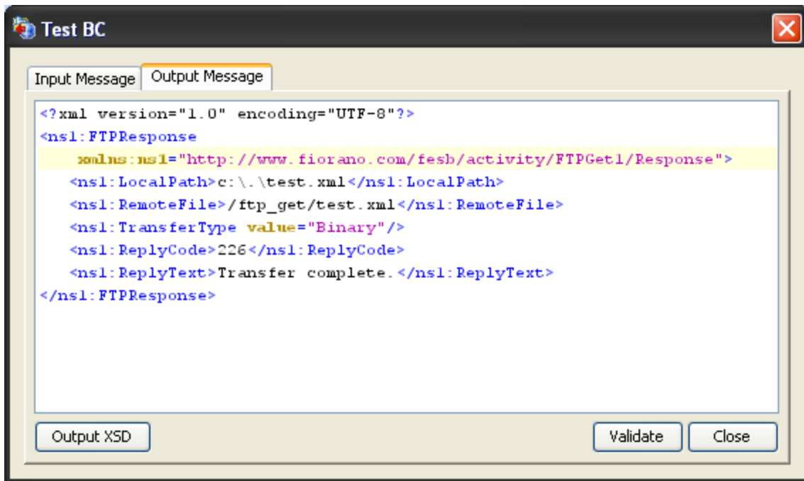
Figure 4.21: Sample response
