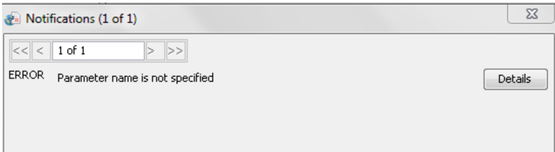
Figure 17: Error Notifications
