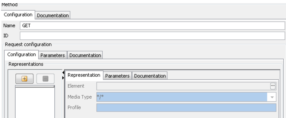
Figure 8: Method Configuration
