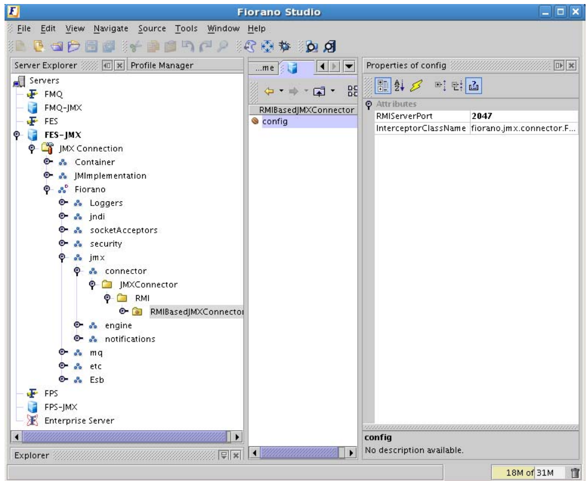
Figure 2.3.13: JMX Explorer
