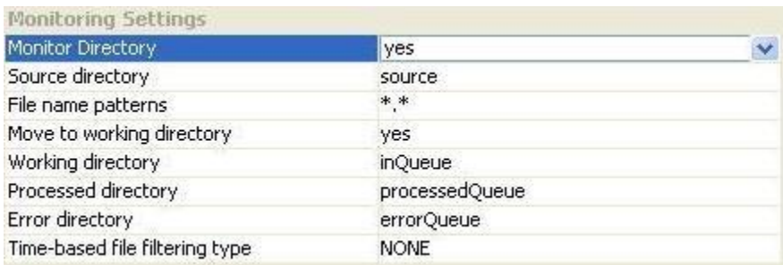
Figure 28: Monitoring Settings
