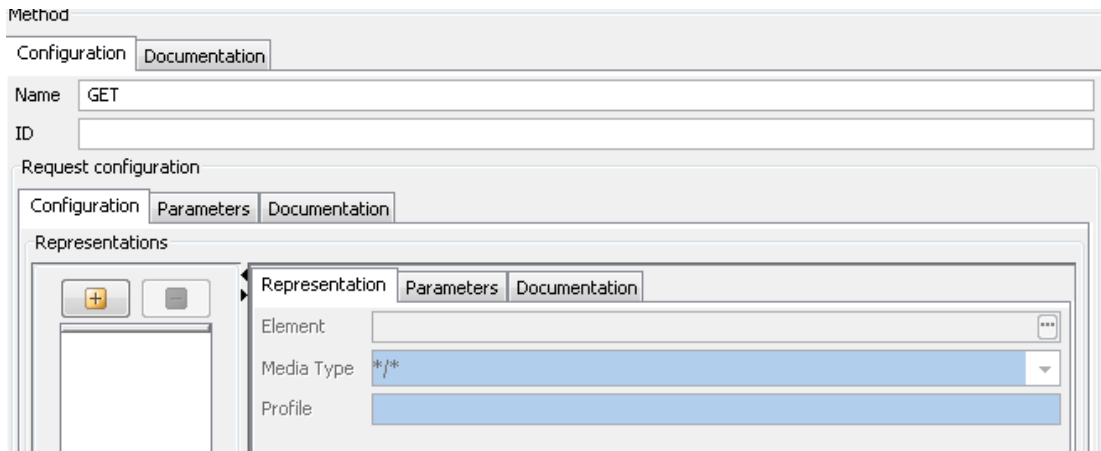
Figure 8: Method Configuration
