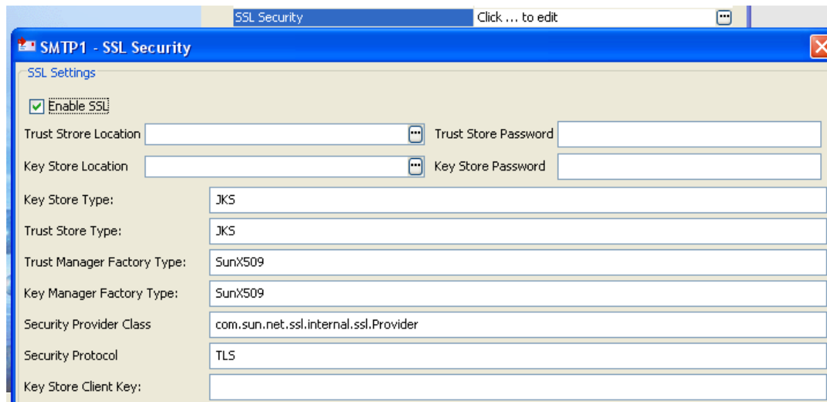
Figure 14: SSL configurations
