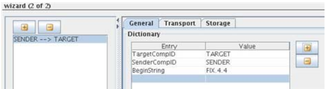
Figure 3: General Session Configuration
