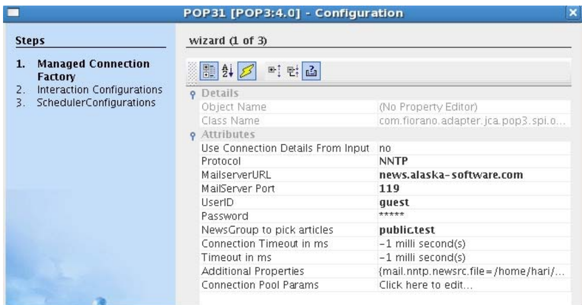
Figure 1: Managed Connection Panel of POP3
