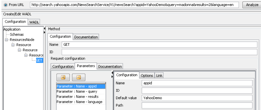
Figure 4: Analyzing URL
