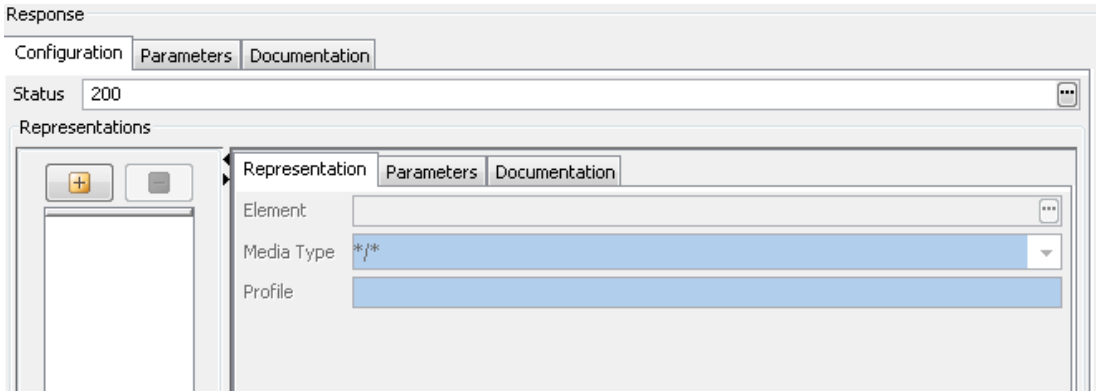
Figure 10: Response configuration
