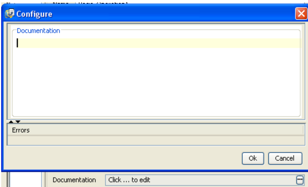
Figure 4.515: Documentation Panel
