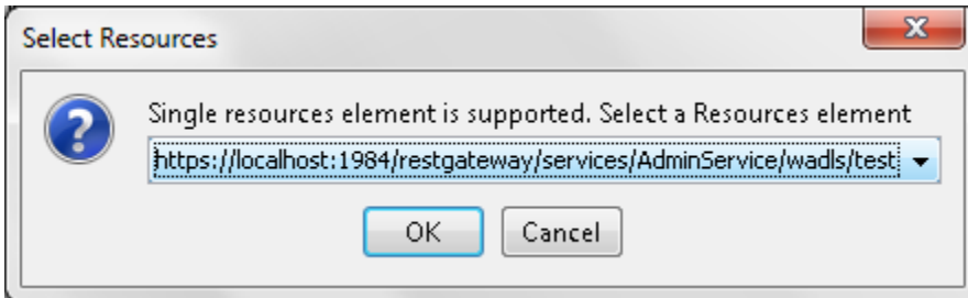
Figure 3: Resources selection
