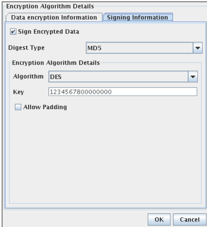
Figure 3: Digest type used and Encryption algorithm used for verifying digested data can be provided as given above.
