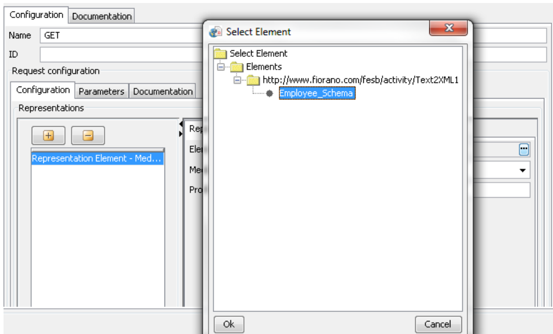
Figure 13: Configuring elements
