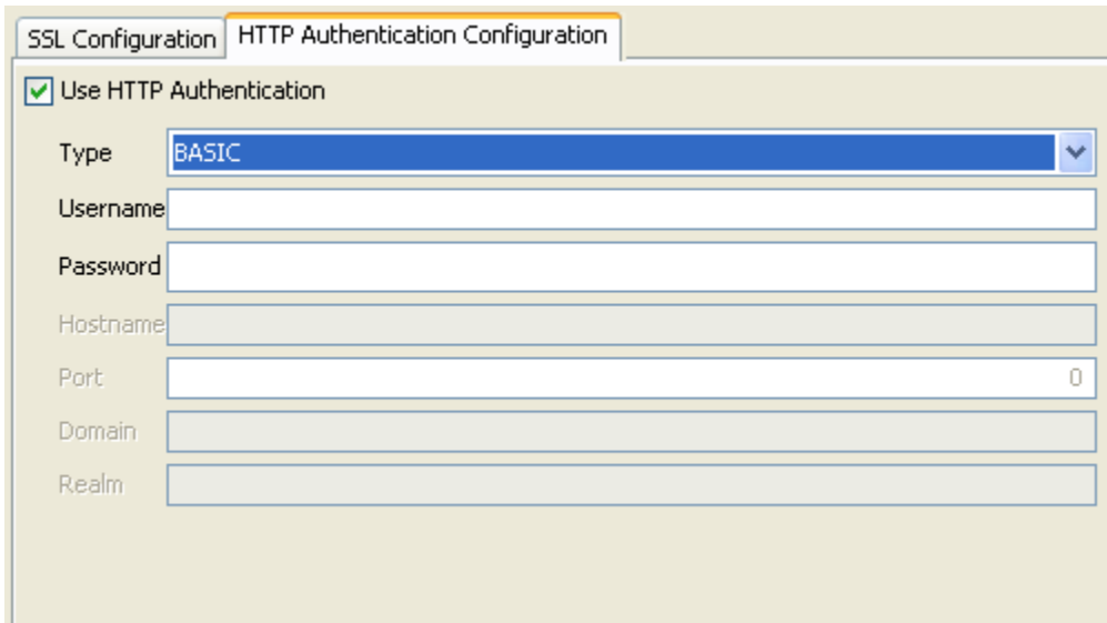
Figure 20: HTTP Authentication
