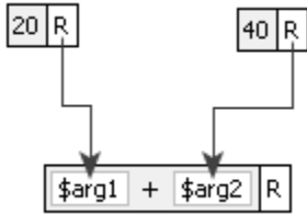
Figure 39: Add(+) operator
