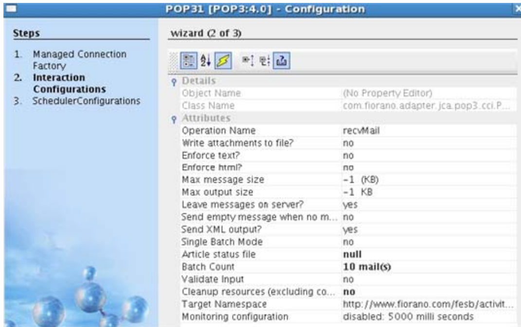
Figure 2: Interaction Configuration panel
