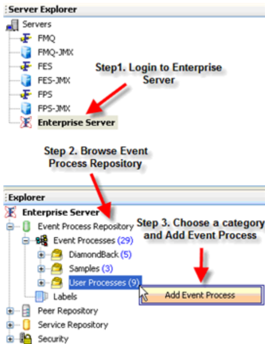
Figure 5.2.3: Creating an Event Process
