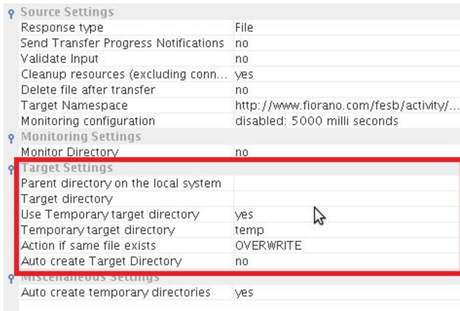
Figure 4.5: Interaction Configurations with response type – File
