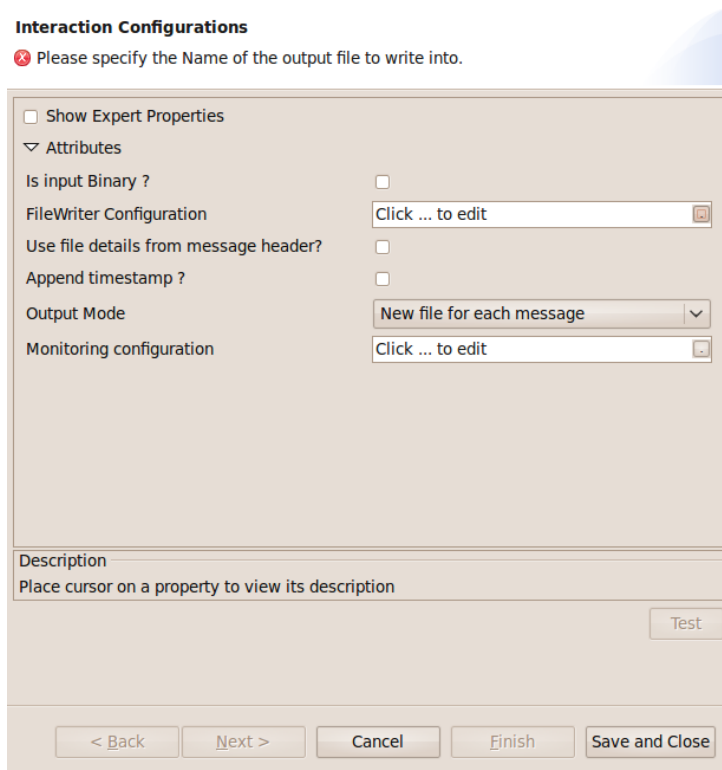
Figure: Modified Interaction Configurations panel
