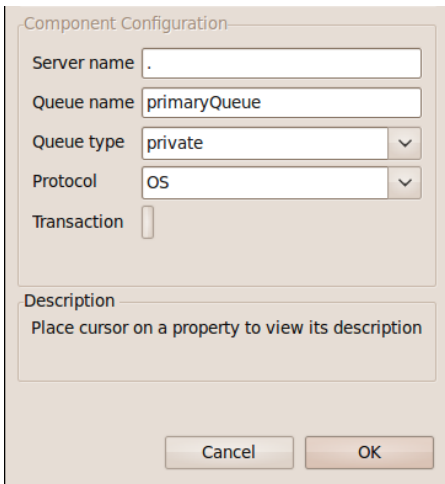
Figure: Connection Configuration
