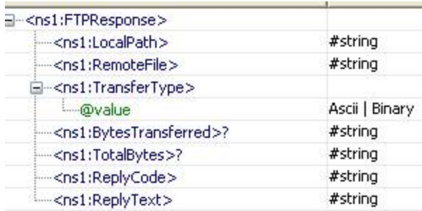
Figure 8: Output schema structure for the response type – File
