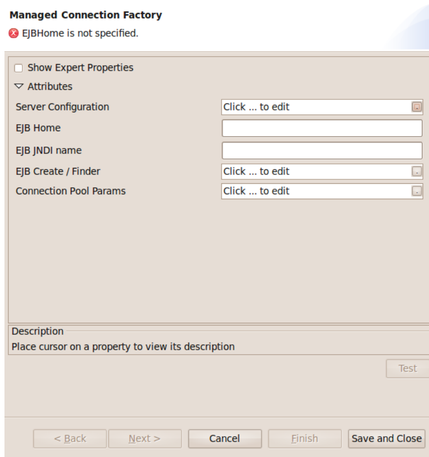
Figure: Modified Managed Connection Factory
