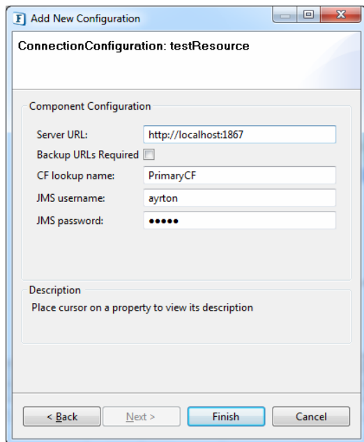
Figure 9: Connection Configuration
