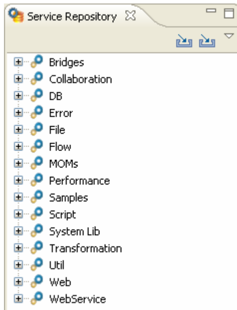
Figure 2.3.1: Service repository
