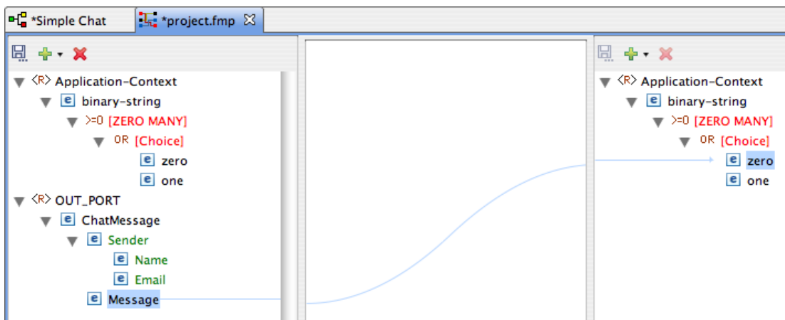
Figure 5.10.3: Mapper editor
