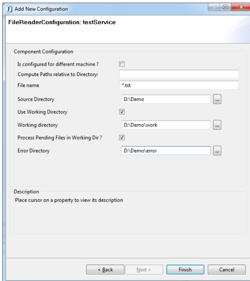
Figure 20: FileReader Configuration
