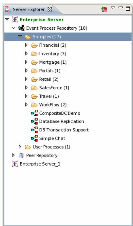
Figure 3.1.3: Server Explorer
