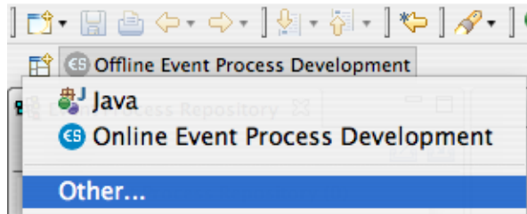
Figure 1.2.1: Perspective switch
