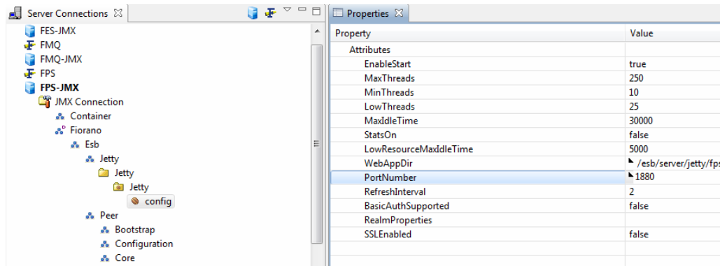
Figure 19: MBean attributes/properties
