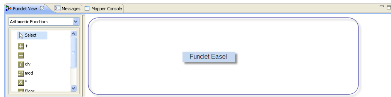
Figure 10.4 Funclet View
