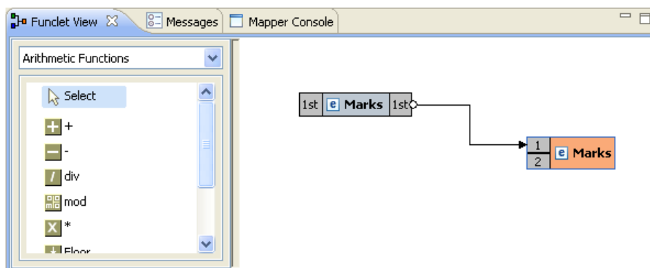
Figure 10.2.4: Funclet View
