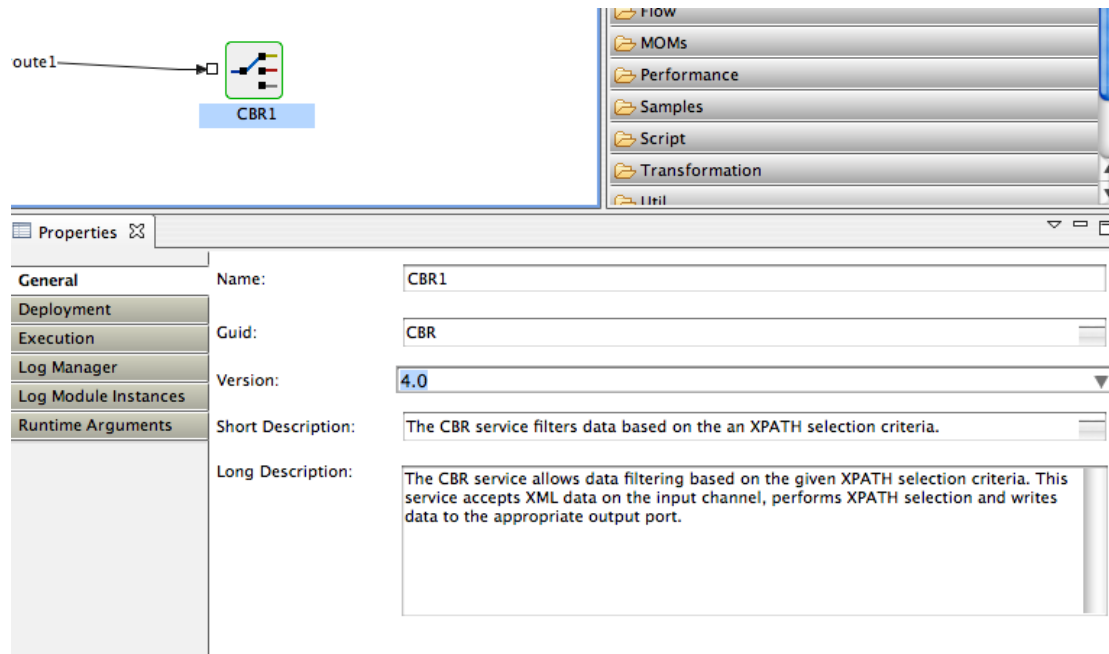
Figure 5.4.1: Component properties
