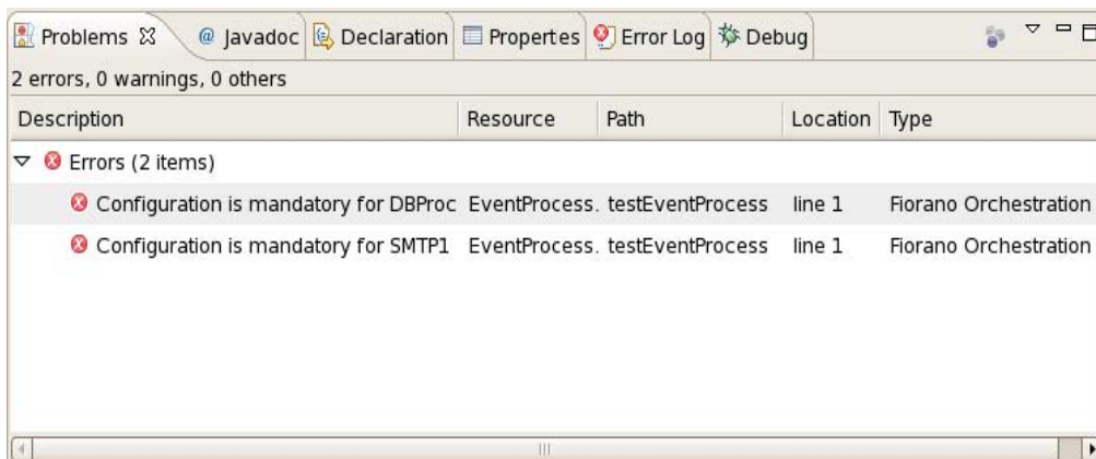
Figure 2.1.5: Problems view
