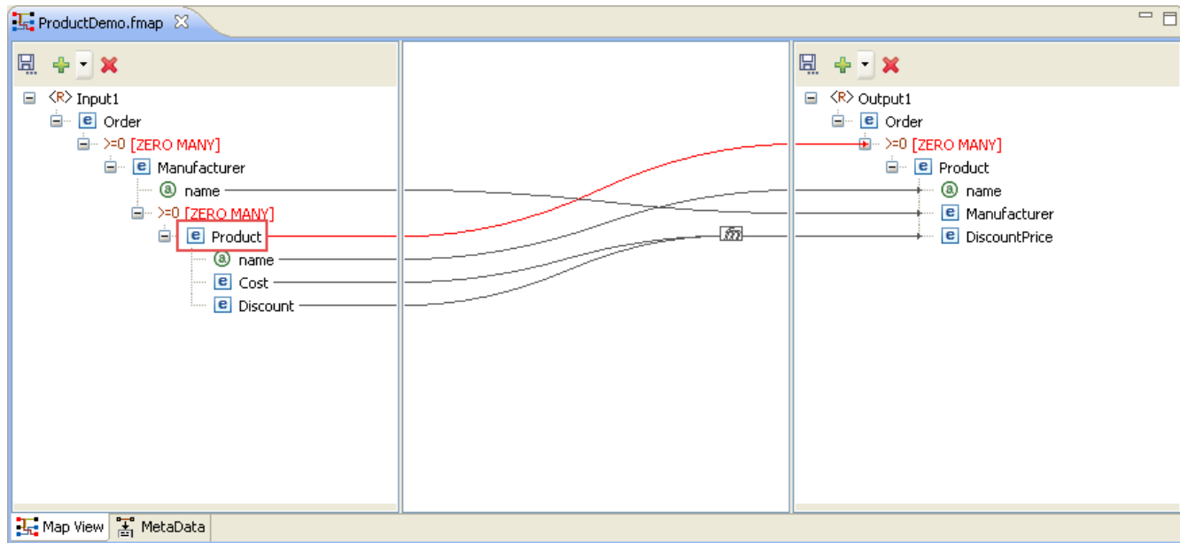
Figure 10.5.7: For-Each Mapping
