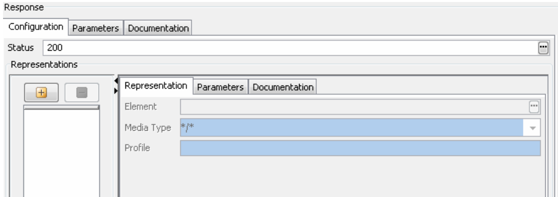
Figure 10: Response configuration
