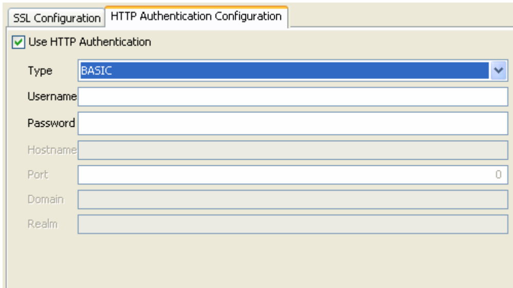
Figure 20: HTTP Authentication
