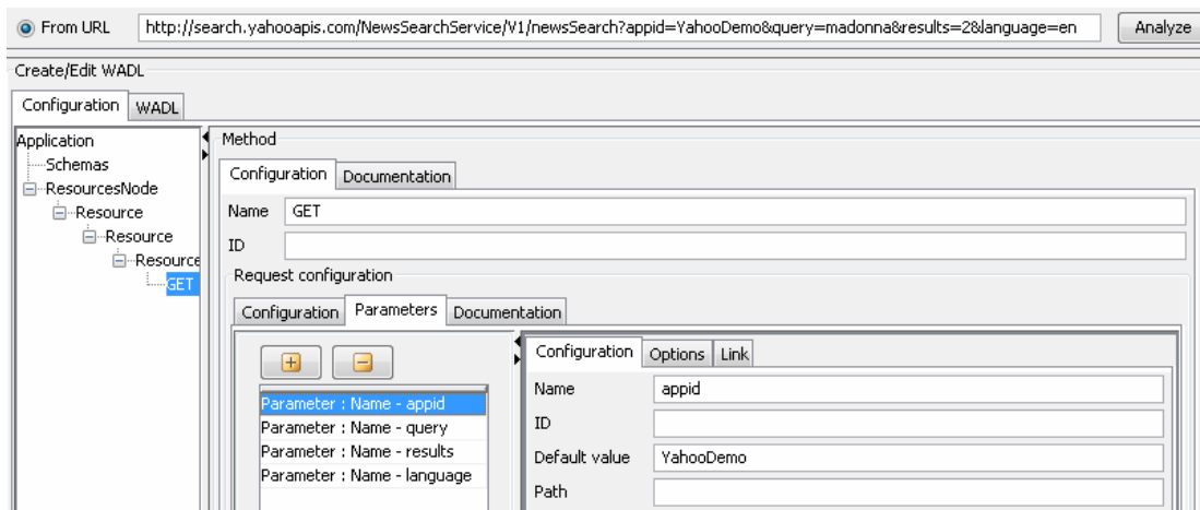
Figure 4: Analyzing URL
