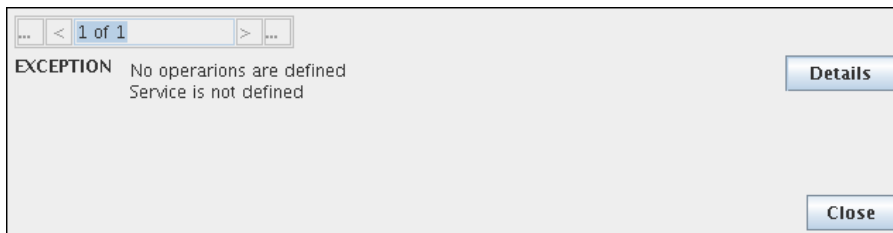
Figure 4.514: Errors Panel
