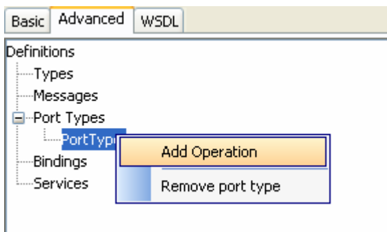
Figure 4.499: Adding Operation
