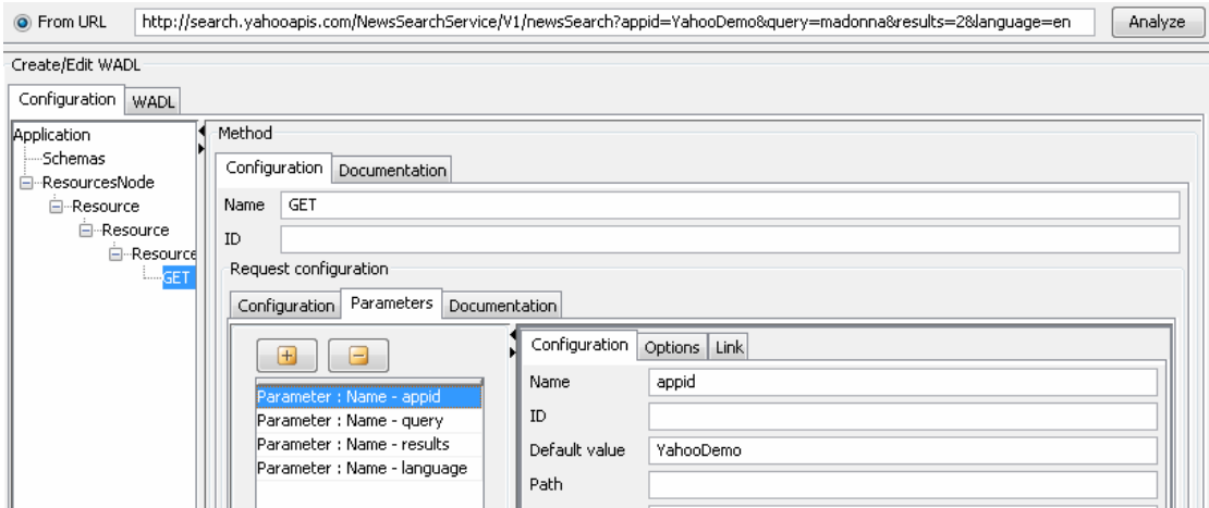
Figure 4: Analyzing URL
