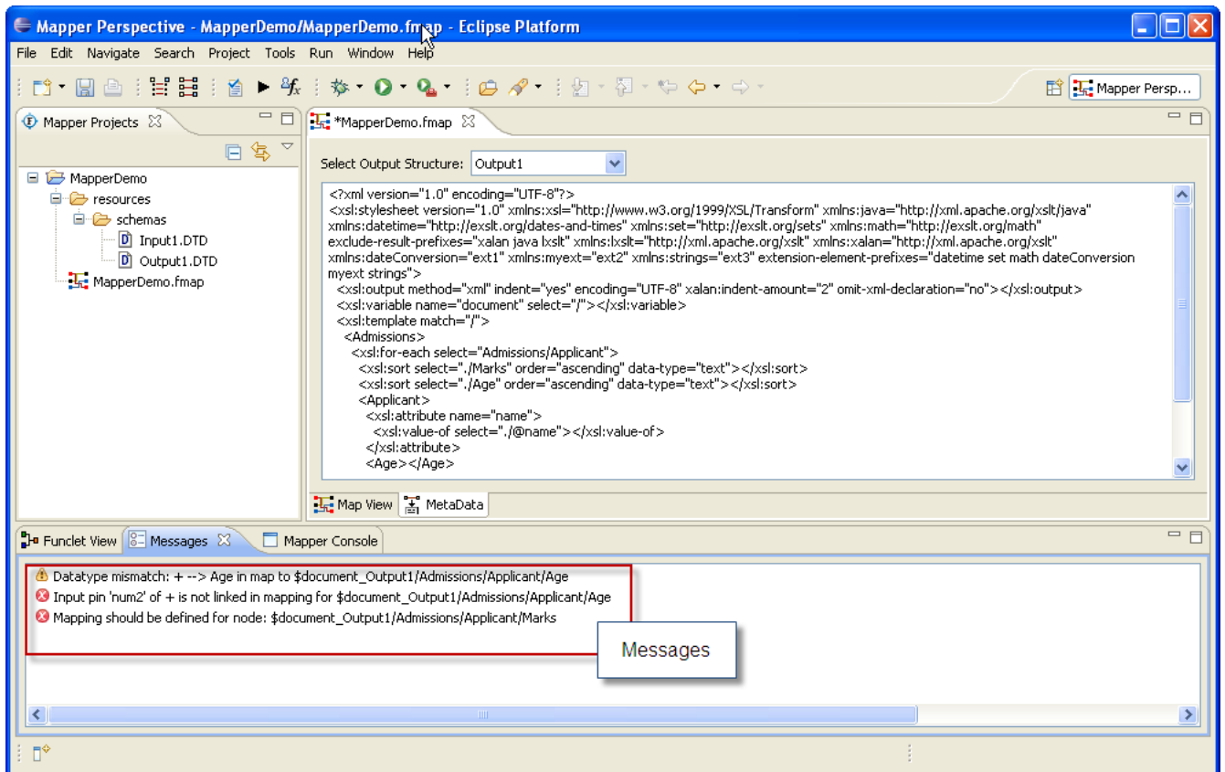
Figure 10.2.5: Meta Data and MetaData Messages view
