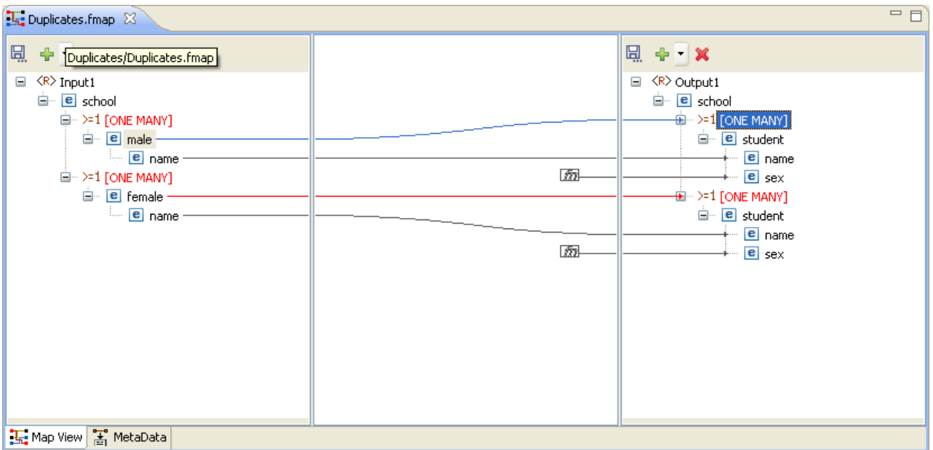
Figure 10.5.8: Mapping a node to One Many control node
