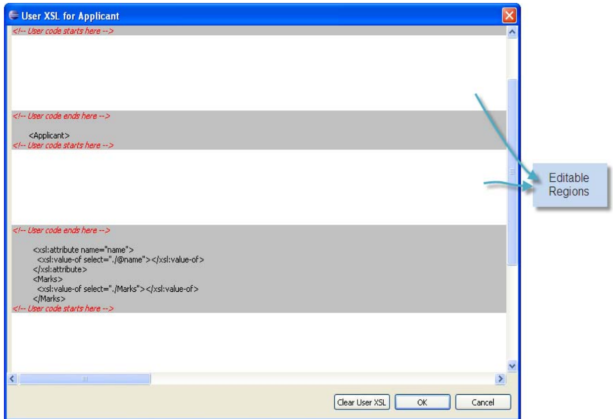
Figure 10.6.2: Editing the user xsl
