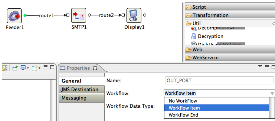
Figure 5.7.1: Enabling Document Tracking
