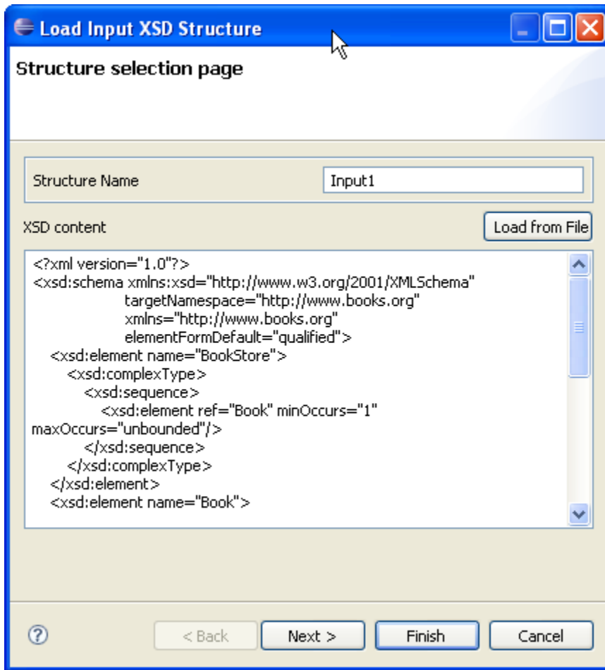
Figure 10.3.1: Structure Selection Page
