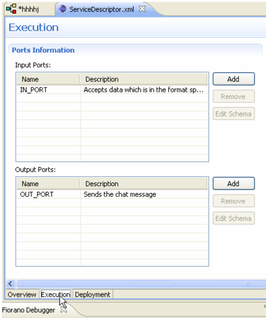
Figure 8.1.3: Sections under Service Descriptor
