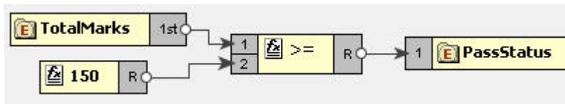
Figure 10.4.13: Linking the \geq and PassStatus nodes
