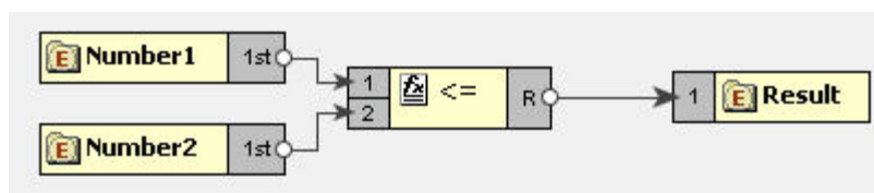
Figure 10.4.18: Linking outputs of the Number1 and Number2 nodes
