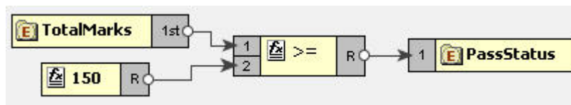
Figure 10.4.13: Linking the >= and PassStatus nodes
