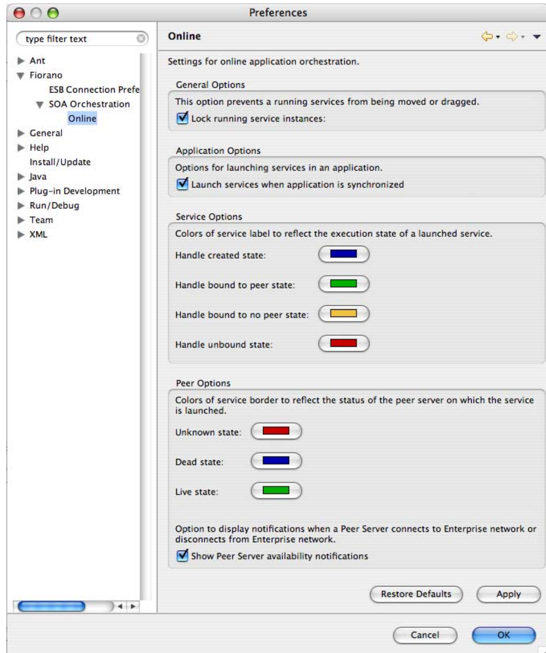
Figure 12.3.1: Online Orchestration preferences
