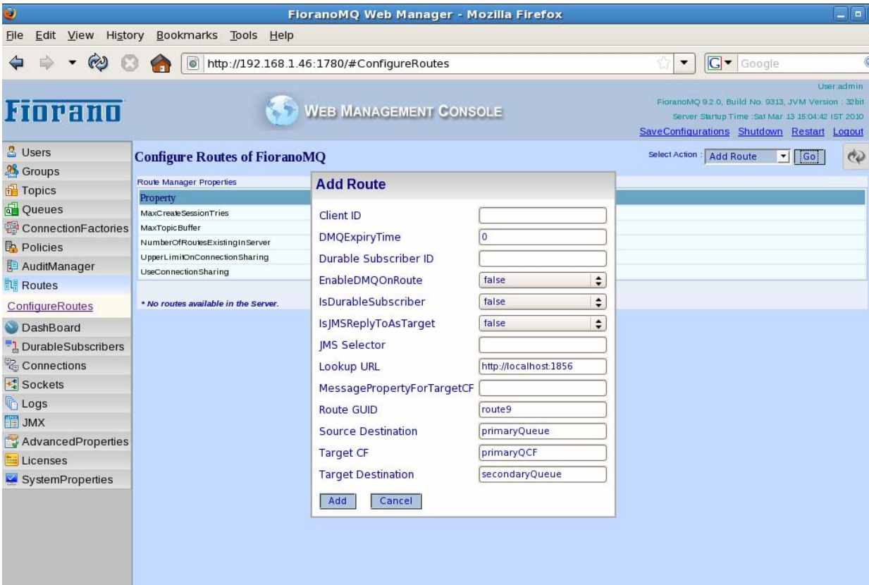
Figure 30.15: Adding Route
