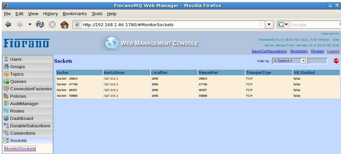
Figure 30.29: Monitor Sockets
