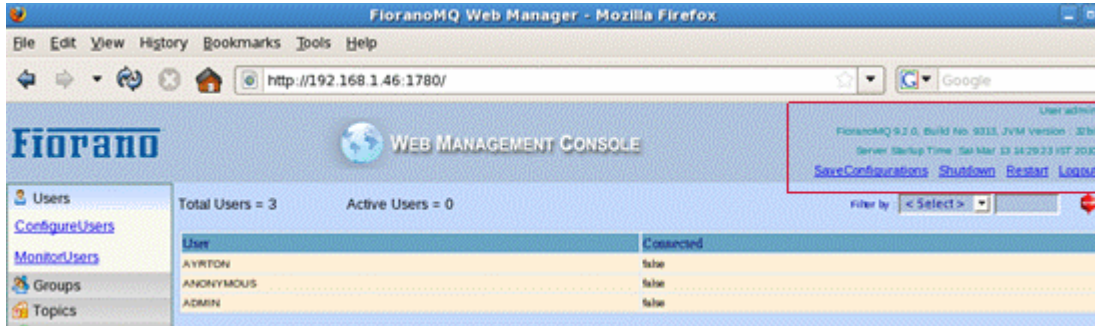
Figure 30.32: Status information
