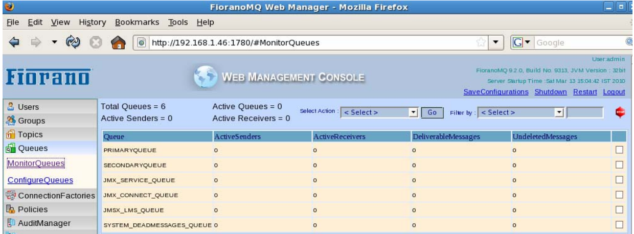
Figure 30.12: MonitorQueues View
