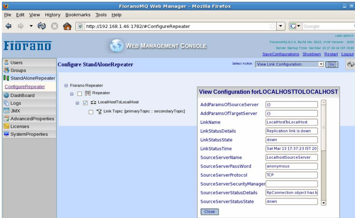
Figure 30.28: View Link Configuration
