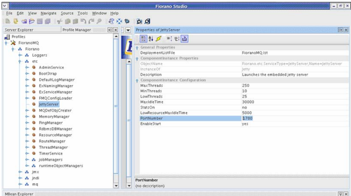
Figure 30.1: Properties of JettyServer Pane
