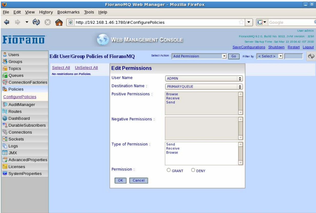
Figure 30.13: Editing policies of a destination
