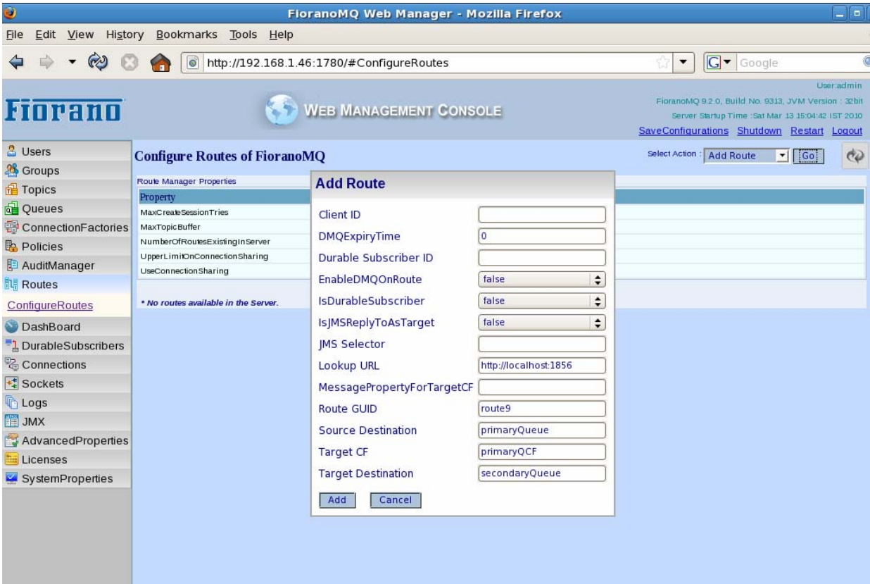
Figure 30.16: Route Added
