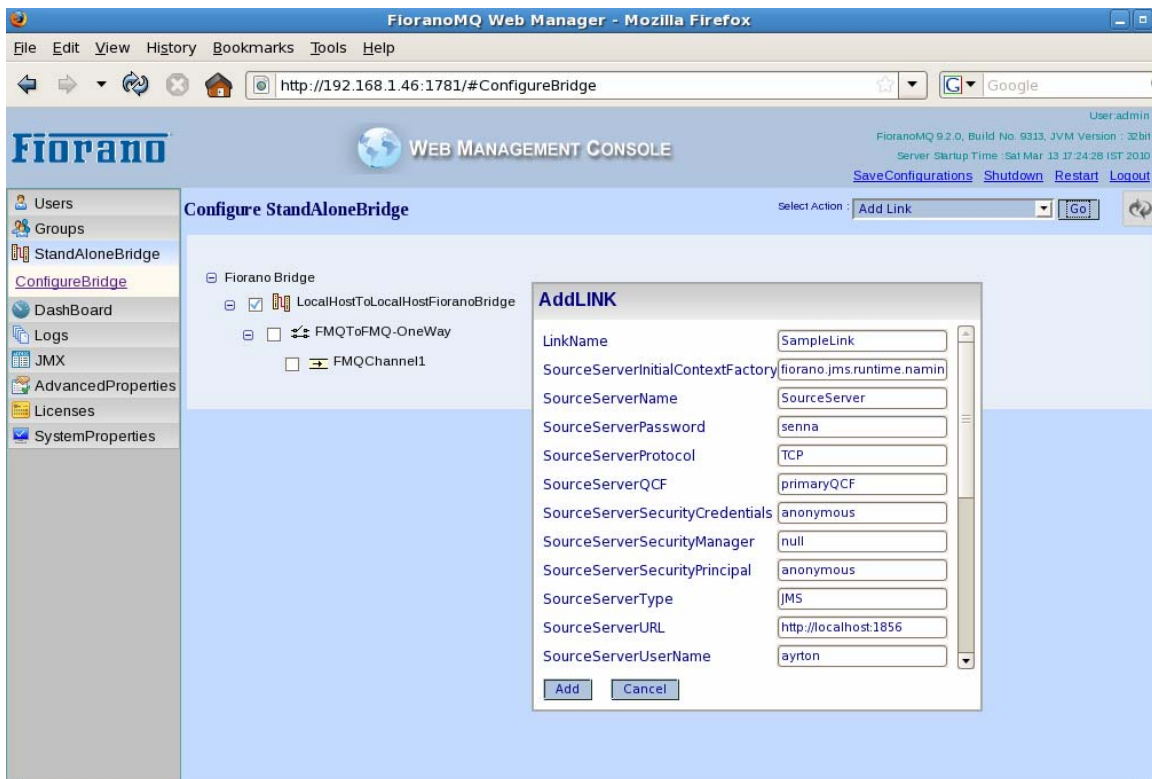
Figure 30.26: AddLink
