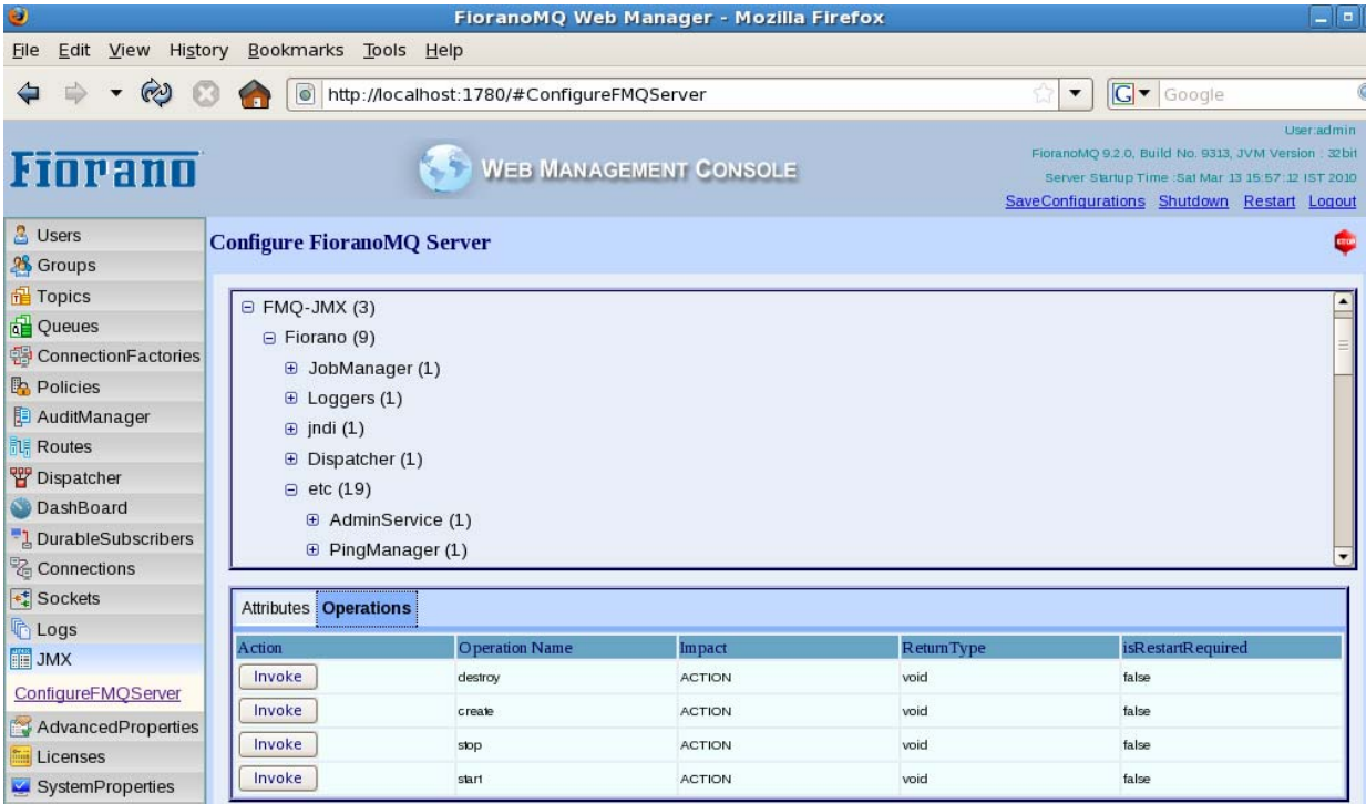
Figure 30.22: Operations View of JMX
