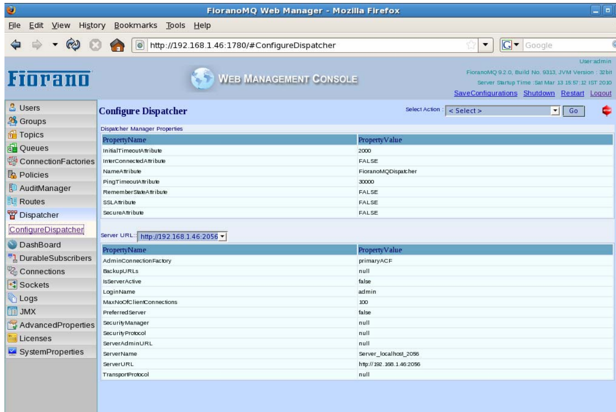
Figure 30.17: Dispatcher
