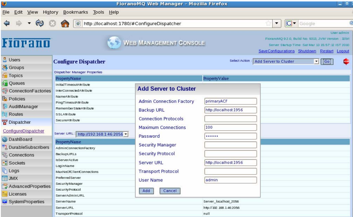
Figure 30.18: AddDispatcher Server
