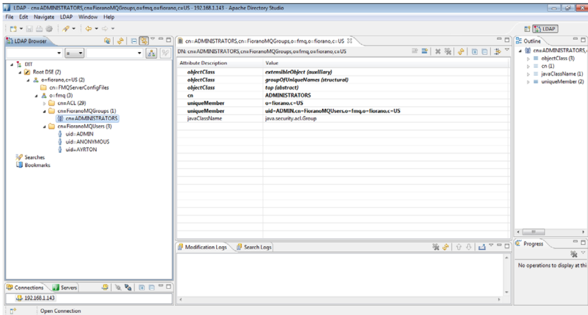
Figure – LDAP_Browser 1
