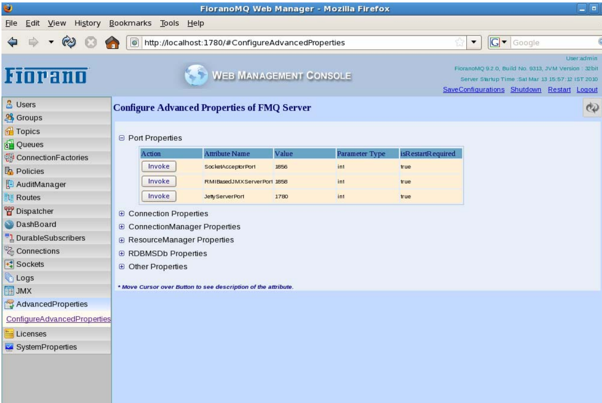
Figure 30.23: AdvancedProperties View
