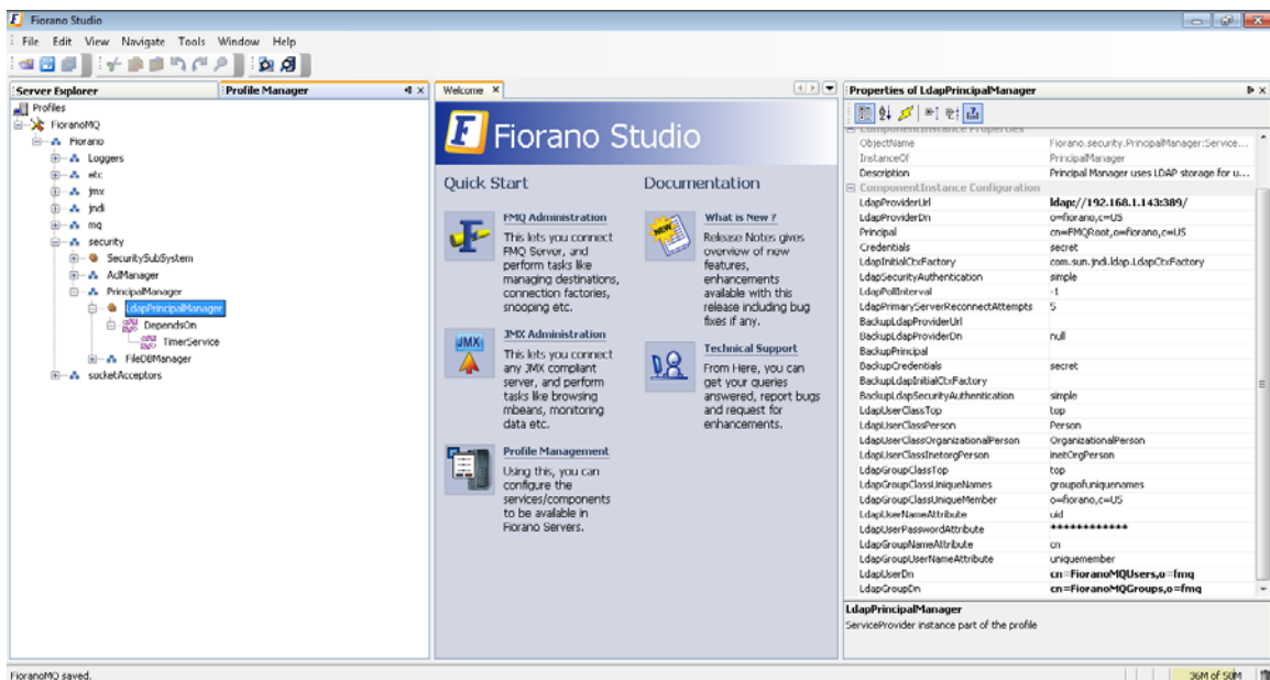
Figure – LDAP_Conf 1
