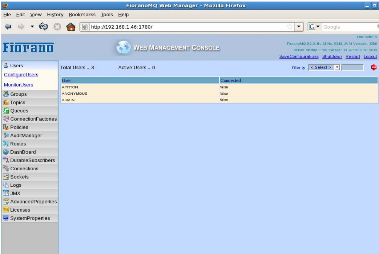
Figure 30.3: MonitorUsers View
