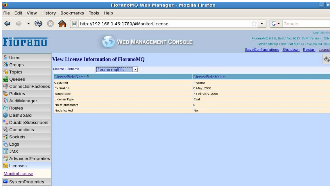
Figure 30.30: Licenses
