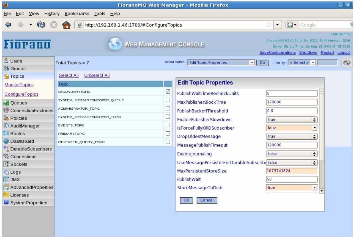
Figure 30.11: Editing Topic Properties
