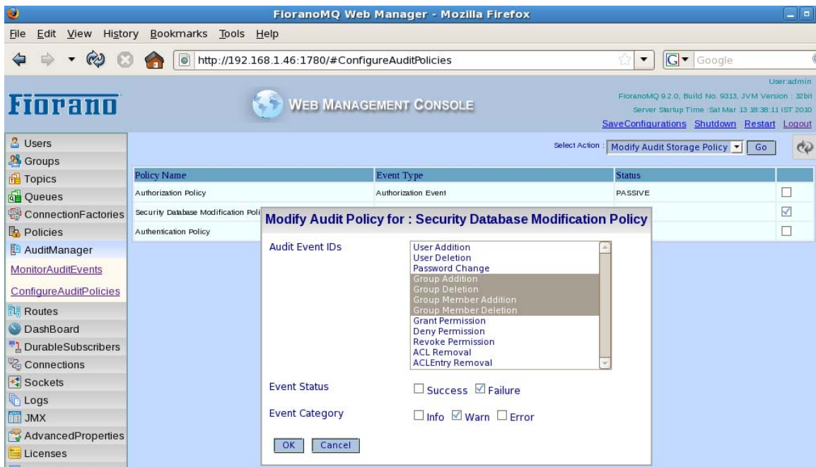
Figure 30.34: ConfigureAuditPolicies > Modify Audit Storage Policy
