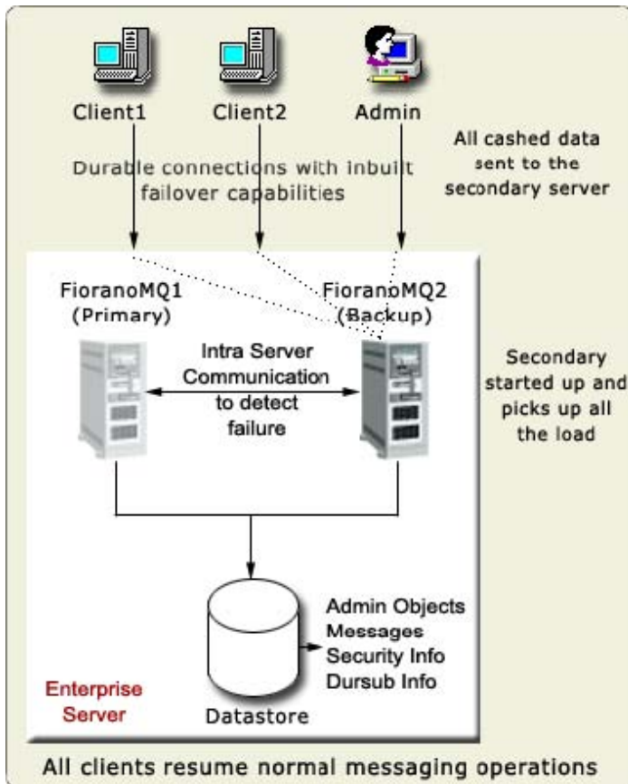
Figure 5: The Secondary Server Starts up Completely
