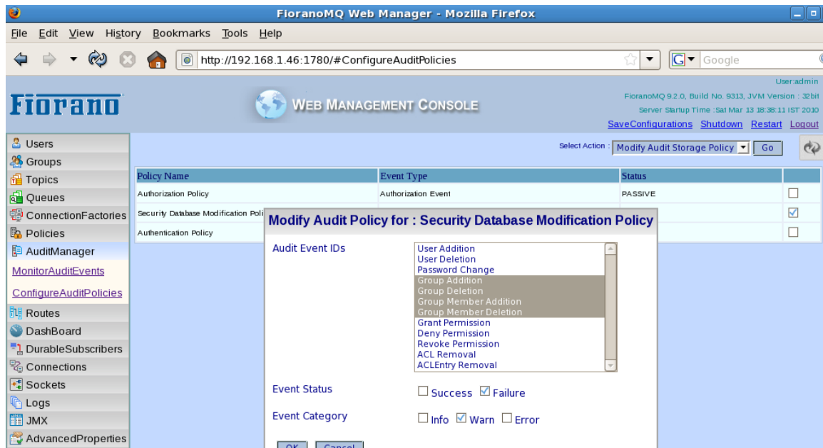
Figure 32.34: ConfigureAuditPolicies > Modify Audit Storage Policy
