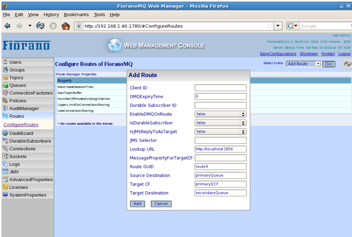
Figure 32.15: Adding Route
