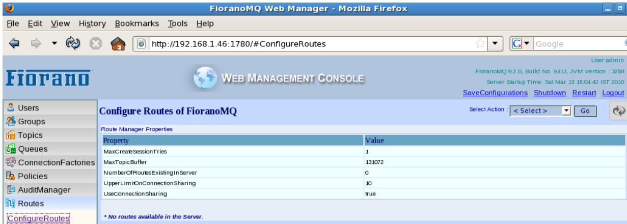
Figure 32.14: Route
