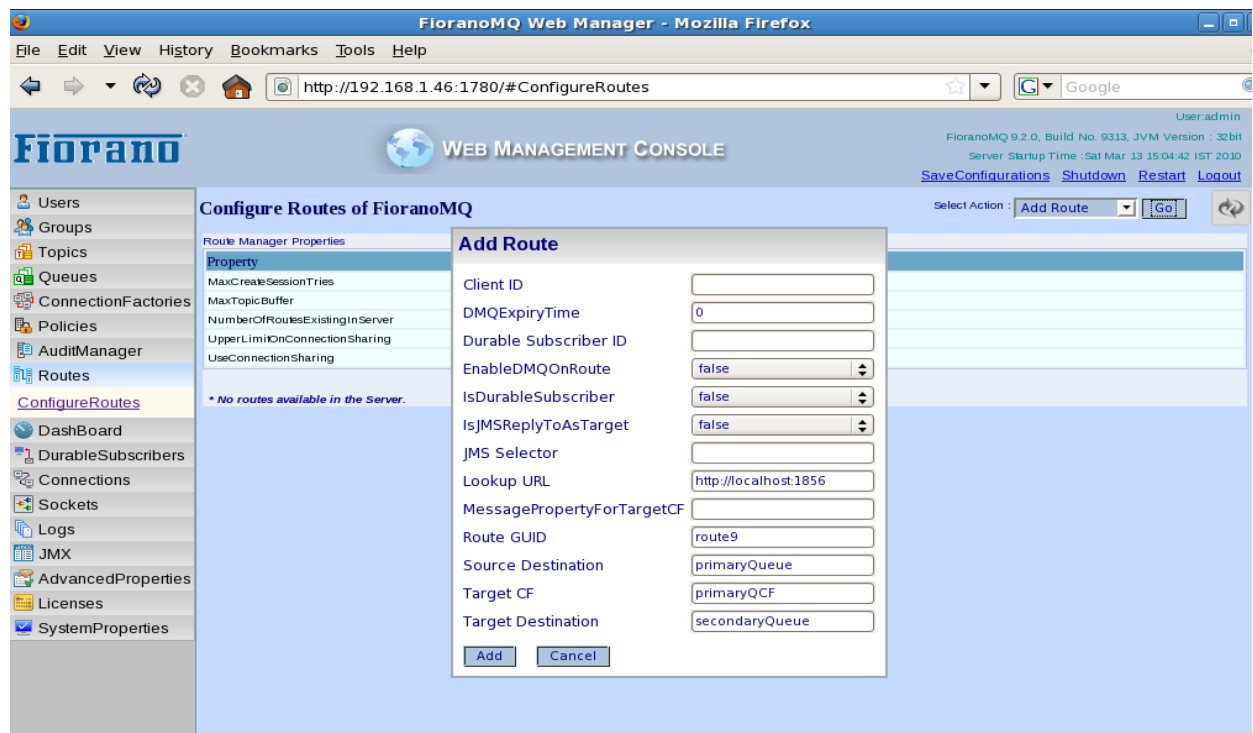
Figure: Adding Route
