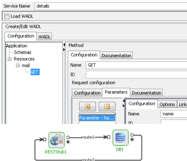
Figure 28: RESTStub being used to expose a database
