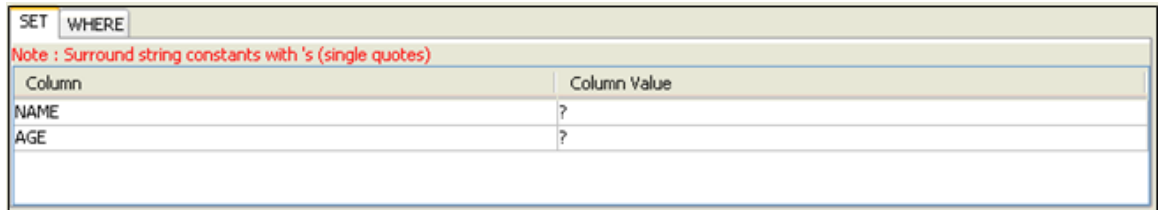
Figure 4.123: Columns added to SET clause
