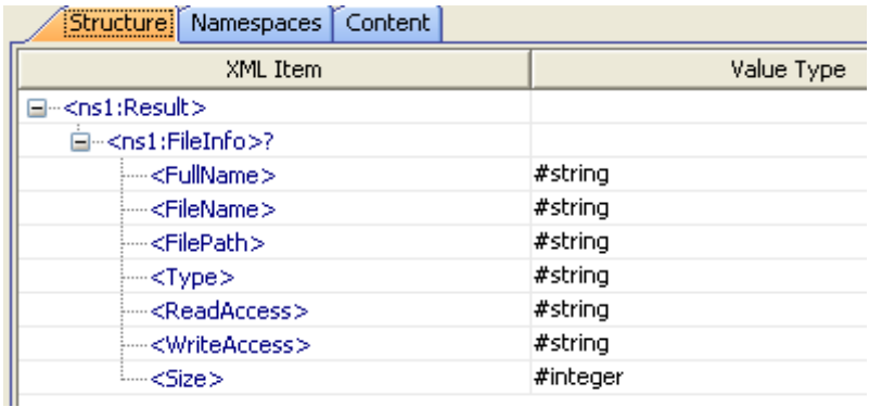
Figure 9: Schema on the output port
