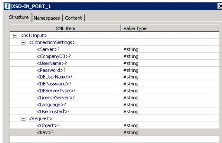
Figure 8: Input Schema for Select/Delete operation when Use Connection Details from input is set to "yes".
