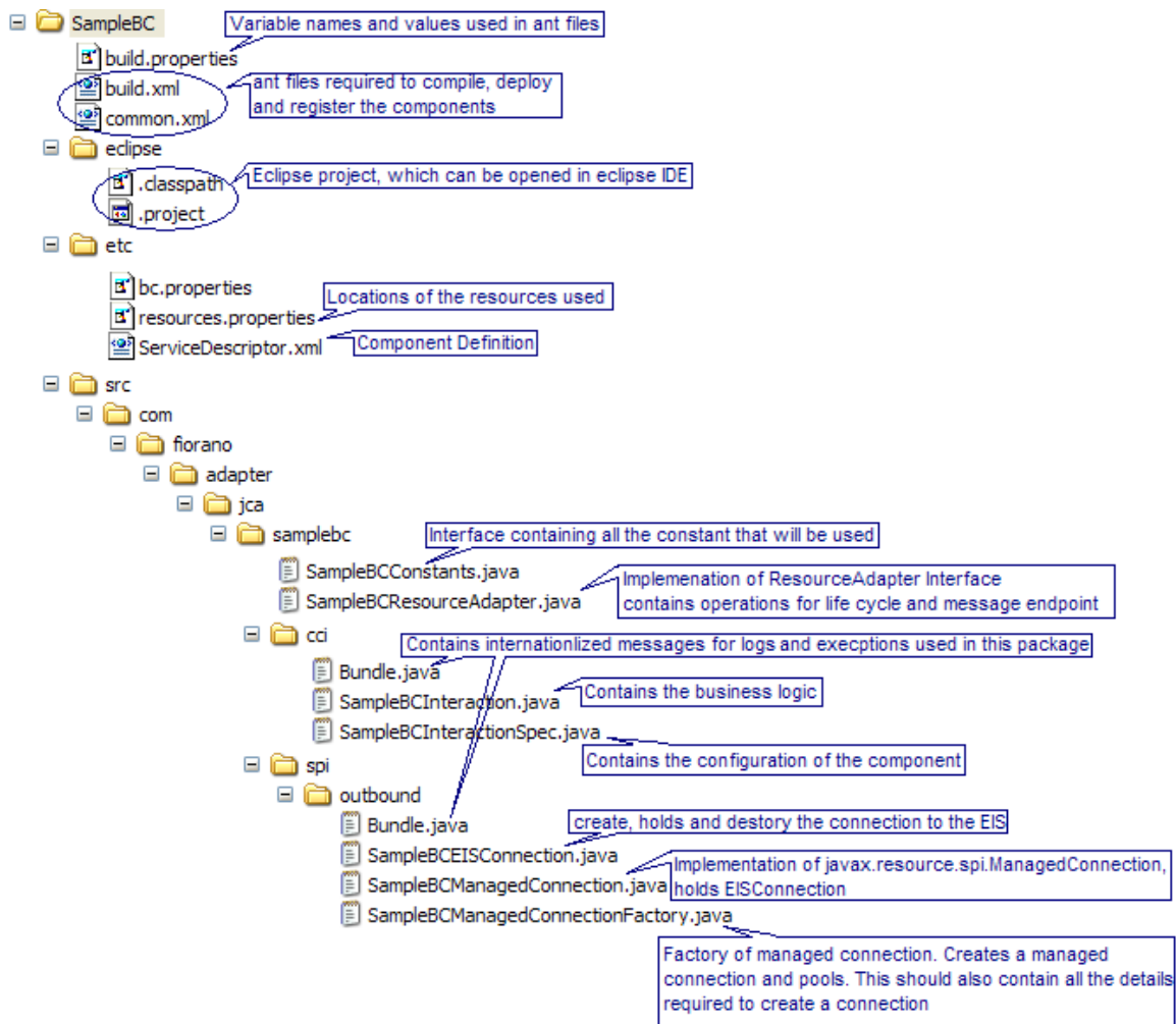
Figure 3.6.60: Structure of synchronous component
