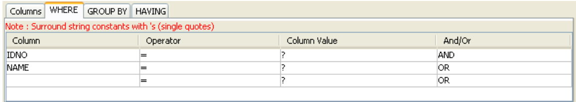
Figure 4.150: Specifying multiple conditions for WHERE clause
